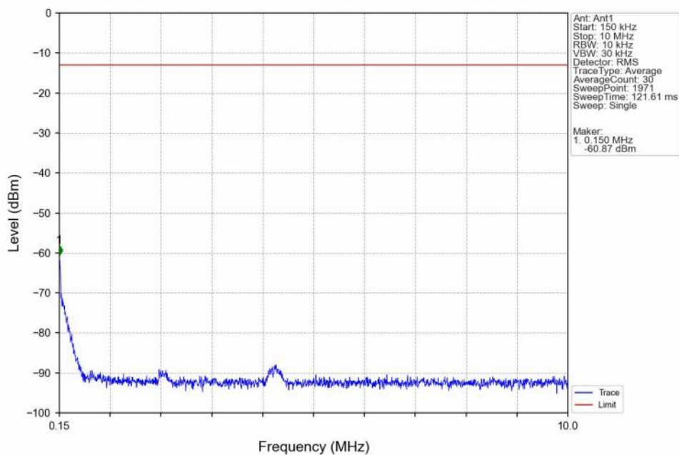
Band2_5MHz_16QAM_MCH_1880MHz_RB_1_0_NTNV
