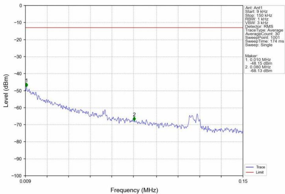
Band2_15MHz_16QAM_HCH_1902.5MHz_RB_1_0_NTNV
