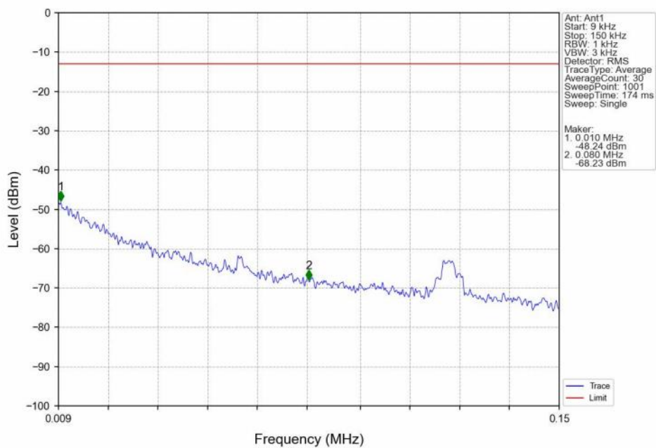
Band2_5MHz_16QAM_MCH_1880MHz_RB_1_0_NTNV
