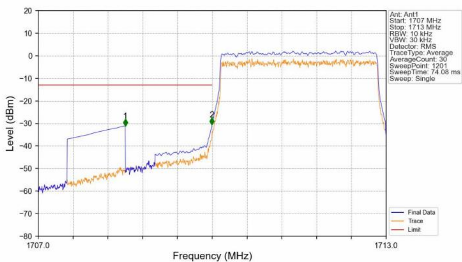
Band4_3MHz_16QAM_LCH_1711.5MHz_RB_15_0_NTNV
