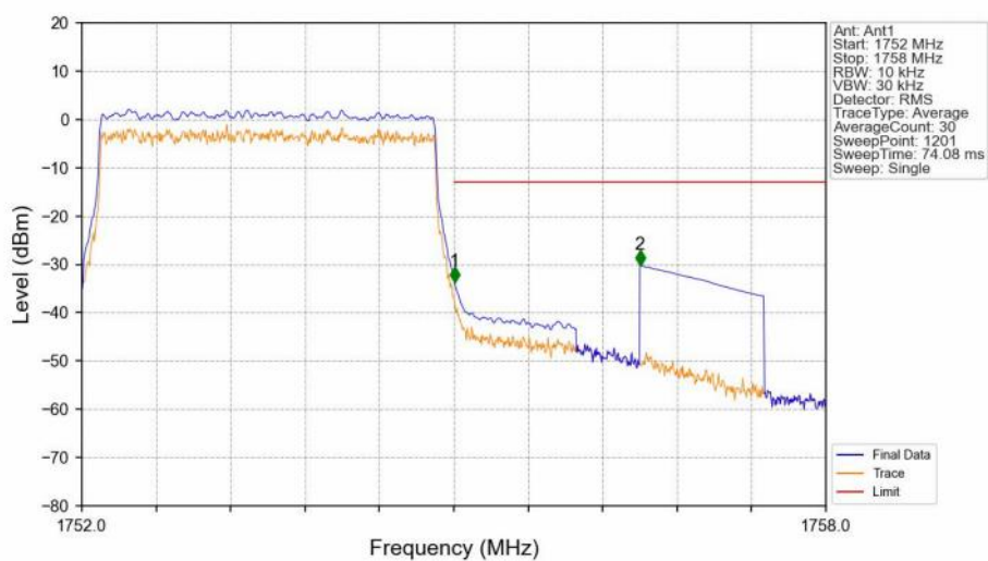
Band4_3MHz_16QAM_HCH_1753.5MHz_RB_15_0_NTNV
