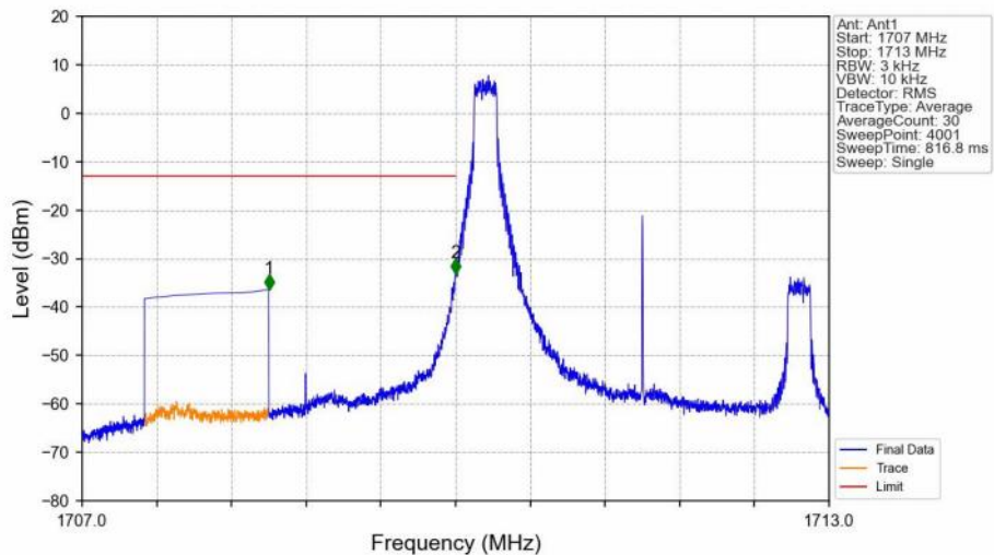
Band4_3MHz_QPSK_LCH_1711.5MHz_RB_1_0_NTNV
