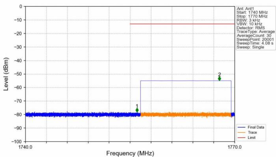
Band4_15MHz_16QAM_HCH_1747.5MHz_RB_1_74_NTNV
