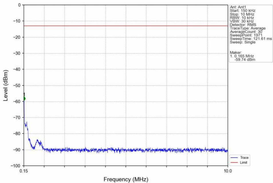
Band12_5MHz_QPSK_HCH_713.5MHz_RB_1_0_NTNV
