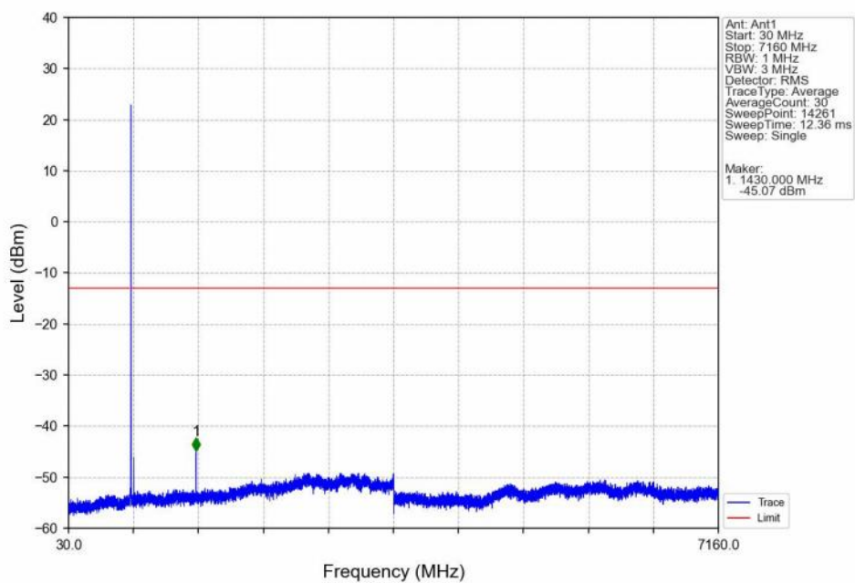
Band12_1.4MHz_QPSK_HCH_715.3MHz_RB_1_0_NTNV
