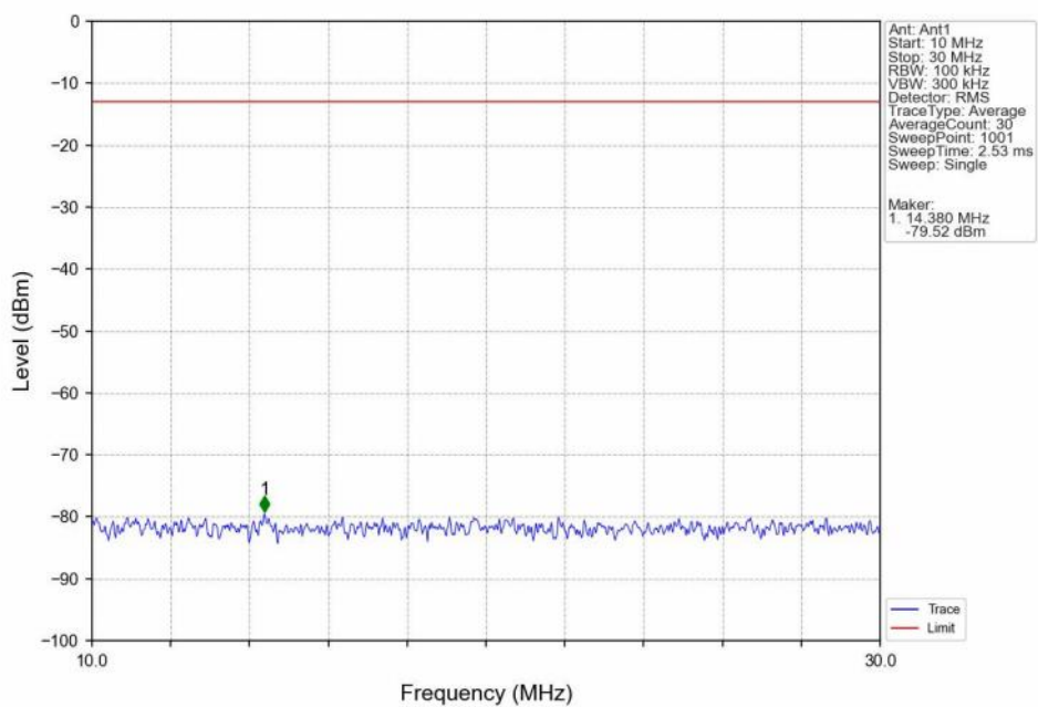
Band4_RMC_LCH_1712.4MHz_12.2kbps RMC_NTNV
