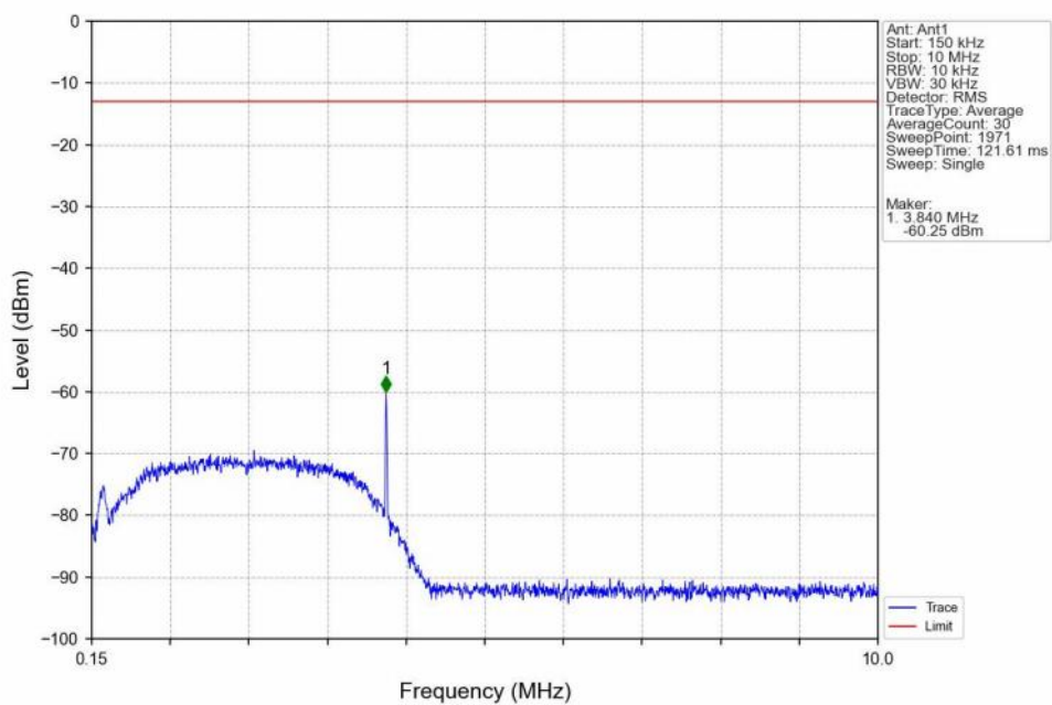
Band4_RMC_MCH_1732.6MHz_12.2kbps RMC_NTNV
