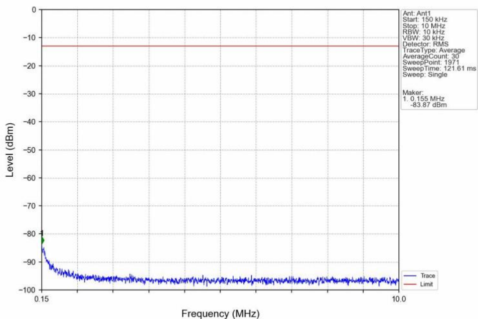
Band4_15MHz_QPSK_HCH_1747.5MHz_RB_1_0_NTNV
