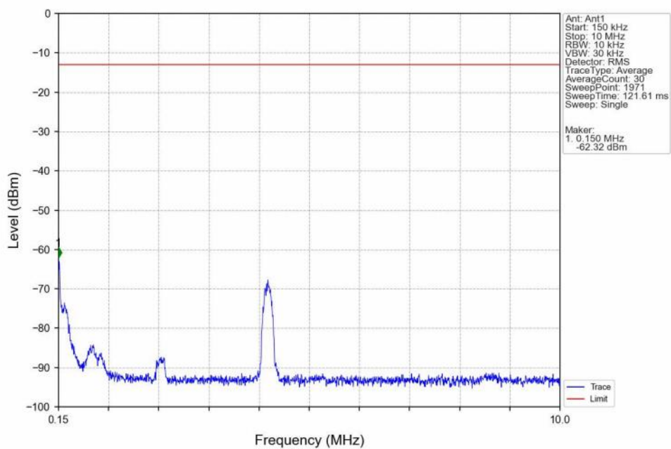
Band4_5MHz_16QAM_LCH_1712.5MHz_RB_1_0_NTNV
