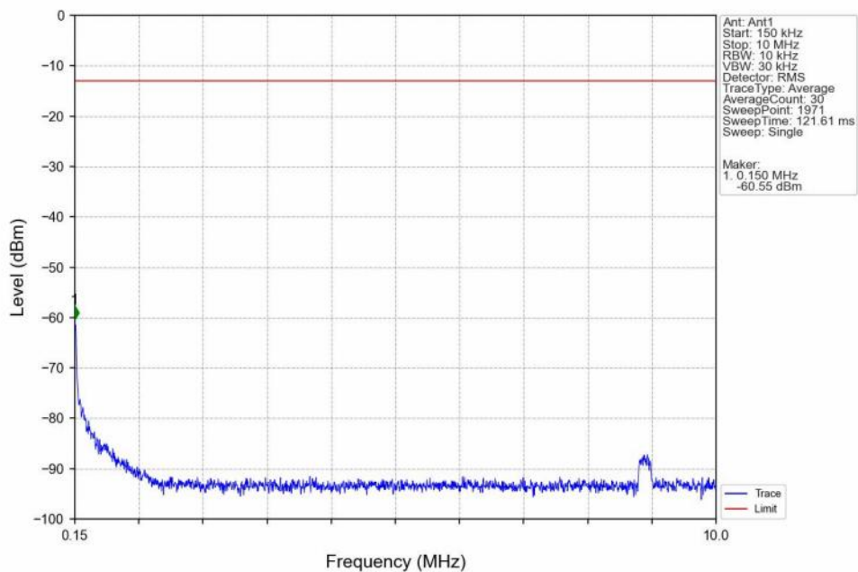
Band4_20MHz_16QAM_MCH_1732.5MHz_RB_1_0_NTNV
