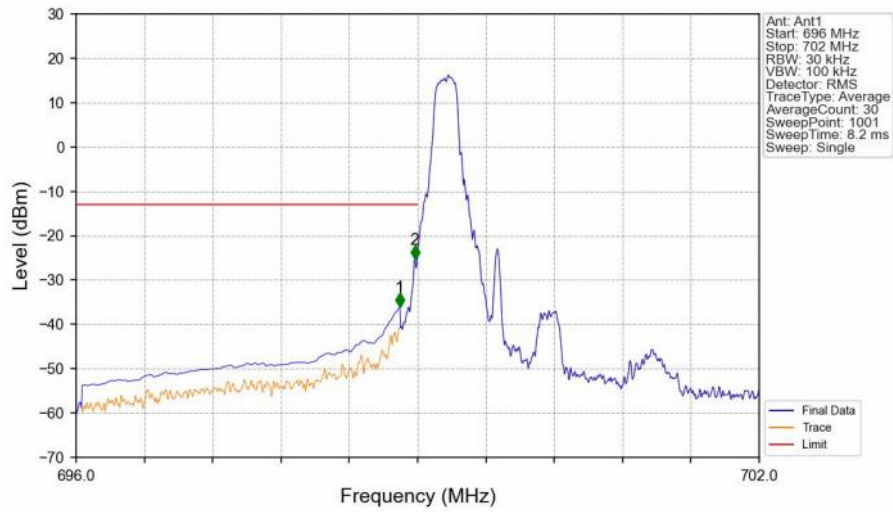
Band12_1.4MHz_16QAM_LCH_699.7MHz_RB_1_0_NTNV
