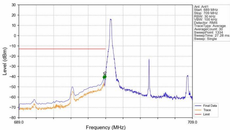
Band12_10MHz_16QAM_LCH_704MHz_RB_1_0_NTNV
