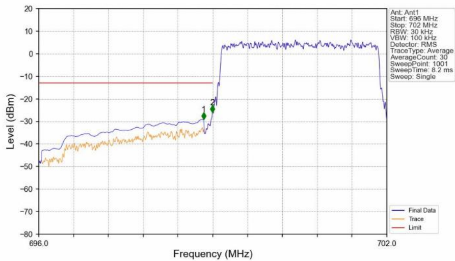
Band12_3MHz_QPSK_LCH_700.5MHz_RB_15_0_NTNV
