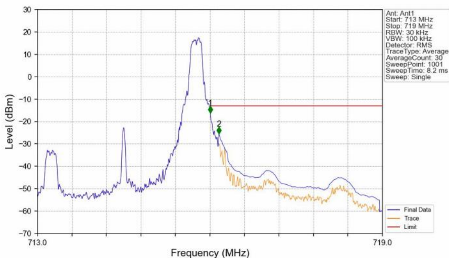
Band12_3MHz_16QAM_HCH_714.5MHz_RB_1_14_NTNV
