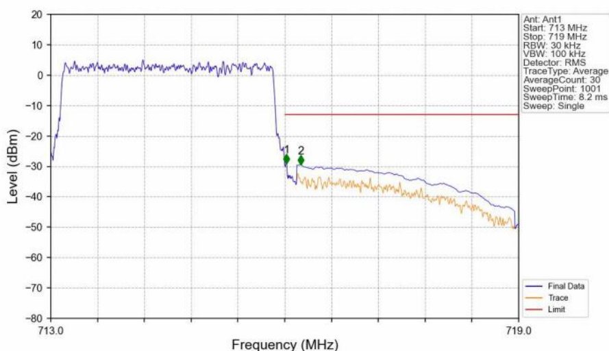
Band12_3MHz_16QAM_HCH_714.5MHz_RB_15_0_NTNV
