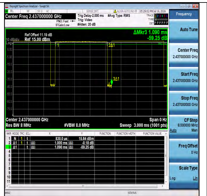
NTNV-11b-Ant1-2437
