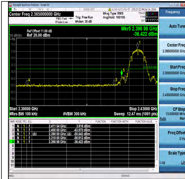
11b-Ant1-2412-PASS
