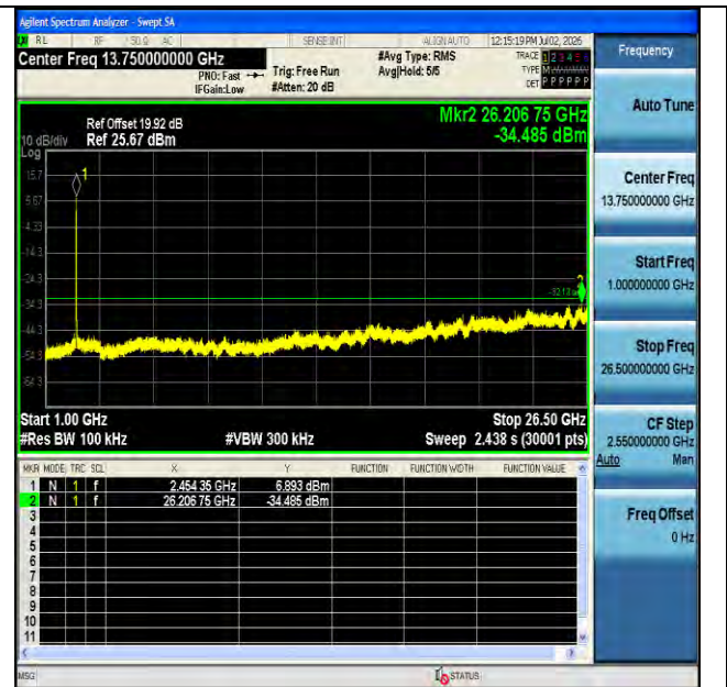
11g-Ant1-2462-1000~26500-PASS
