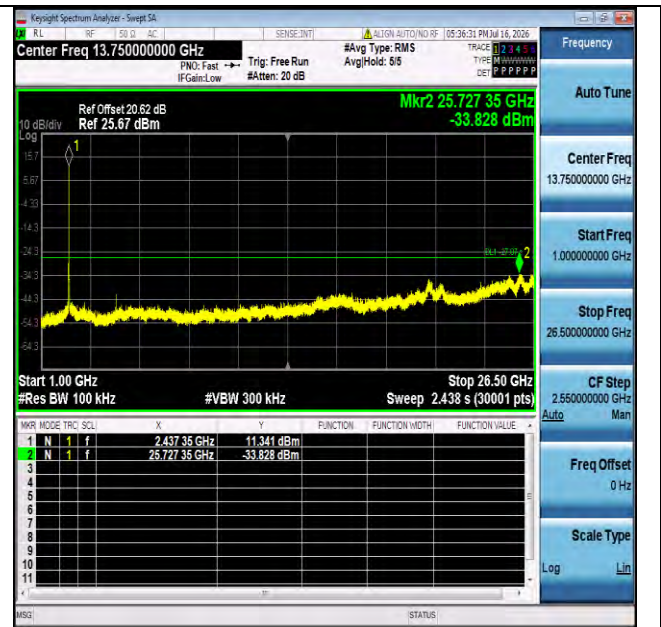
11b-Ant1-2437-1000~26500-PASS
