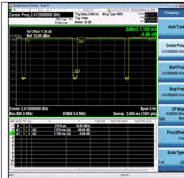
NTNV-11b-Ant1-2412
