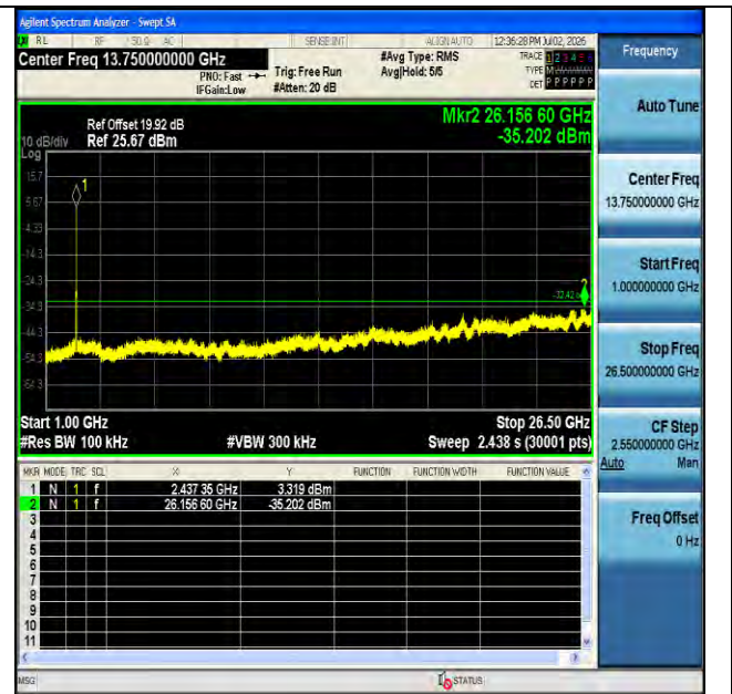
11n20SISO-Ant1-2437-1000~26500-PASS
