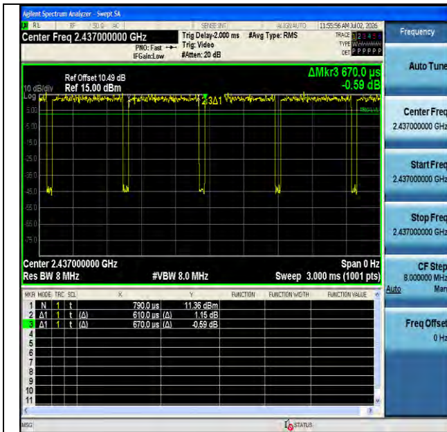
NTVN-11g-Ant1-2437
