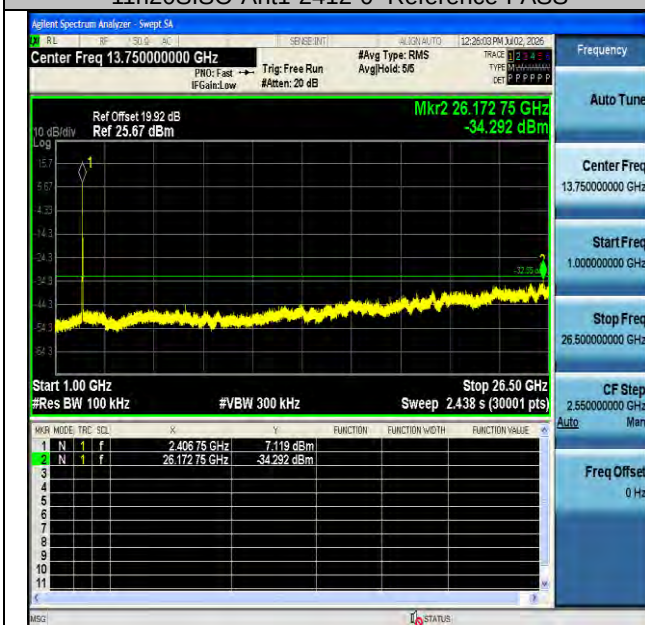
11n20SISO-Ant1-2412-1000~26500-PASS
