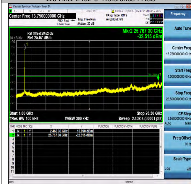
11b-Ant1-2462-1000~26500-PASS
