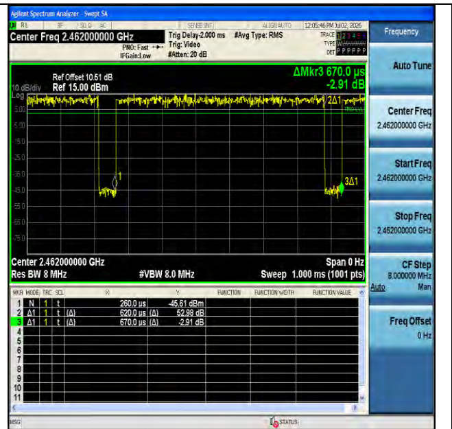
NTVN-11g-Ant1-2462
