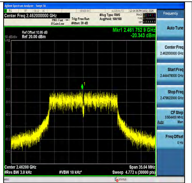
11g-Ant1-2462-PASS
