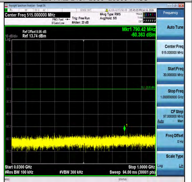
11b-Ant1-2462-30~1000-PASS
