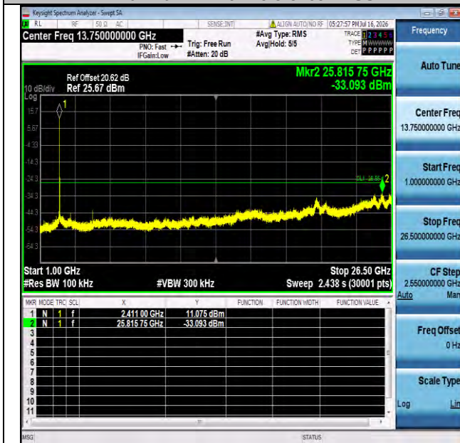
11b-Ant1-2412-1000~26500-PASS
