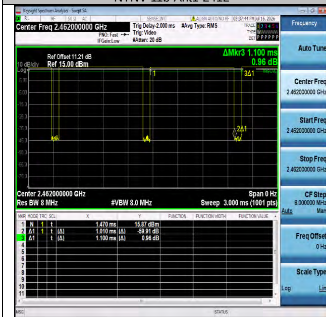
NTNV-11b-Ant1-2462
