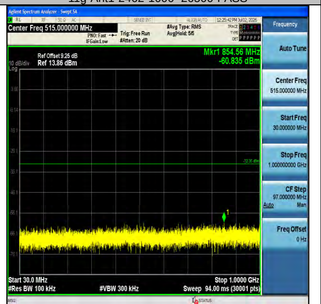
11n20SISO-Ant1-2412-30~1000-PASS
