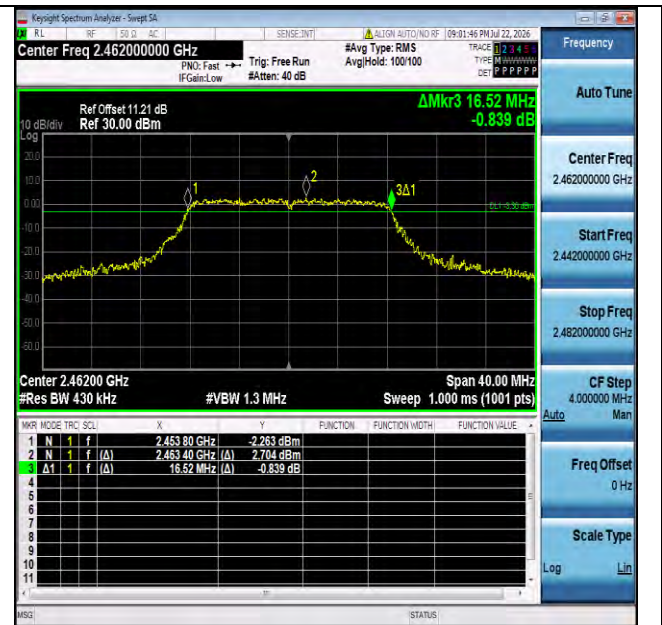
11g-Ant1-2462-PASS
