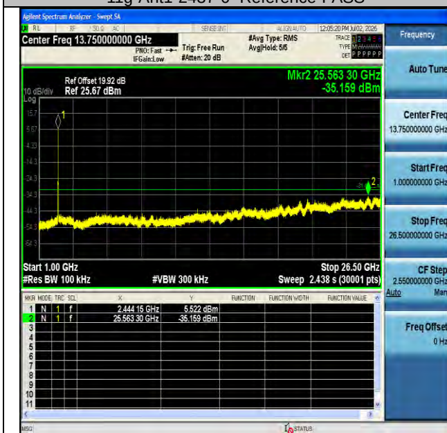
11g-Ant1-2437-1000~26500-PASS
