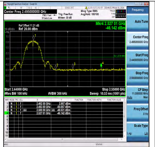
11b-Ant1-2462-PASS
