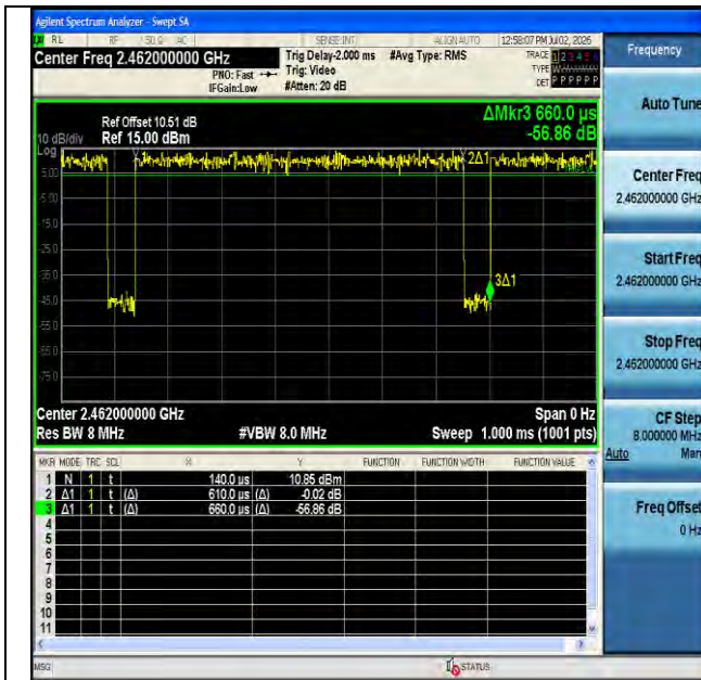
NTNV-11n20SISO-Ant1-2462
