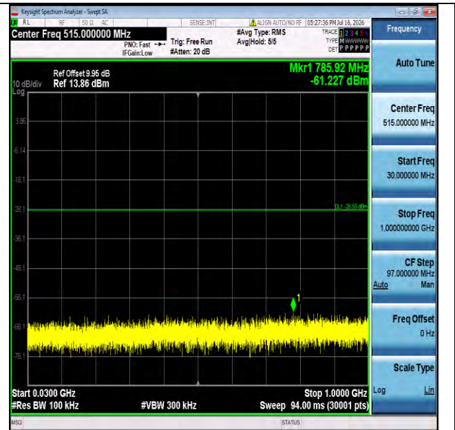
11b-Ant1-2412-30~1000-PASS
