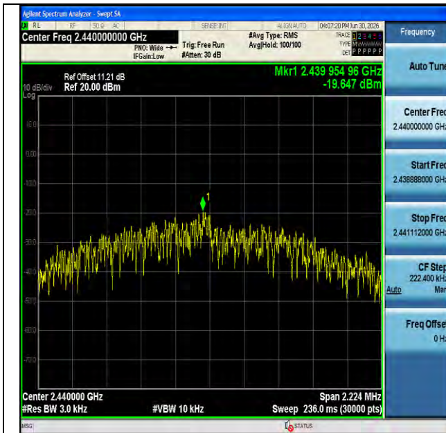
BLE_2M-Ant1-2440-PASS
