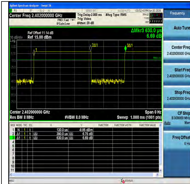
NTNV-BLE_1M-Ant1-2402
