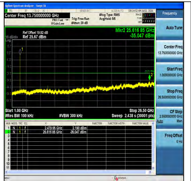
BLE_2M-Ant1-2480-1000~26500-PASS
