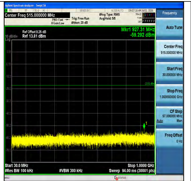
BLE_1M-Ant1-2402-30~1000-PASS
