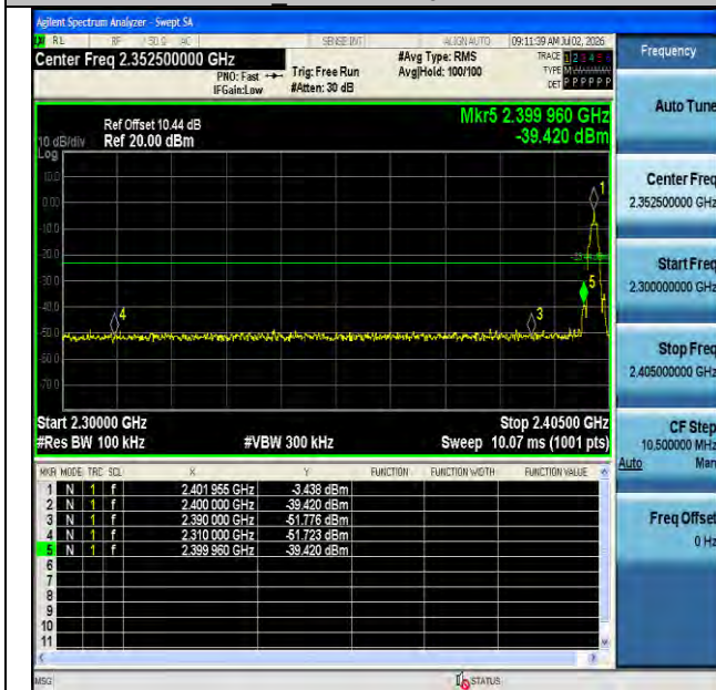
BLE_2M-Ant1-2402-PASS
