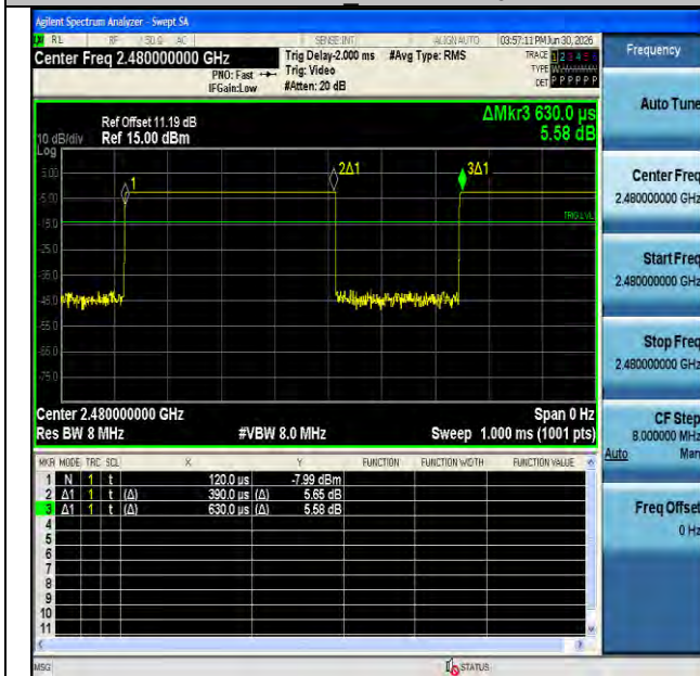
NTNV-BLE_1M-Ant1-2480
