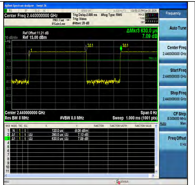
NTNV-BLE_1M-Ant1-2440
