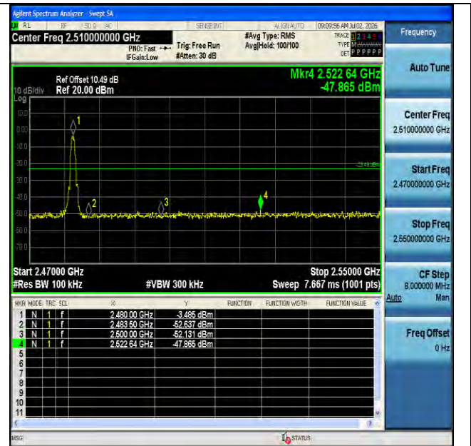
BLE_1M-Ant1-2480-PASS
