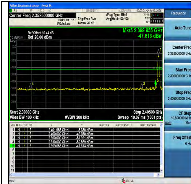
BLE_1M-Ant1-2402-PASS
