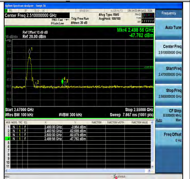
BLE_2M-Ant1-2480-PASS
