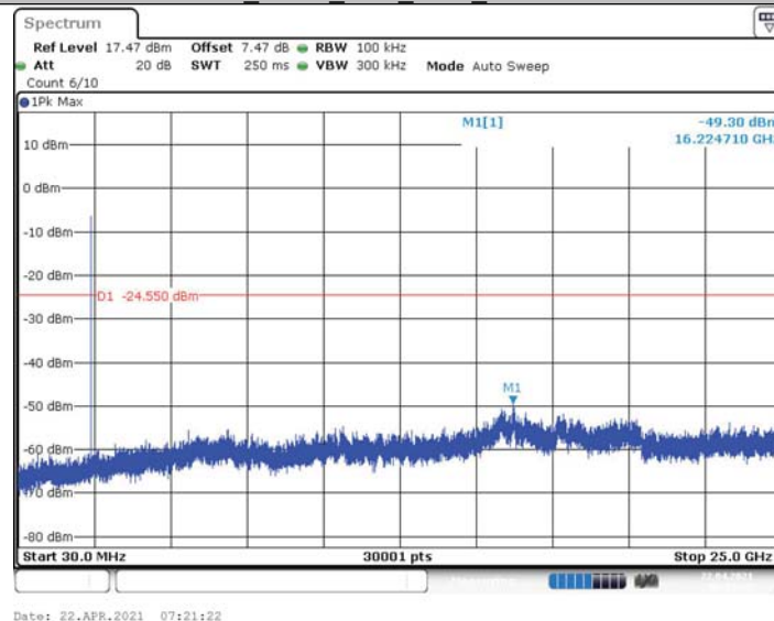
BLE_BT4.0_Ant1_2440_0~Reference
