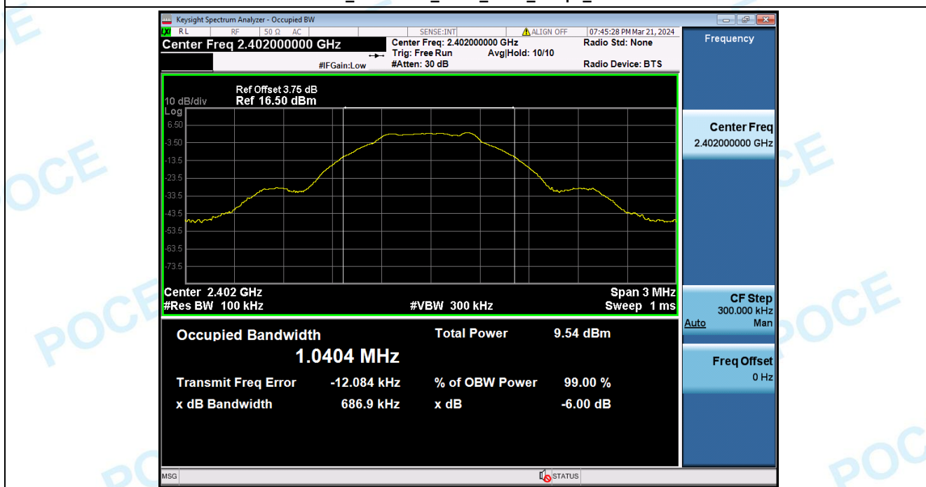
-6dB_Bandwidth_NVNT_ANT1_1Mbps_2402
