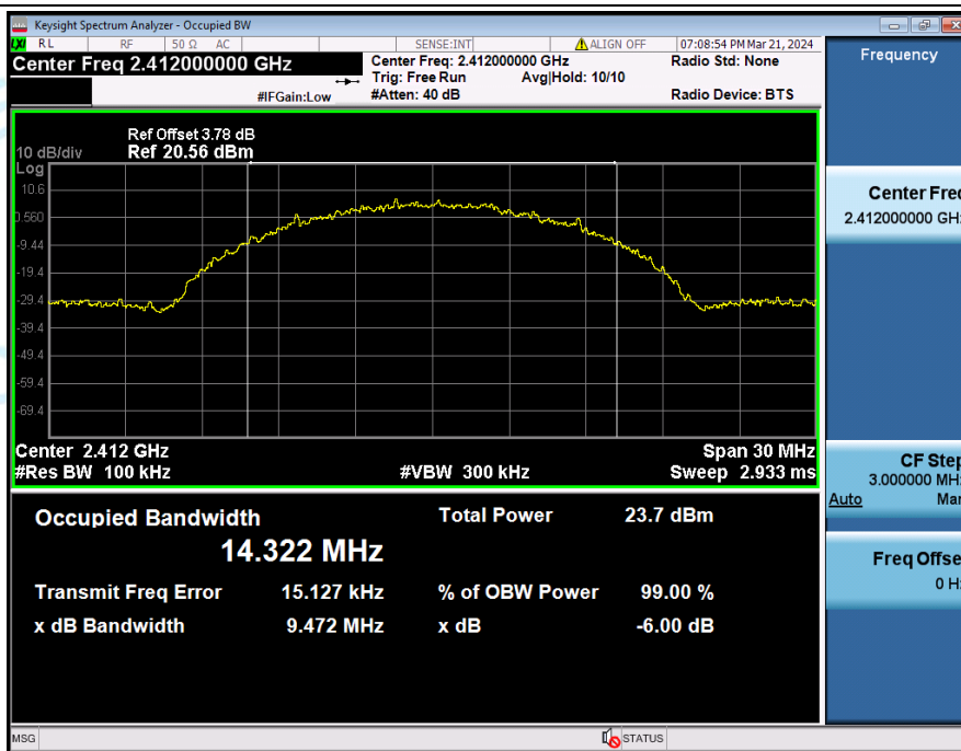
-6dB_Bandwidth_NVNT_ANT1_802_11b_2412
