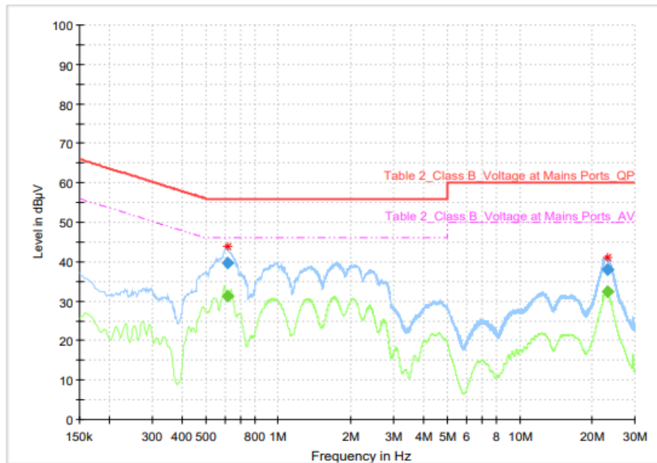
N-Line Conducted Emission
