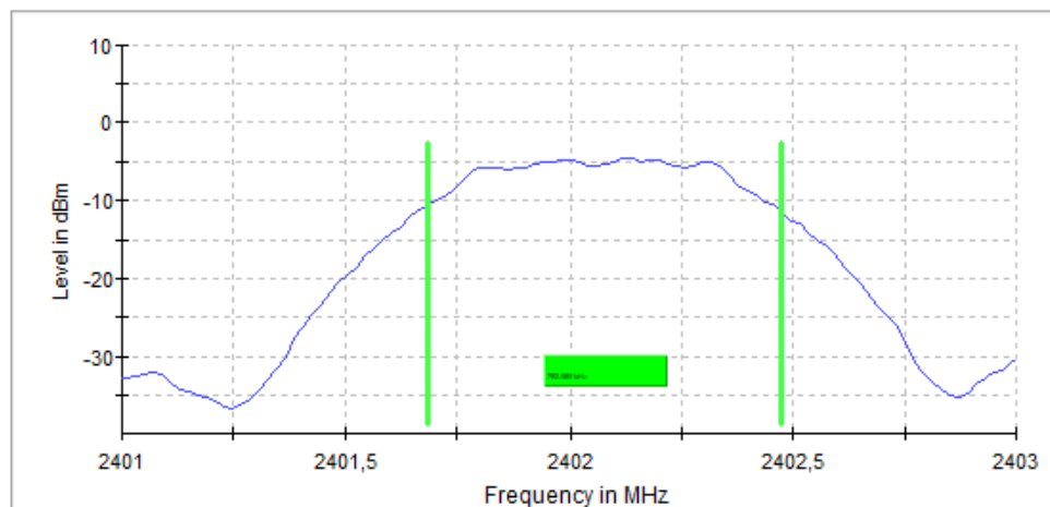
Channel 37 (2402 MHz)
