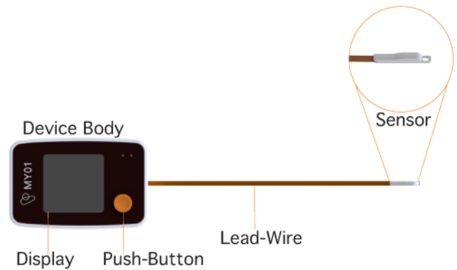
Figure 4 : Pressure Monitor (Applied Part)
