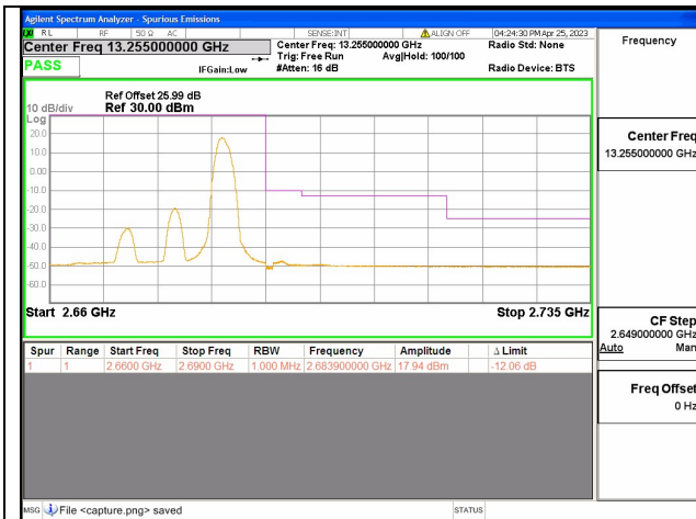
Band41C / 20+5MHz / High CH / QPSK / 1 RB
