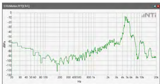
ANSI/TIA 5050-2018 \ 2N HAC OFF \ WB 23.85kbps\ 5.2 Receive path – distortion and noise\WCDMA Band V
