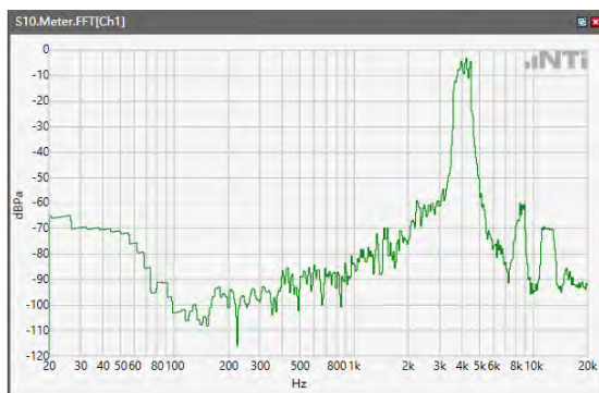
ANSI/TIA 5050-2018 \ 2N HAC OFF \ WB 23.85kbps\ 5.2 Receive path – distortion and noise\LTE Band 7
