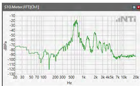
ANSI/TIA 5050-2018 \ 8N HAC OFF \ NB 12.2kbps\ 5.2 Receive path – distortion and noise\LTE Band 48
