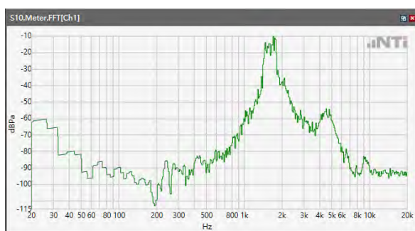
ANSI/TIA 5050-2018 \ 8N HAC OFF \ WB 23.85kbps\ 5.2 Receive path – distortion and noise\LTE Band 48
