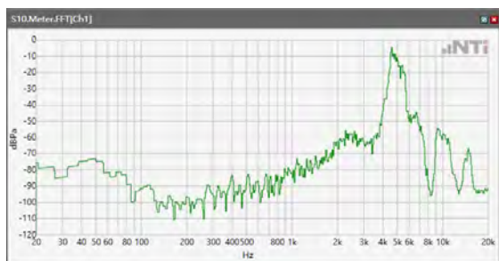
ANSI/TIA 5050-2018 \ 2N HAC OFF \ WB 23.85kbps\ 5.2 Receive path – distortion and noise\5GNR n41
