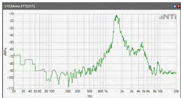
ANSI/TIA 5050-2018 \ 8N HAC OFF \ WB 23.85kbps\ 5.2 Receive path – distortion and noise\LTE Band 7
