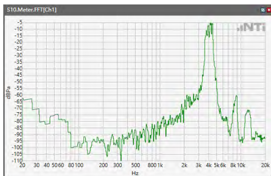
ANSI/TIA 5050-2018 \ 2N HAC OFF \ WB 23.85kbps\ 5.2 Receive path – distortion and noise\LTE Band 13
