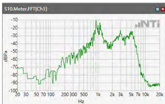
ANSI/TIA 5050-2018 \ 2N HAC OFF \ WB 23.85kbps\ 5.2 Receive path – distortion and noise\LTE Band 30
