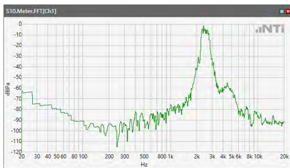
ANSI/TIA 5050-2018 \ 8N HAC OFF \ WB 23.85kbps\ 5.2 Receive path – distortion and noise\5GNR n26
