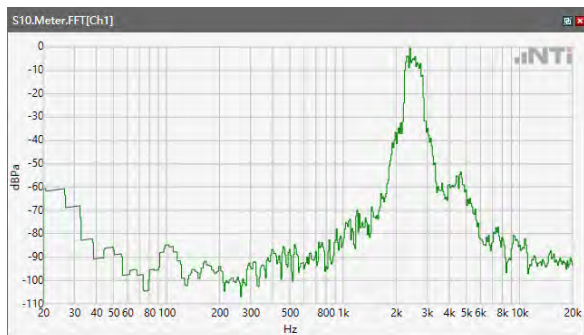
ANSI/TIA 5050-2018 \ 8N HAC OFF \ WB 23.85kbps\ 5.2 Receive path – distortion and noise\5GNR n71
