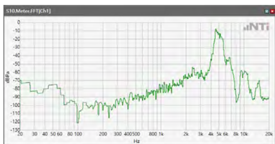
ANSI/TIA 5050-2018 \ 2N HAC OFF \ WB 23.85kbps\ 5.2 Receive path – distortion and noise\5GNR n66
