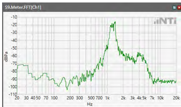
ANSI/TIA 5050-2018 \ 8N HAC OFF \ WB 23.85kbps\ 5.2 Receive path – distortion and noise\5GNR n71
