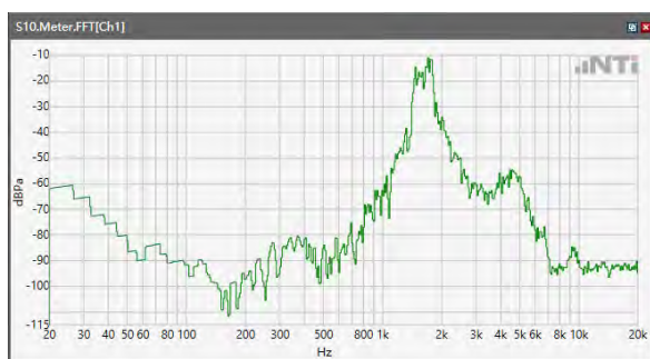
ANSI/TIA 5050-2018 \ 8N HAC OFF \ WB 23.85kbps\ 5.2 Receive path – distortion and noise\5GNR n41
