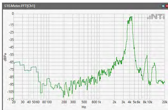
ANSI/TIA 5050-2018 \ 8N HAC OFF \ WB 23.85kbps\ 5.2 Receive path – distortion and noise\5GNR n30
