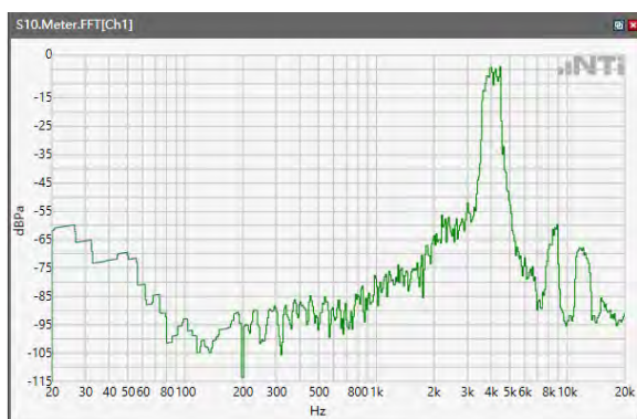
ANSI/TIA 5050-2018 \ 8N HAC OFF \ WB 23.85kbps\ 5.2 Receive path – distortion and noise\LTE Band 48
