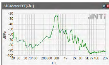
ANSI/TIA 5050-2018 \ 2N HAC OFF \ NB 12.2kbps\ 5.2 Receive path – distortion and noise\LTE Band 26
