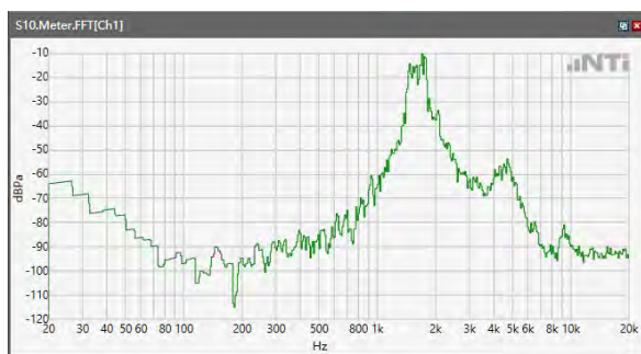
ANSI/TIA 5050-2018 \ 8N HAC OFF \ WB 23.85kbps\ 5.2 Receive path – distortion and noise\LTE Band 41
