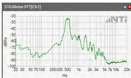
ANSI/TIA 5050-2018 \ 2N HAC OFF \ NB 12.2kbps\ 5.2 Receive path – distortion and noise\LTE Band 25
