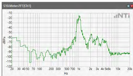
ANSI/TIA 5050-2018 \ 2N HAC OFF \ WB 23.85kbps\ 5.2 Receive path – distortion and noise\LTE Band 7
