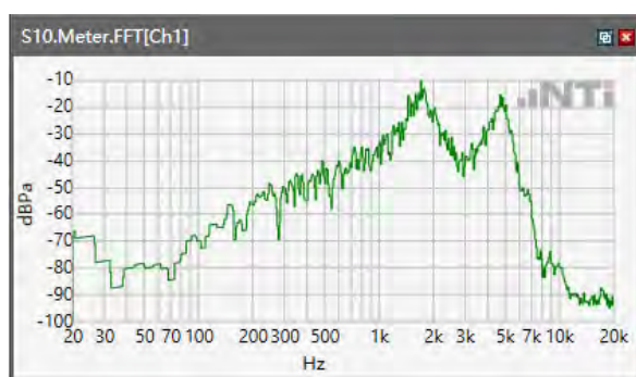
ANSI/TIA 5050-2018 \ 2N HAC OFF \ WB 23.85kbps\ 5.2 Receive path – distortion and noise\WCDMA Band II
