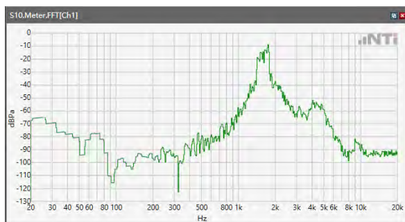
ANSI/TIA 5050-2018 \ 8N HAC OFF \ WB 23.85kbps\ 5.2 Receive path – distortion and noise\5GNR n66
