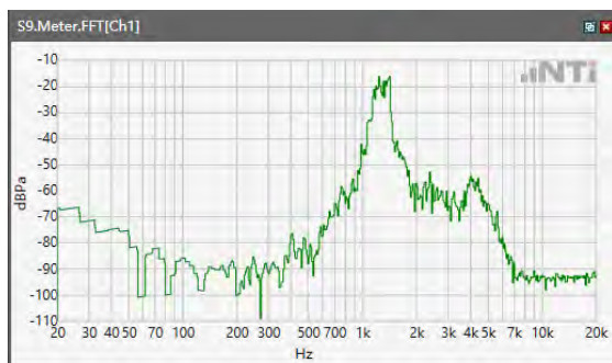
ANSI/TIA 5050-2018 \ 2N HAC OFF \ WB 23.85kbps\ 5.2 Receive path – distortion and noise\LTE Band 71
