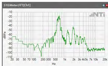
ANSI/TIA 5050-2018 \ 8N HAC OFF \ NB 12.2kbps\ 5.2 Receive path – distortion and noise\LTE Band 30
