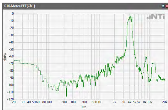
ANSI/TIA 5050-2018 \ 2N HAC OFF \ WB 23.85kbps\ 5.2 Receive path – distortion and noise\LTE Band 48
