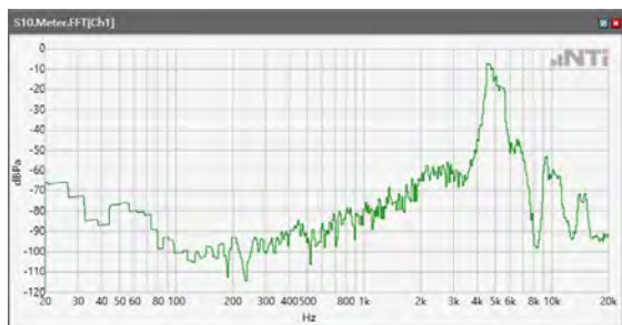
ANSI/TIA 5050-2018 \ 2N HAC OFF \ WB 23.85kbps\ 5.2 Receive path – distortion and noise\5GNR n71
