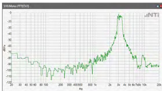
ANSI/TIA 5050-2018 \ 2N HAC OFF \ WB 23.85kbps\ 5.2 Receive path – distortion and noise\5GNR n41
