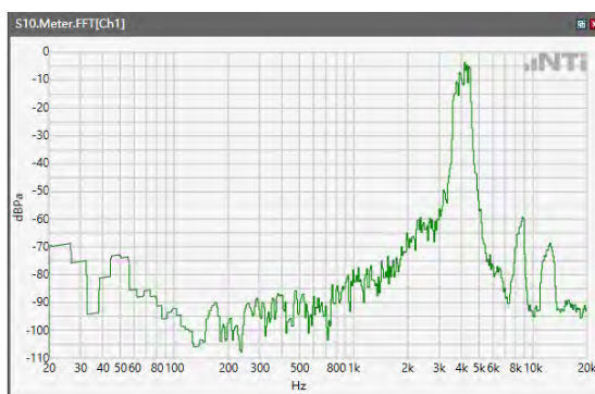
ANSI/TIA 5050-2018 \ 2N HAC OFF \ WB 23.85kbps\ 5.2 Receive path – distortion and noise\ LTE Band 14
