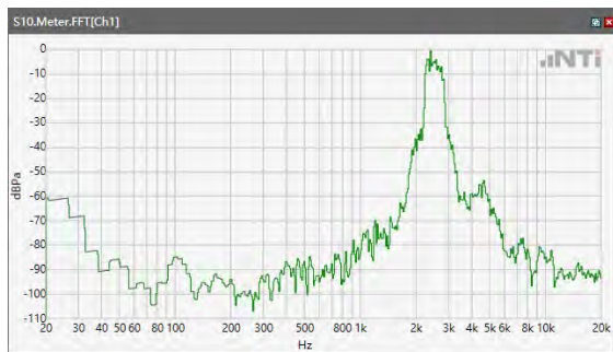
ANSI/TIA 5050-2018 \ 2N HAC OFF \ WB 23.85kbps\ 5.2 Receive path – distortion and noise\5GNR n77
