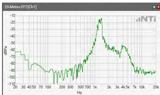
ANSI/TIA 5050-2018 \ 2N HAC OFF \ WB 23.85kbps\ 5.2 Receive path – distortion and noise\LTE Band 30
