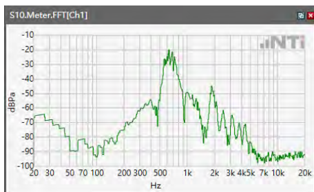
ANSI/TIA 5050-2018 \ 8N HAC OFF \ NB 12.2kbps\ 5.2 Receive path – distortion and noise\LTE Band 71
