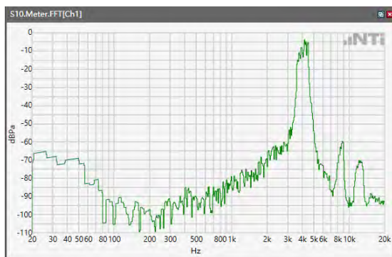
ANSI/TIA 5050-2018 \ 2N HAC OFF \ WB 23.85kbps\ 5.2 Receive path – distortion and noise\LTE Band 30
