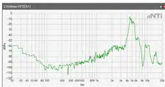
ANSI/TIA 5050-2018 \ 8N HAC OFF \ WB 23.85kbps\ 5.2 Receive path – distortion and noise\5GNR n66
