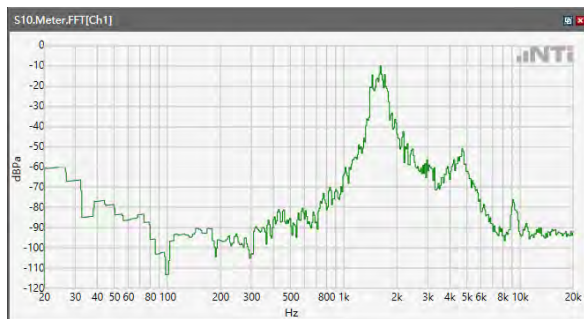
ANSI/TIA 5050-2018 \ 8N HAC OFF \ WB 23.85kbps\ 5.2 Receive path – distortion and noise\LTE Band 26
