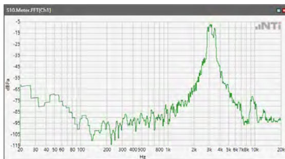
ANSI/TIA 5050-2018 \ 2N HAC OFF \ WB 23.85kbps\ 5.2 Receive path – distortion and noise\WCDMA Band V
