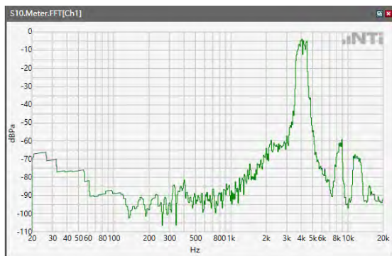
ANSI/TIA 5050-2018 \ 2N HAC OFF \ WB 23.85kbps\ 5.2 Receive path – distortion and noise\LTE Band 66
