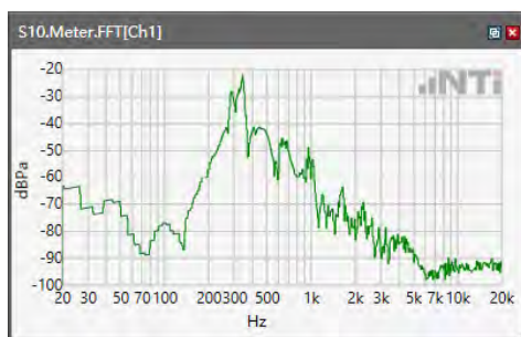
ANSI/TIA 5050-2018 \ 8N HAC OFF \ NB 12.2kbps\ 5.2 Receive path – distortion and noise\5GNR n66
