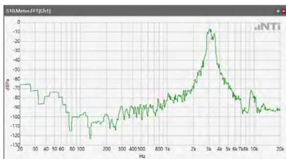
ANSI/TIA 5050-2018 \ 2N HAC OFF \ WB 23.85kbps\ 5.2 Receive path – distortion and noise\WCDMA Band II
