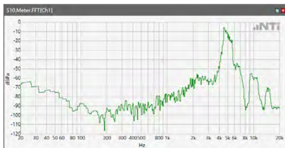
ANSI/TIA 5050-2018 \ 2N HAC OFF \ WB 23.85kbps\ 5.2 Receive path – distortion and noise\WCDMA Band II
