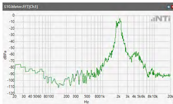
ANSI/TIA 5050-2018 \ 2N HAC OFF \ WB 23.85kbps\ 5.2 Receive path – distortion and noise\LTE Band 13
