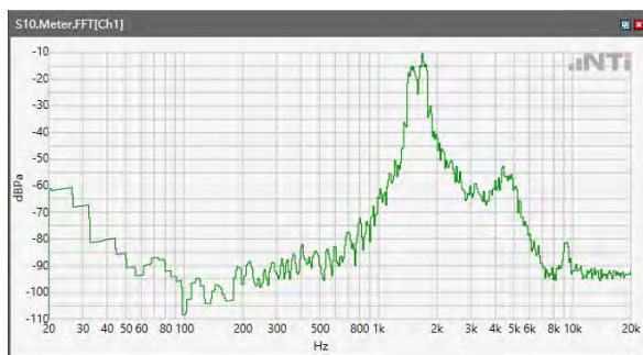
ANSI/TIA 5050-2018 \ 8N HAC OFF \ WB 23.85kbps\ 5.2 Receive path – distortion and noise\ LTE Band 14
