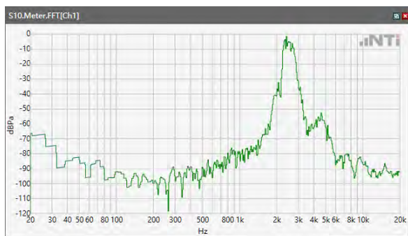
ANSI/TIA 5050-2018 \ 8N HAC OFF \ WB 23.85kbps\ 5.2 Receive path – distortion and noise\5GNR n30
