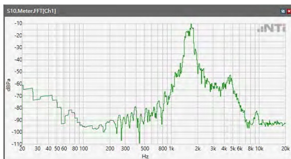
ANSI/TIA 5050-2018 \ 8N HAC OFF \ WB 23.85kbps\ 5.2 Receive path – distortion and noise\LTE Band 12
