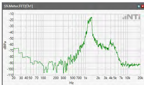
ANSI/TIA 5050-2018 \ 2N HAC OFF \ WB 23.85kbps\ 5.2 Receive path – distortion and noise\LTE Band 48
