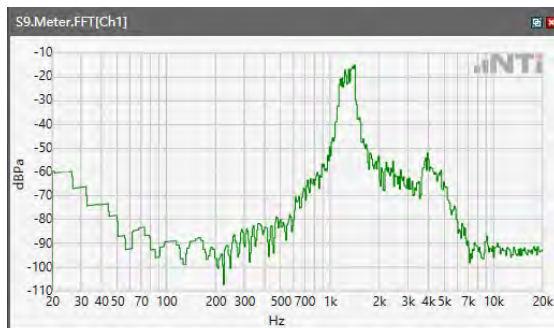
ANSI/TIA 5050-2018 \ 2N HAC OFF \ WB 23.85kbps\ 5.2 Receive path – distortion and noise\LTE Band 25
