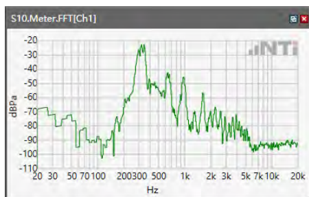
ANSI/TIA 5050-2018 \ 2N HAC OFF \ NB 12.2kbps\ 5.2 Receive path – distortion and noise\WCDMA Band V
