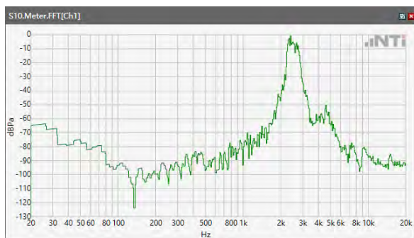
ANSI/TIA 5050-2018 \ 8N HAC OFF \ WB 23.85kbps\ 5.2 Receive path – distortion and noise\5GNR n25
