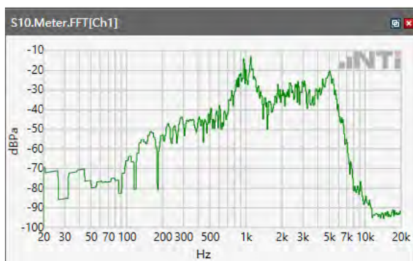
ANSI/TIA 5050-2018 \ 2N HAC OFF \ WB 23.85kbps\ 5.2 Receive path – distortion and noise\LTE Band 41
