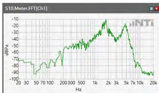
ANSI/TIA 5050-2018 \ 2N HAC OFF \ WB 23.85kbps\ 5.2 Receive path – distortion and noise\WCDMA Band IV
