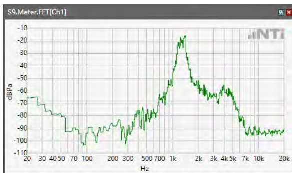
ANSI/TIA 5050-2018 \ 8N HAC OFF \ WB 23.85kbps\ 5.2 Receive path – distortion and noise\LTE Band 7
