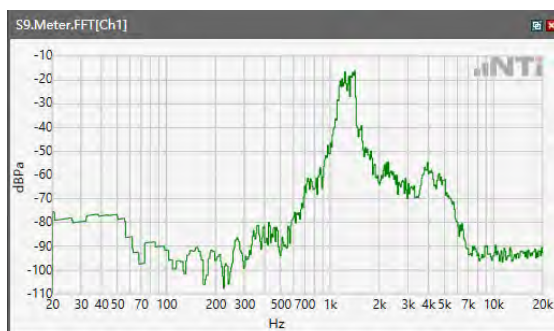
ANSI/TIA 5050-2018 \ 2N HAC OFF \ WB 23.85kbps\ 5.2 Receive path – distortion and noise\ LTE Band 14
