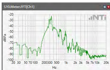
ANSI/TIA 5050-2018 \ 2N HAC OFF \ NB 12.2kbps\ 5.2 Receive path – distortion and noise\5GNR n66
