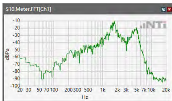
ANSI/TIA 5050-2018 \ 2N HAC OFF \ WB 23.85kbps\ 5.2 Receive path – distortion and noise\WCDMA Band V
