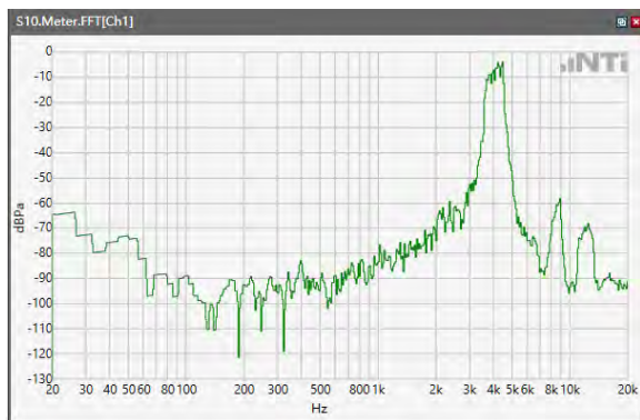
ANSI/TIA 5050-2018 \ 8N HAC OFF \ WB 23.85kbps\ 5.2 Receive path – distortion and noise\LTE Band 30
