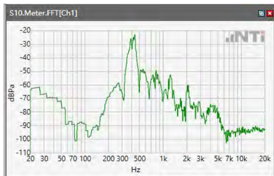
ANSI/TIA 5050-2018 \ 2N HAC OFF \ WB 23.85kbps\ 5.2 Receive path – distortion and noise\WCDMA Band IV
