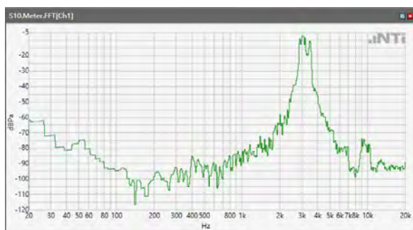
ANSI/TIA 5050-2018 \ 8N HAC OFF \ WB 23.85kbps\ 5.2 Receive path – distortion and noise\5GNR n71
