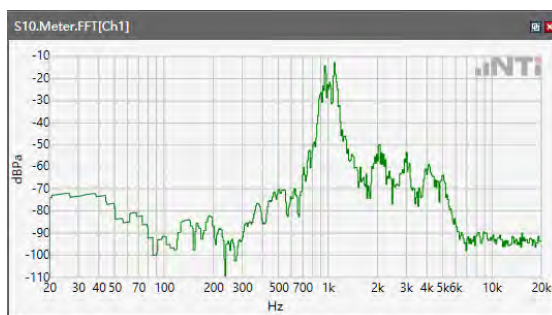
ANSI/TIA 5050-2018 \ 2N HAC OFF \ WB 23.85kbps\ 5.2 Receive path – distortion and noise\LTE Band 13
