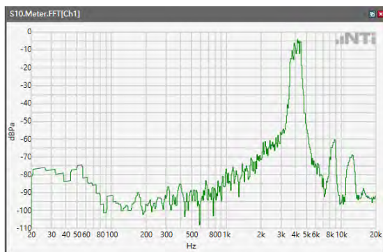
ANSI/TIA 5050-2018 \ 2N HAC OFF \ WB 23.85kbps\ 5.2 Receive path – distortion and noise\LTE Band 26
