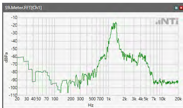
ANSI/TIA 5050-2018 \ 8N HAC OFF \ WB 23.85kbps\ 5.2 Receive path – distortion and noise\5GNR n41
