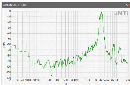
ANSI/TIA 5050-2018 \ 2N HAC OFF \ WB 23.85kbps\ 5.2 Receive path – distortion and noise\LTE Band 13
