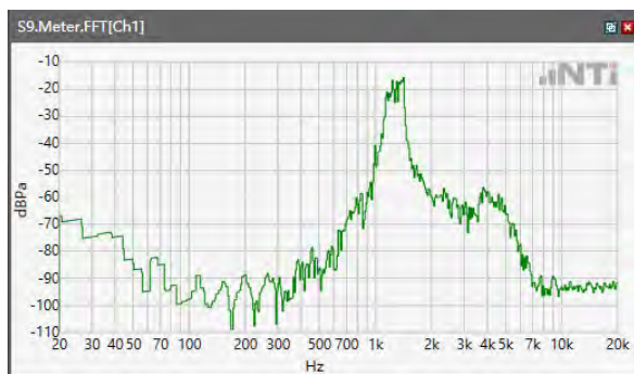
ANSI/TIA 5050-2018 \ 8N HAC OFF \ WB 23.85kbps\ 5.2 Receive path – distortion and noise\5GNR n66
