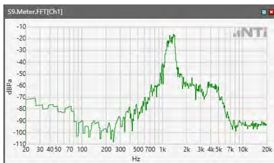
ANSI/TIA 5050-2018 \ 2N HAC OFF \ WB 23.85kbps\ 5.2 Receive path – distortion and noise\LTE Band 5
