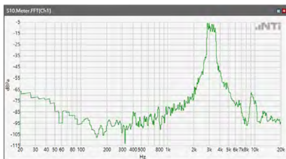
ANSI/TIA 5050-2018 \ 2N HAC OFF \ WB 23.85kbps\ 5.2 Receive path – distortion and noise\5GNR n66
