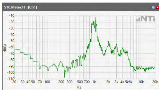
ANSI/TIA 5050-2018 \ 2N HAC OFF \ WB 23.85kbps\ 5.2 Receive path – distortion and noise\LTE Band 5
