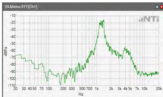
ANSI/TIA 5050-2018 \ 2N HAC OFF \ WB 23.85kbps\ 5.2 Receive path – distortion and noise\LTE Band 7
