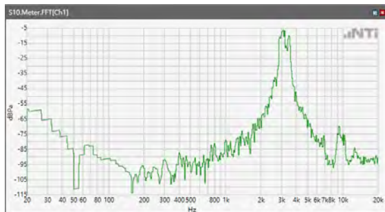
ANSI/TIA 5050-2018 \ 2N HAC OFF \ WB 23.85kbps\ 5.2 Receive path – distortion and noise\5GNR n71
