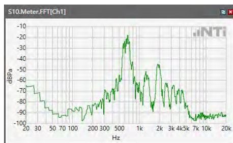
ANSI/TIA 5050-2018 \ 8N HAC OFF \ NB 12.2kbps\ 5.2 Receive path – distortion and noise\5GNR n30
