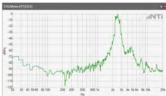
ANSI/TIA 5050-2018 \ 2N HAC OFF \ WB 23.85kbps\ 5.2 Receive path – distortion and noise\5GNR n71
