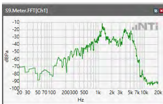
ANSI/TIA 5050-2018 \ 2N HAC OFF \ WB 23.85kbps\ 5.2 Receive path – distortion and noise\5G NR n25
