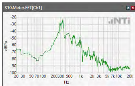
ANSI/TIA 5050-2018 \ 8N HAC OFF \ NB 12.2kbps\ 5.2 Receive path – distortion and noise\5GNR n41
