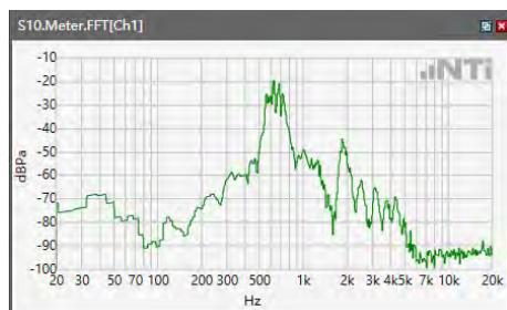
ANSI/TIA 5050-2018 \ 8N HAC OFF \ NB 12.2kbps\ 5.2 Receive path – distortion and noise\LTE Band 26
