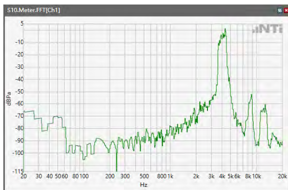
ANSI/TIA 5050-2018 \ 8N HAC OFF \ WB 23.85kbps\ 5.2 Receive path – distortion and noise\LTE Band 26
