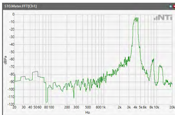
ANSI/TIA 5050-2018 \ 8N HAC OFF \ WB 23.85kbps\ 5.2 Receive path – distortion and noise\ LTE Band 14
