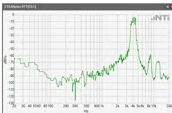
ANSI/TIA 5050-2018 \ 8N HAC OFF \ WB 23.85kbps\ 5.2 Receive path – distortion and noise\LTE Band 13
