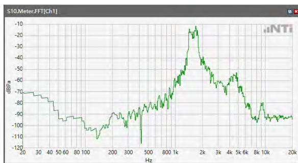
ANSI/TIA 5050-2018 \ 8N HAC OFF \ WB 23.85kbps\ 5.2 Receive path – distortion and noise\LTE Band 25
