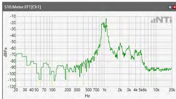
ANSI/TIA 5050-2018 \ 2N HAC OFF \ WB 23.85kbps\ 5.2 Receive path – distortion and noise\LTE Band 12
