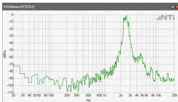
ANSI/TIA 5050-2018 \ 2N HAC OFF \ WB 23.85kbps\ 5.2 Receive path – distortion and noise\5GNR n66
