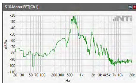
ANSI/TIA 5050-2018 \ 8N HAC OFF \ NB 12.2kbps\ 5.2 Receive path – distortion and noise\5GNR n25
