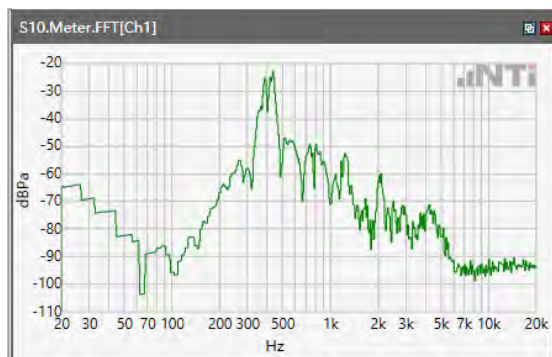
ANSI/TIA 5050-2018 \ 2N HAC OFF \ WB 23.85kbps\ 5.2 Receive path – distortion and noise\LTE Band 25
