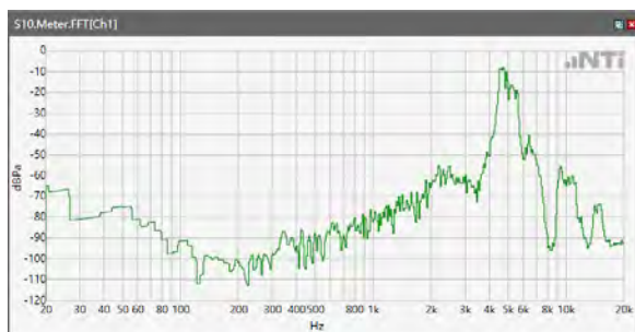
ANSI/TIA 5050-2018 \ 8N HAC OFF \ WB 23.85kbps\ 5.2 Receive path – distortion and noise\5GNR n71
