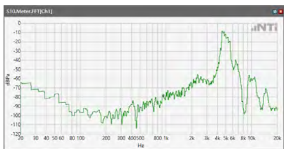
ANSI/TIA 5050-2018 \ 2N HAC OFF \ WB 23.85kbps\ 5.2 Receive path – distortion and noise\WCDMA Band IV
