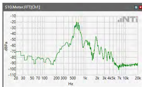
ANSI/TIA 5050-2018 \ 8N HAC OFF \ NB 12.2kbps\ 5.2 Receive path – distortion and noise\LTE Band 25
