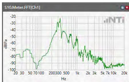
ANSI/TIA 5050-2018 \ 2N HAC OFF \ NB 12.2kbps\ 5.2 Receive path – distortion and noise\WCDMA Band IV
