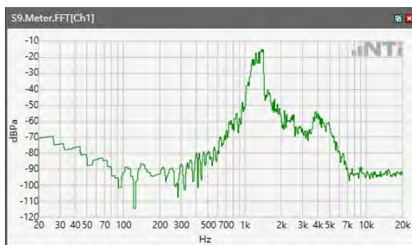
ANSI/TIA 5050-2018 \ 2N HAC OFF \ WB 23.85kbps\ 5.2 Receive path – distortion and noise\LTE Band 41
