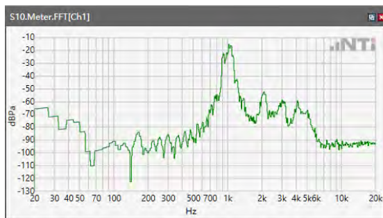
ANSI/TIA 5050-2018 \ 2N HAC OFF \ WB 23.85kbps\ 5.2 Receive path – distortion and noise\ LTE Band 14
