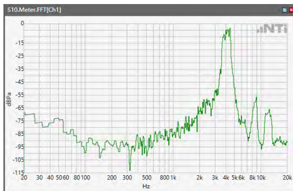
ANSI/TIA 5050-2018 \ 8N HAC OFF \ WB 23.85kbps\ 5.2 Receive path – distortion and noise\5GNR n41
