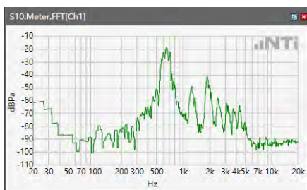
ANSI/TIA 5050-2018 \ 2N HAC OFF \ NB 12.2kbps\ 5.2 Receive path – distortion and noise\LTE Band 13
