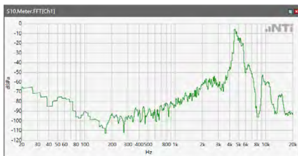
ANSI/TIA 5050-2018 \ 8N HAC OFF \ WB 23.85kbps\ 5.2 Receive path – distortion and noise\5GNR n41
