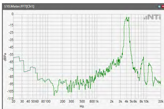
ANSI/TIA 5050-2018 \ 2N HAC OFF \ WB 23.85kbps\ 5.2 Receive path – distortion and noise\LTE Band 12
