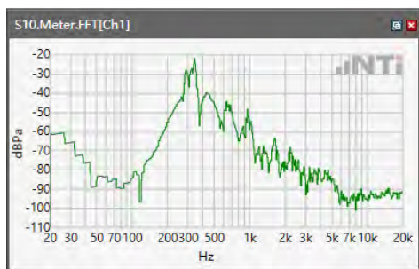
ANSI/TIA 5050-2018 \ 2N HAC OFF \ NB 12.2kbps\ 5.2 Receive path – distortion and noise\WCDMA Band II
