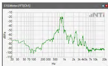
ANSI/TIA 5050-2018 \ 2N HAC OFF \ NB 12.2kbps\ 5.2 Receive path – distortion and noise\5GNR n71
