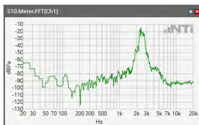
ANSI/TIA 5050-2018 \ 2N HAC OFF \ NB 12.2kbps\ 5.2 Receive path – distortion and noise\LTE Band 30
