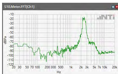
ANSI/TIA 5050-2018 \ 2N HAC OFF \ NB 12.2kbps\ 5.2 Receive path – distortion and noise\LTE Band 66
