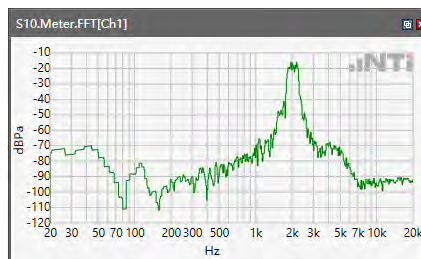
ANSI/TIA 5050-2018 \ 2N HAC OFF \ NB 12.2kbps\ 5.2 Receive path – distortion and noise\LTE Band 41
