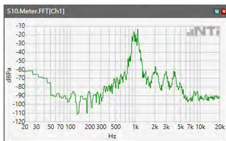
ANSI/TIA 5050-2018 \ 8N HAC OFF \ NB 12.2kbps\ 5.2 Receive path – distortion and noise\5GNR n77
