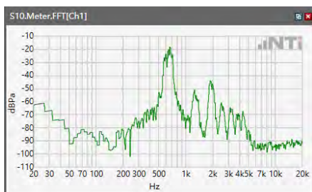
ANSI/TIA 5050-2018 \ 2N HAC OFF \ NB 12.2kbps\ 5.2 Receive path – distortion and noise\5GNR n30
