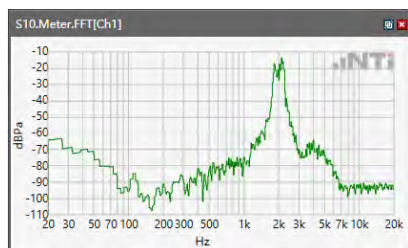
ANSI/TIA 5050-2018 \ 2N HAC OFF \ NB 12.2kbps\ 5.2 Receive path – distortion and noise\LTE Band 5
