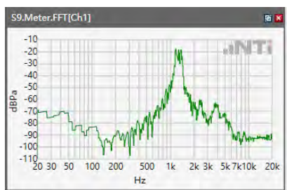
ANSI/TIA 5050-2018 \ 2N HAC OFF \ NB 12.2kbps\ 5.2 Receive path – distortion and noise\5GNR n77
