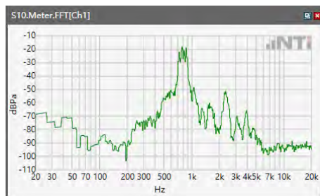
ANSI/TIA 5050-2018 \ 8N HAC OFF \ NB 12.2kbps\ 5.2 Receive path – distortion and noise\LTE Band 12
