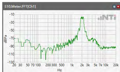
ANSI/TIA 5050-2018 \ 2N HAC OFF \ NB 12.2kbps\ 5.2 Receive path – distortion and noise\LTE Band 66
