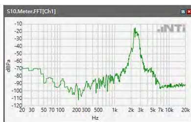
ANSI/TIA 5050-2018 \ 2N HAC OFF \ NB 12.2kbps\ 5.2 Receive path – distortion and noise\LTE Band 7
