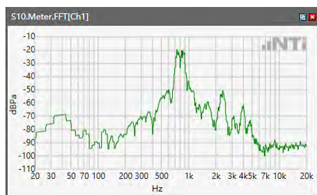
ANSI/TIA 5050-2018 \ 8N HAC OFF \ NB 12.2kbps\ 5.2 Receive path – distortion and noise\LTE Band 7
