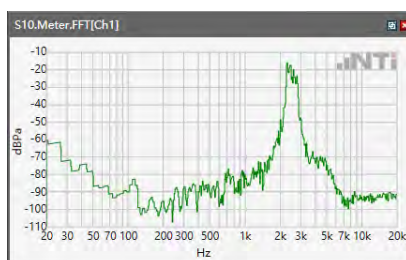
ANSI/TIA 5050-2018 \ 2N HAC OFF \ NB 12.2kbps\ 5.2 Receive path – distortion and noise\LTE Band 41
