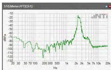
ANSI/TIA 5050-2018 \ 2N HAC OFF \ NB 12.2kbps\ 5.2 Receive path – distortion and noise\LTE Band 5
