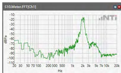
ANSI/TIA 5050-2018 \ 2N HAC OFF \ NB 12.2kbps\ 5.2 Receive path – distortion and noise\WCDMA Band V
