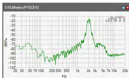
ANSI/TIA 5050-2018 \ 2N HAC OFF \ NB 12.2kbps\ 5.2 Receive path – distortion and noise\LTE Band 12
