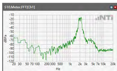
ANSI/TIA 5050-2018 \ 2N HAC OFF \ NB 12.2kbps\ 5.2 Receive path – distortion and noise\LTE Band 7
