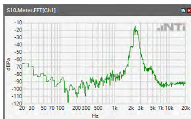
ANSI/TIA 5050-2018 \ 2N HAC OFF \ NB 12.2kbps\ 5.2 Receive path – distortion and noise\5GNR n71
