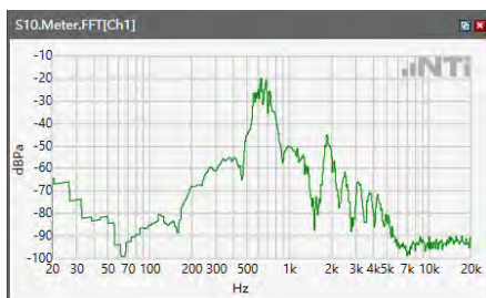
ANSI/TIA 5050-2018 \ 2N HAC OFF \ NB 12.2kbps\ 5.2 Receive path – distortion and noise\5GNR n25
