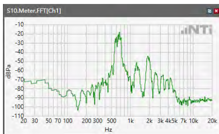
ANSI/TIA 5050-2018 \ 2N HAC OFF \ NB 12.2kbps\ 5.2 Receive path – distortion and noise\5GNR n26
