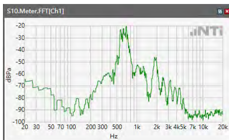
ANSI/TIA 5050-2018 \ 2N HAC OFF \ NB 12.2kbps\ 5.2 Receive path – distortion and noise\5GNR n41
