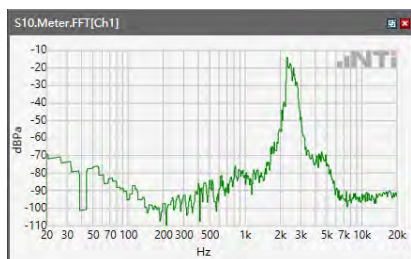
ANSI/TIA 5050-2018 \ 2N HAC OFF \ NB 12.2kbps\ 5.2 Receive path – distortion and noise\LTE Band 12
