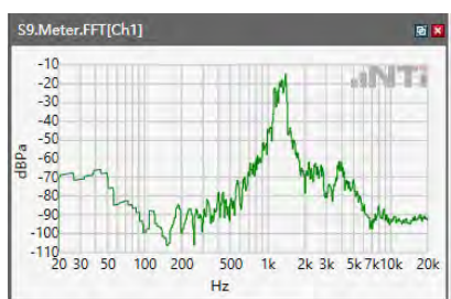
ANSI/TIA 5050-2018 \ 2N HAC OFF \ NB 12.2kbps\ 5.2 Receive path – distortion and noise\5GNR n71
