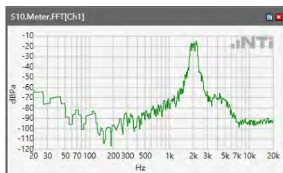
ANSI/TIA 5050-2018 \ 2N HAC OFF \ NB 12.2kbps\ 5.2 Receive path – distortion and noise\LTE Band 48
