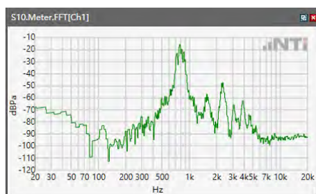
ANSI/TIA 5050-2018 \ 8N HAC OFF \ NB 12.2kbps\ 5.2 Receive path – distortion and noise\5GNR n71
