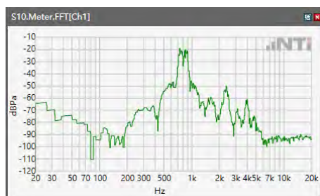
ANSI/TIA 5050-2018 \ 8N HAC OFF \ NB 12.2kbps\ 5.2 Receive path – distortion and noise\LTE Band 13
