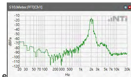
ANSI/TIA 5050-2018 \ 2N HAC OFF \ NB 12.2kbps\ 5.2 Receive path – distortion and noise\LTE Band 30
