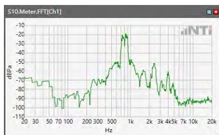
ANSI/TIA 5050-2018 \ 2N HAC OFF \ NB 12.2kbps\ 5.2 Receive path – distortion and noise\5GNR n77
