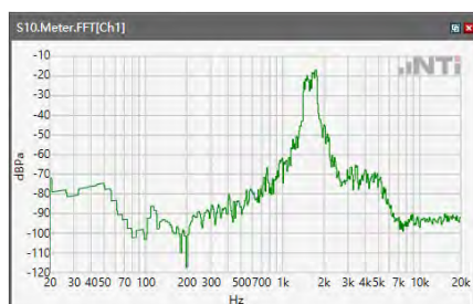
ANSI/TIA 5050-2018 \ 8N HAC OFF \ NB 12.2kbps\ 5.2 Receive path – distortion and noise\5GNR n71
