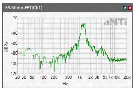
ANSI/TIA 5050-2018 \ 2N HAC OFF \ NB 12.2kbps\ 5.2 Receive path – distortion and noise\5GNR n66
