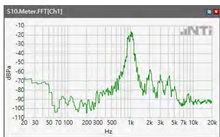
ANSI/TIA 5050-2018 \ 2N HAC OFF \ NB 12.2kbps\ 5.2 Receive path – distortion and noise\5GNR n77
