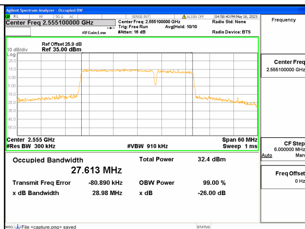
Band7C / 20+10MHz / 64QAM/ High CH
