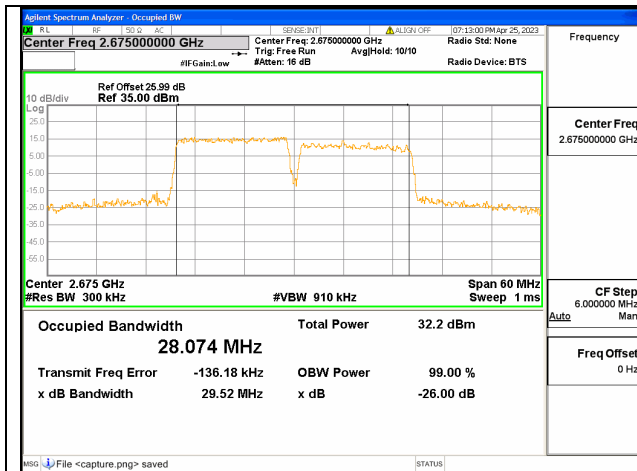
Band41C / 15+15MHz / QPSK/ High CH
