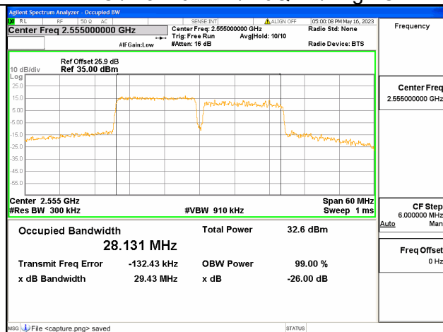
Band7C / 15+15MHz / QPSK/ High CH
