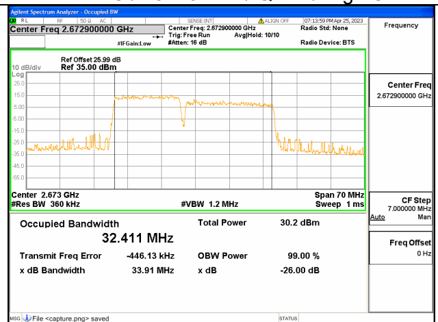
Band41C / 15+20MHz / 64QAM/ High CH
