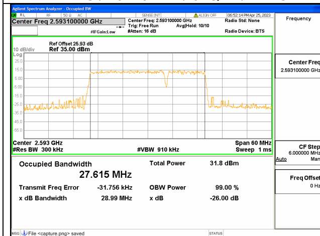
Band41C / 20+10MHz / 16QAM/ Mid CH
