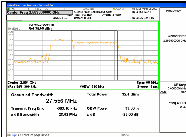
Band41C / 10+20MHz / QPSK/ Mid CH
