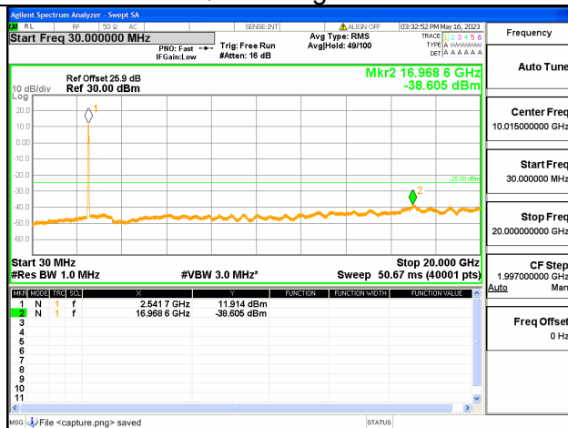
Band7C-30M-20G / 15+20MHz / 75RB+100RB/ QPSK / High CH
