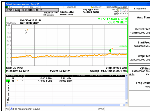
Band7C-30M-20G / 15+15MHz / 1RB+1RB/ QPSK / Mid CH
