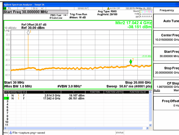
Band7C-30M-20G / 15+20MHz / 1RB+1RB/ QPSK / Low CH
