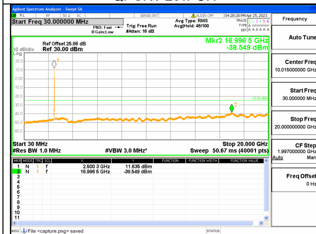
Band41C-30M-20G / 5+20MHz / 25RB+100RB/ QPSK / Low CH
