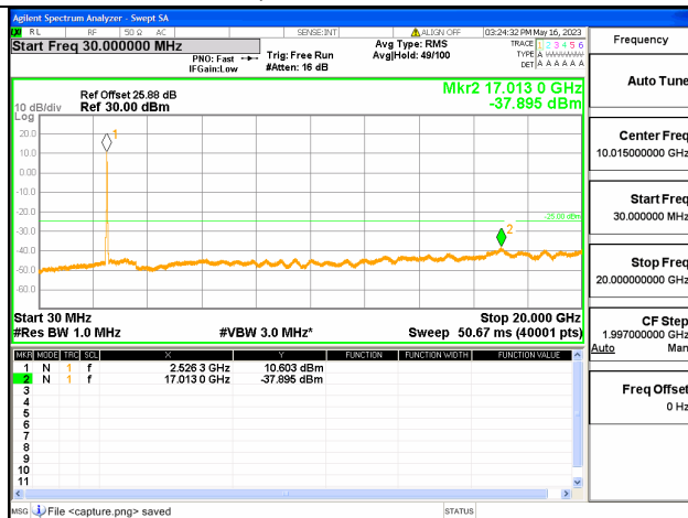
Band7C-30M-20G / 20+20MHz /100RB+100RB/ QPSK / Mid CH
