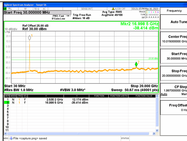
Band7C-30M-20G / 15+20MHz / 75RB+100RB/ QPSK / Mid CH
