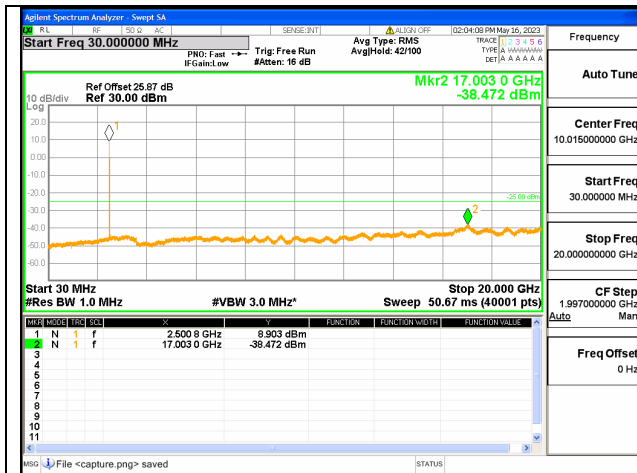
Band7C-30M-20G / 15+20MHz / 1RB+1RB/ QPSK / Low CH
