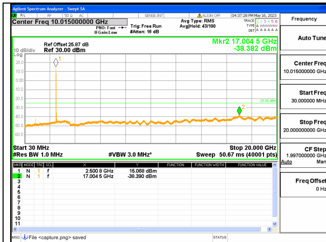
Band7C-30M-20G / 15+15MHz / 1RB+1RB/ QPSK / Low CH
