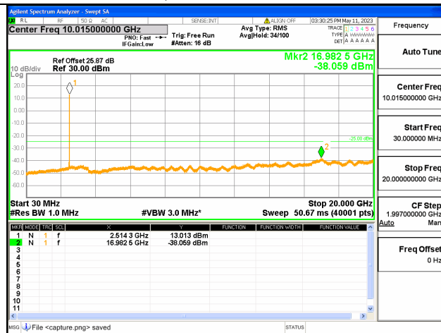
Band7C-30M-20G / 15+15MHz / 1RB+1RB/ QPSK / Low CH
