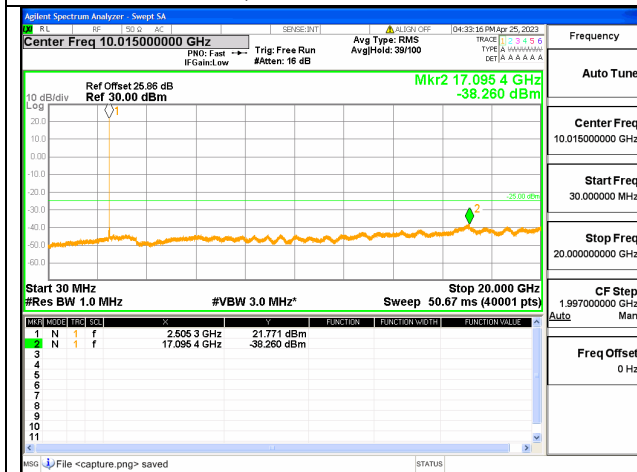
Band41C-30M-20G / 10+15MHz /1RB+1RB/ QPSK / Low CH
