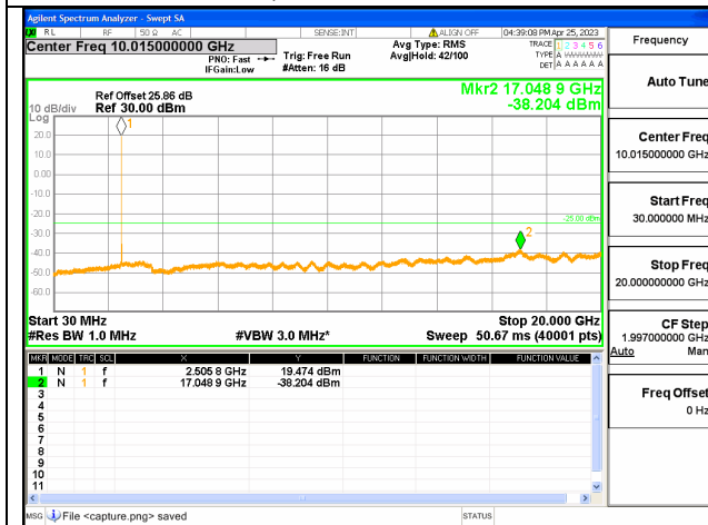
Band41C-30M-20G / 10+20MHz / 1RB+1RB/ QPSK / Low CH
