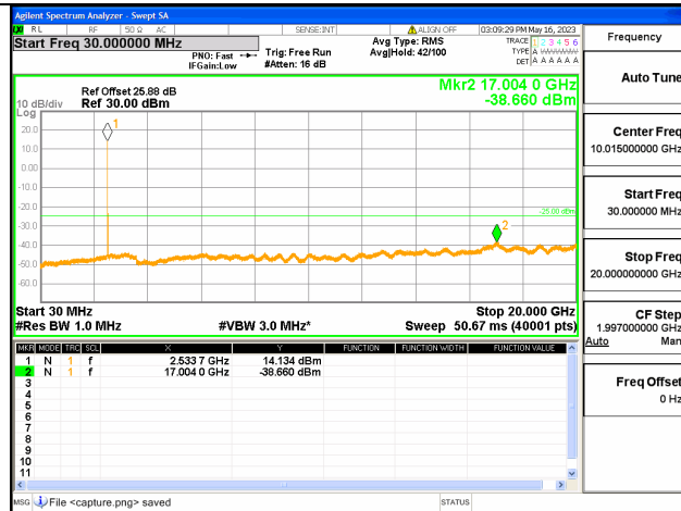
Band7C-30M-20G / 15+15MHz / 1RB+1RB/ QPSK / Mid CH
