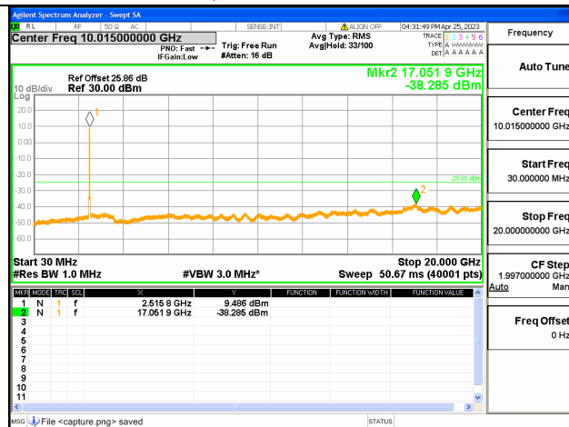
Band41C-30M-20G / 20+5MHz / 100RB+25RB/ QPSK / Low CH
