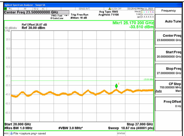
Band7C-20G-27G / 15+15MHz / 1RB+1RB/ QPSK / Low CH
