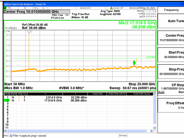
Band41C-30M-20G / 20+5MHz / 1RB+1RB/ QPSK / Low CH
