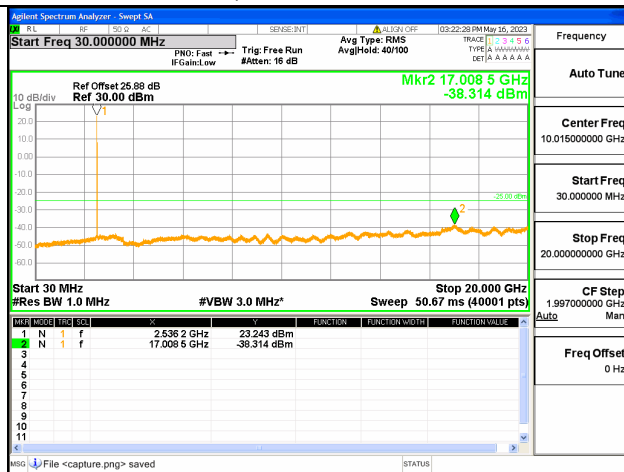
Band7C-30M-20G / 20+15MHz /1RB+1RB/ QPSK / Mid CH
