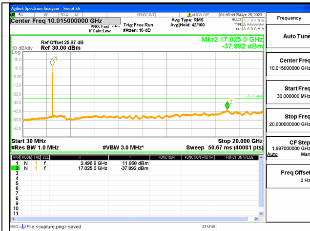
Band41C-30M-20G / 20+15MHz / 1RB+1RB/ QPSK / Low CH
