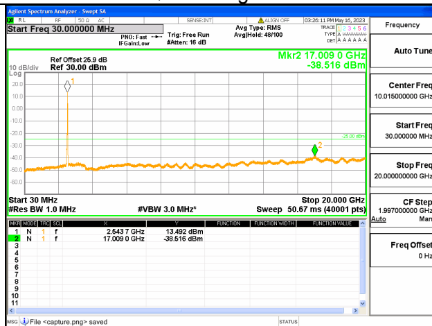
Band7C-30M-20G / 10+20MHz / 50RB+100RB/ QPSK / High CH
