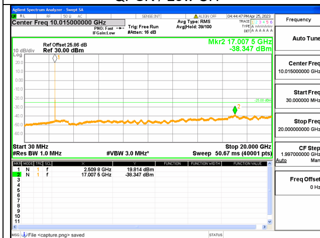
Band41C-30M-20G / 15+15MHz / 1RB+1RB/ QPSK / Low CH
