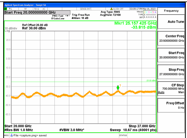
Band7C-20G-27G / 15+15MHz / 1RB+1RB/ QPSK / Mid CH
