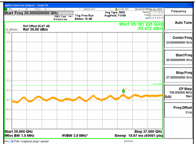
Band7C-20G-27G / 20+15MHz / 1RB+1RB/ QPSK / Low CH
