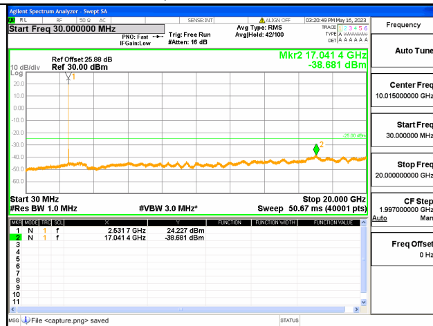
Band7C-30M-20G / 15+20MHz / 1RB+1RB/ QPSK / Mid CH
