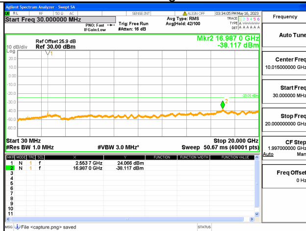
Band7C-30M-20G / 20+15MHz / 1RB+1RB/ QPSK / High CH
