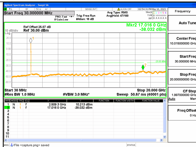
Band7C-30M-20G / 20+20MHz / 100RB+100RB / QPSK / Low CH
