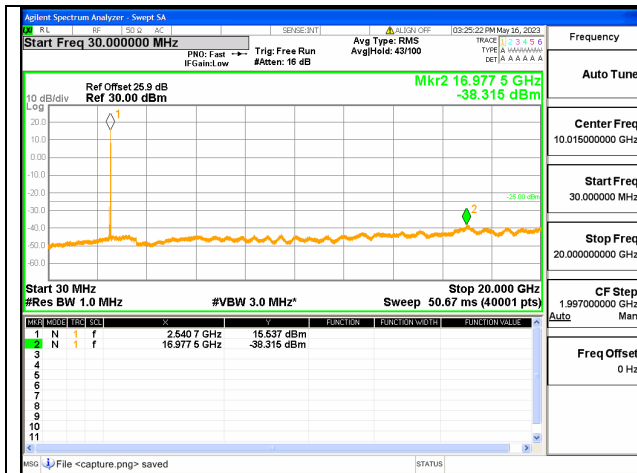
Band7C-30M-20G / 10+20MHz / 1RB+1RB/ QPSK / High CH
