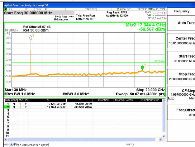
Band7C-30M-20G / 20+20MHz / 1RB+1RB / QPSK / Low CH
