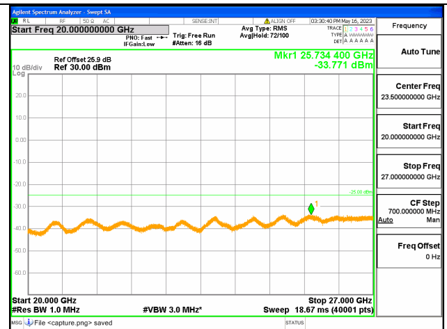
Band7C-20G-27G / 15+15MHz / 1RB+1RB/ QPSK / High CH
