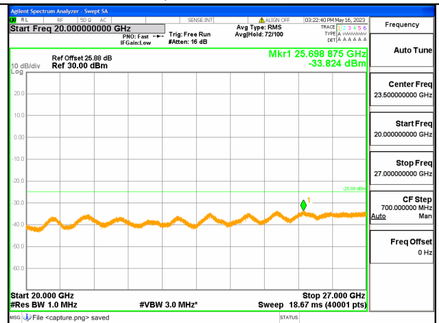
Band7C-20G-27G / 20+15MHz /1RB+1RB/ QPSK / Mid CH
