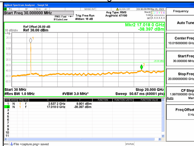
Band7C-30M-20G / 20+20MHz /100RB+100RB/ QPSK / High CH
