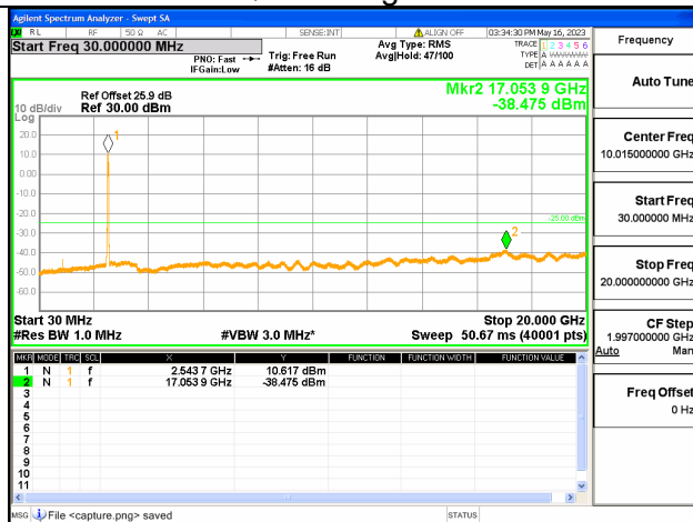
Band7C-30M-20G / 20+15MHz / 100RB+75RB/ QPSK / High CH
