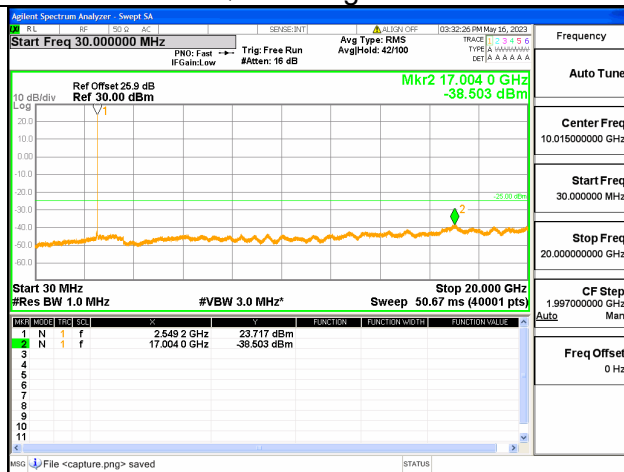
Band7C-30M-20G / 15+20MHz / 1RB+1RB/ QPSK / High CH
