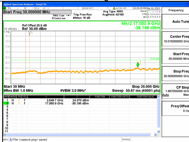
Band7C-30M-20G / 10+20MHz / 1RB+1RB/ QPSK / High CH
