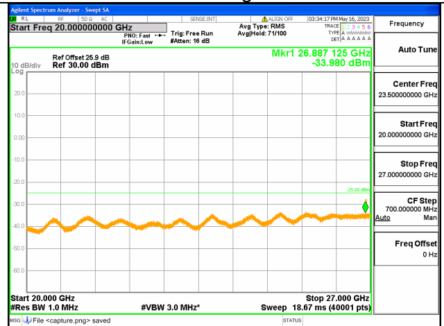
Band7C-20G-27G / 20+15MHz / 1RB+1RB/ QPSK / High CH
