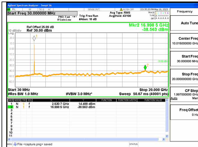
Band7C-30M-20G / 20+20MHz / 1RB+1RB/ QPSK / High CH
