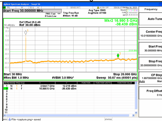
Band7C-30M-20G / 15+15MHz / 75RB+75RB/ QPSK / High CH
