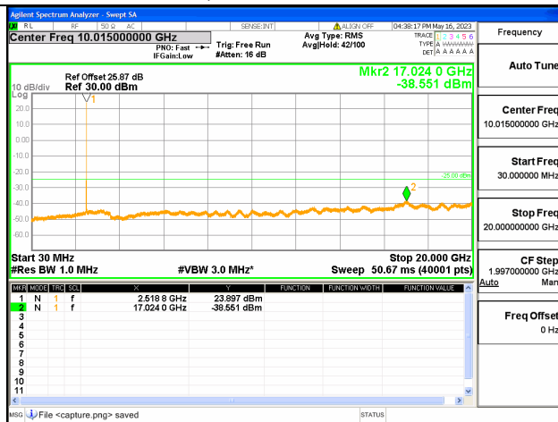
Band7C-30M-20G / 20+15MHz / 1RB+1RB/ QPSK / Low CH
