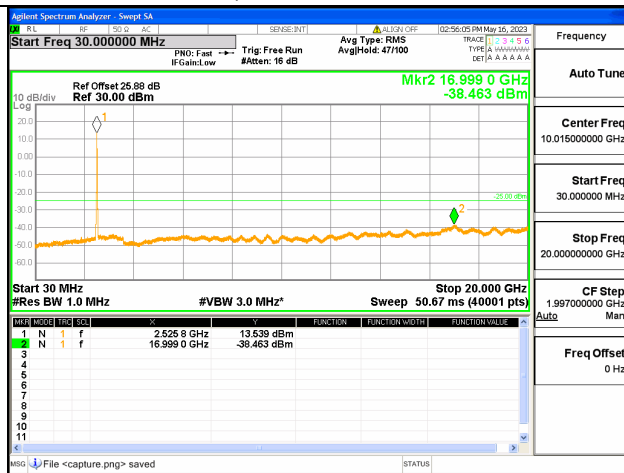
Band7C-30M-20G / 10+20MHz / 50RB+100RB/ QPSK / Mid CH
