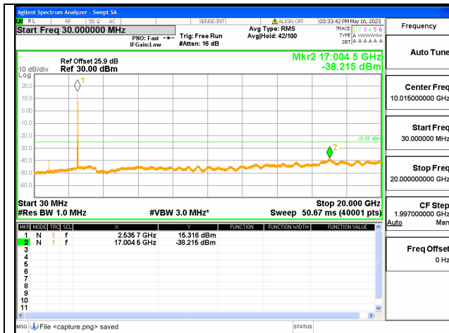
Band7C-30M-20G / 20+15MHz / 1RB+1RB/ QPSK / High CH
