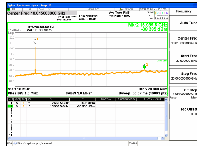
Band41C-30M-20G / 10+15MHz /1RB+1RB/ QPSK / High CH
