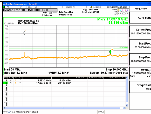
Band41C-30M-20G / 20+5MHz / 100RB+25RB / QPSK / Mid CH
