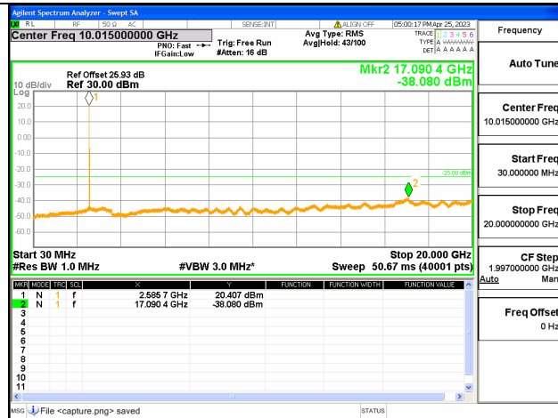
Band41C-30M-20G / 5+20MHz / 1RB+1RB/ QPSK / Mid CH
