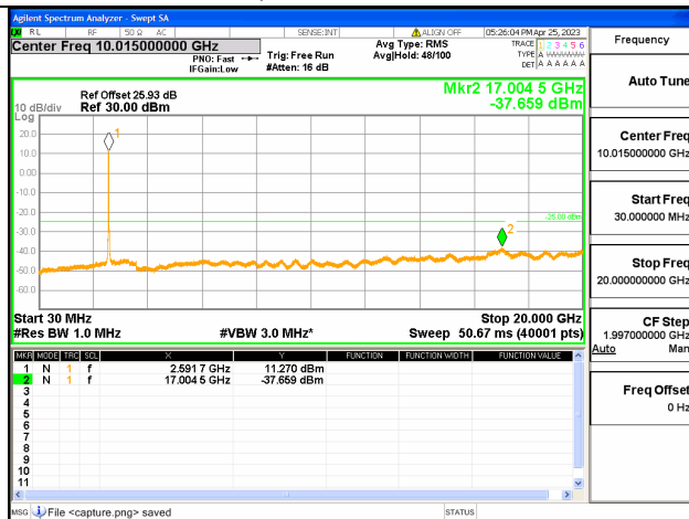
Band41C-30M-20G / 15+10MHz / 75RB+50RB/ QPSK / Mid CH
