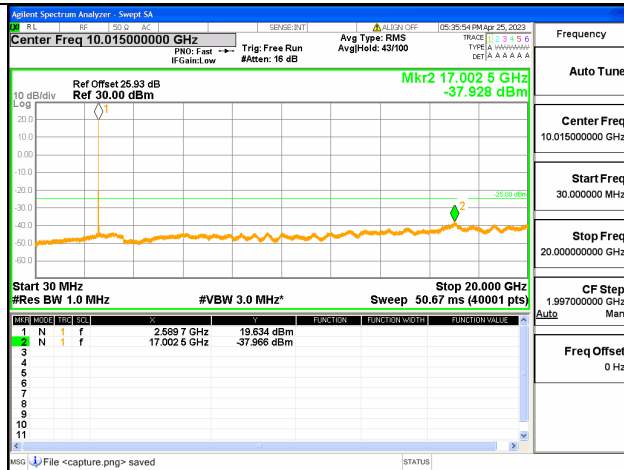
Band41C-30M-20G / 15+20MHz / 1RB+1RB/ QPSK / Mid CH
