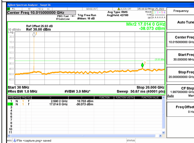
Band41C-30M-20G / 10+15MHz /1RB+1RB/ QPSK / Mid CH
