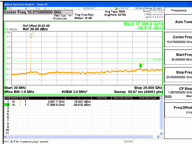
Band41C-30M-20G / 15+15MHz / 1RB+1RB/ QPSK / Mid CH
