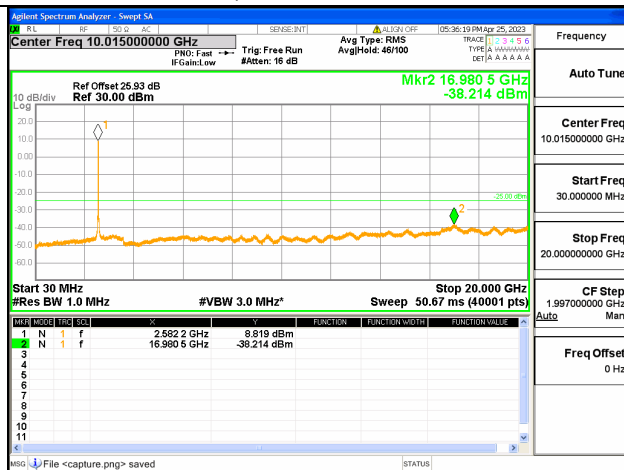
Band41C-30M-20G / 15+20MHz /75RB+100RB/ QPSK / Mid CH
