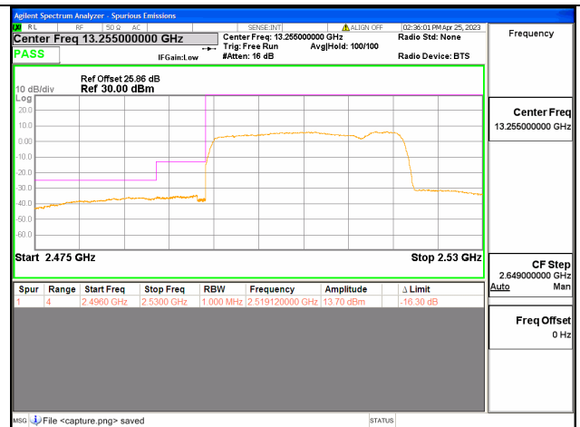
Band41C / 20+5MHz / Low CH / QPSK / 100 RB
