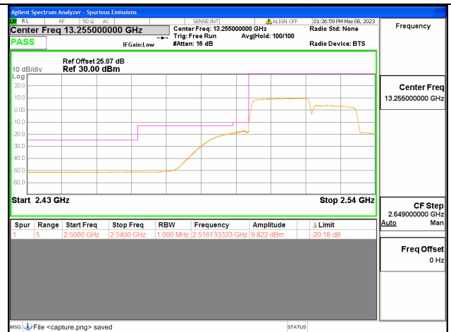
Band7C / 20+15MHz / Low CH / QPSK / 100 RB
