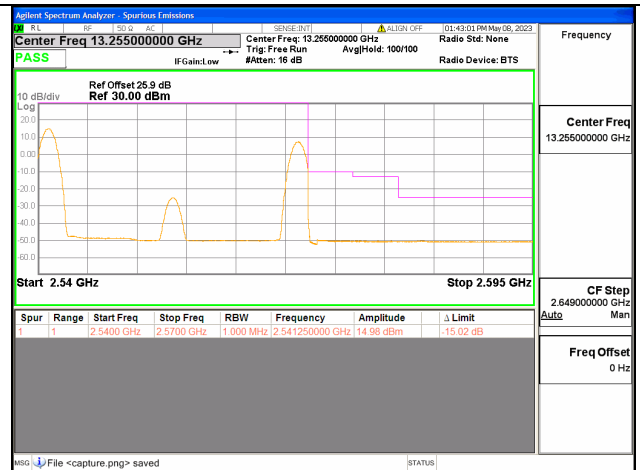
Band7C / 10+20MHz / High CH / QPSK / 1 RB
