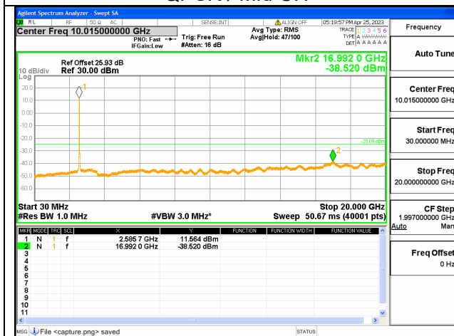
Band41C-30M-20G / 10+15MHz /50RB+75RB/ QPSK / Mid CH
