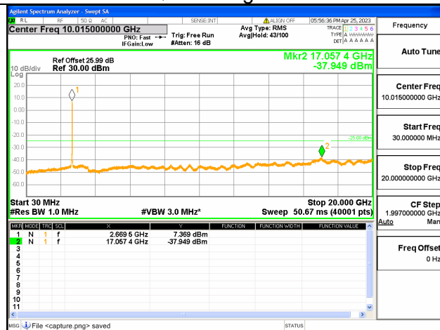
Band41C-30M-20G / 20+5MHz / 100RB+25RB/ QPSK / High CH
