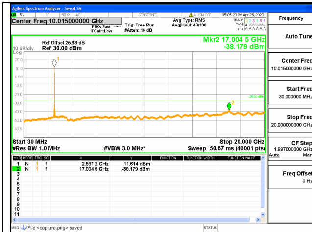
Band41C-30M-20G / 20+5MHz / 1RB+1RB / QPSK / Mid CH
