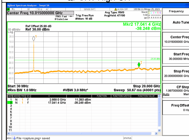
Band41C-30M-20G / 10+15MHz /50RB+75RB/ QPSK / High CH
