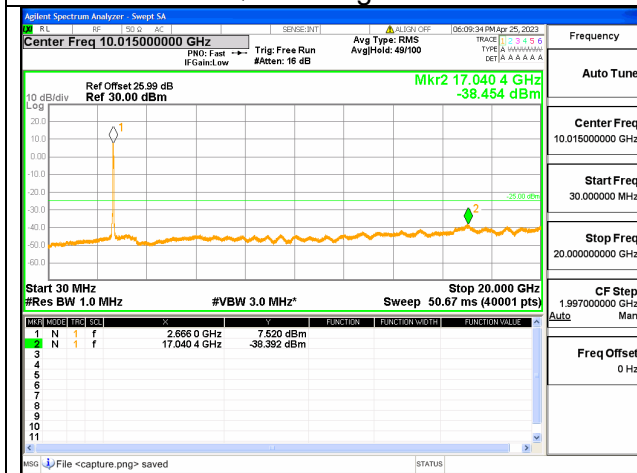
Band41C-30M-20G / 20+20MHz /100RB+100RB/ QPSK / High CH
