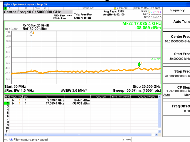
Band41C-30M-20G / 5+20MHz / 1RB+1RB/ QPSK / High CH
