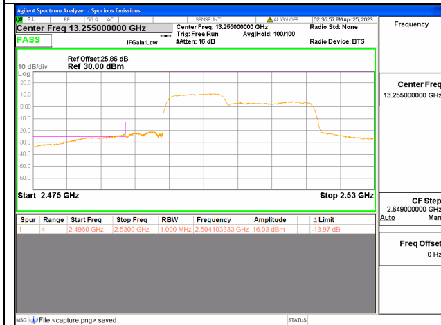
Band41C / 10+15MHz / Low CH / QPSK / 50 RB
