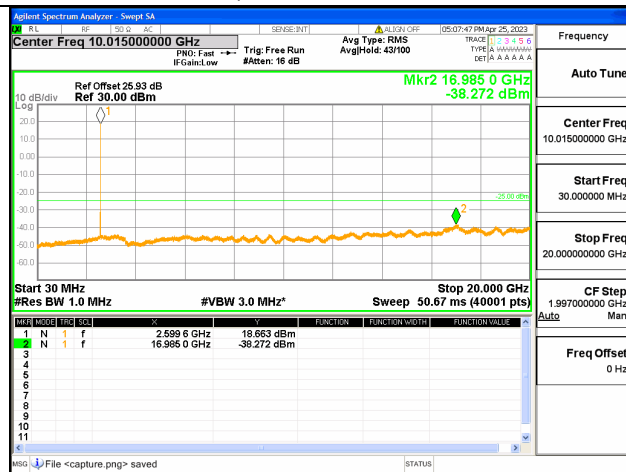
Band41C-30M-20G / 20+5MHz / 1RB+1RB / QPSK / Mid CH
