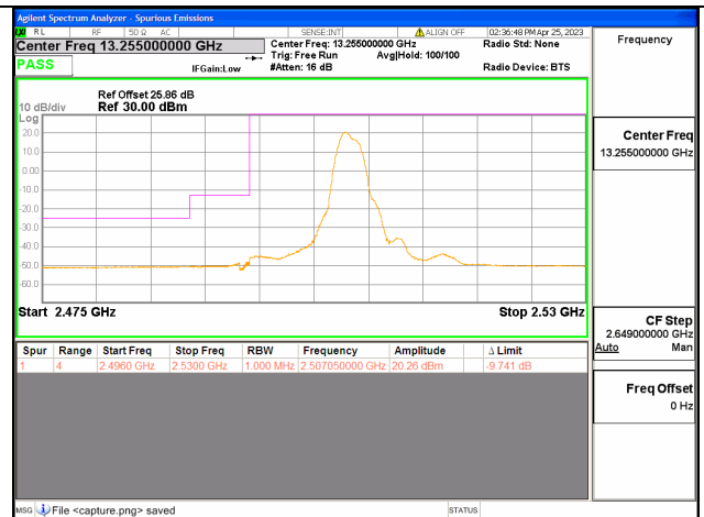
Band41C / 10+15MHz / Low CH / QPSK / 1 RB
