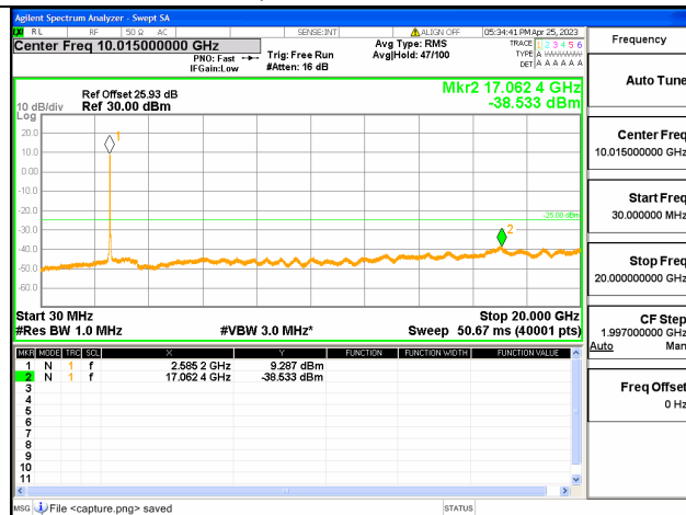
Band41C-30M-20G / 15+15MHz / 75RB+75RB/ QPSK / Mid CH
