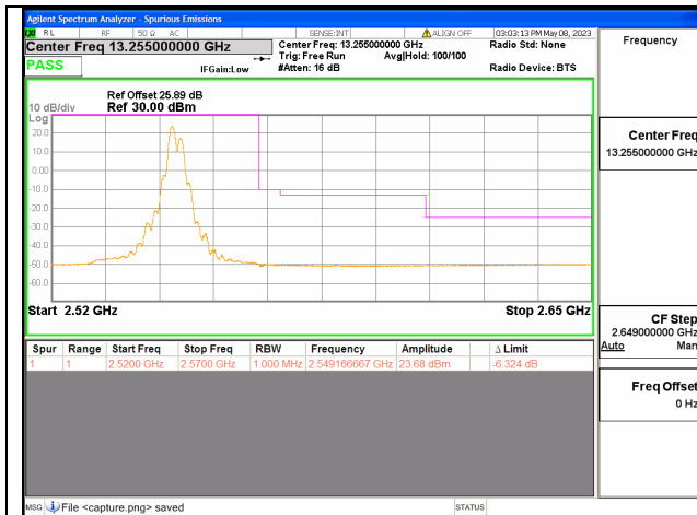
Band7C / 20+20MHz / High CH / QPSK / 1 RB
