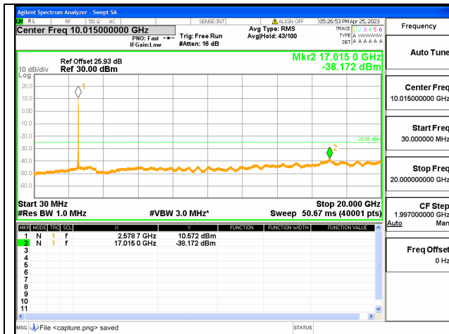
Band41C-30M-20G / 10+20MHz / 1RB+1RB/ QPSK / Mid CH
