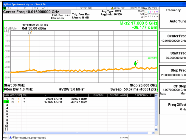
Band41C-30M-20G / 15+10MHz / 1RB+1RB/ QPSK / Mid CH
