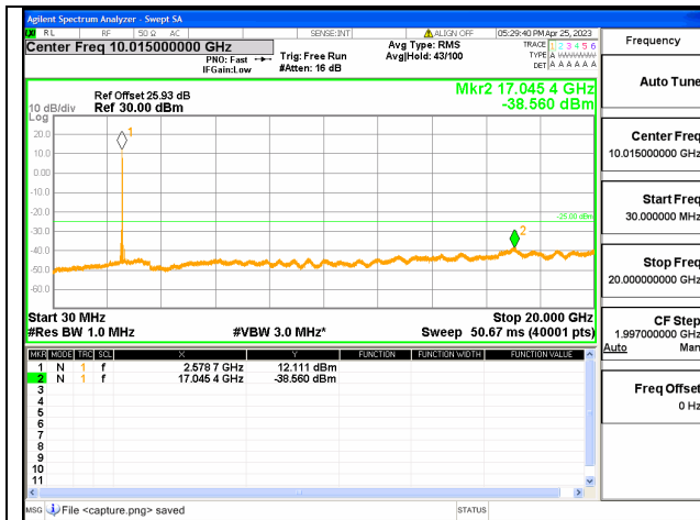
Band41C-30M-20G / 20+10MHz / 1RB+1RB/ QPSK / Mid CH
