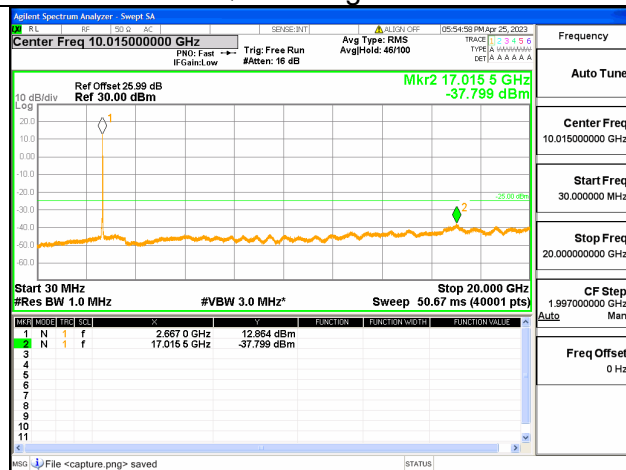
Band41C-30M-20G / 5+20MHz / 25RB+100RB/ QPSK / High CH
