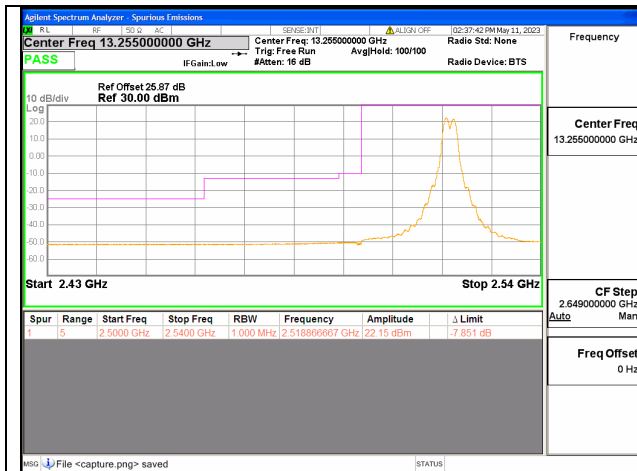
Band7C / 20+15MHz / Low CH / QPSK / 1 RB
