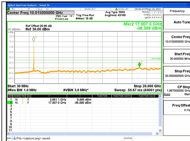
Band41C-30M-20G / 20+20MHz / 1RB+1RB/ QPSK / High CH
