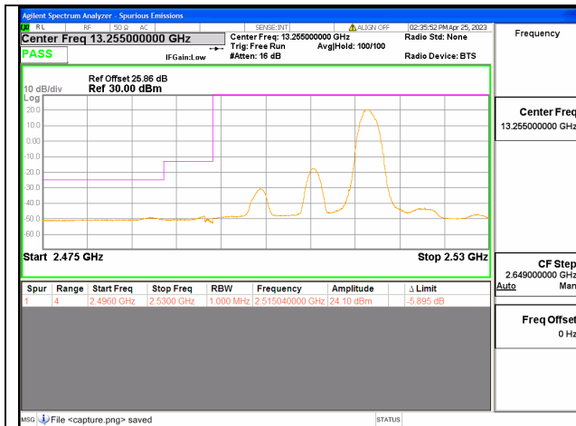
Band41C / 20+5MHz / Low CH / QPSK / 1 RB
