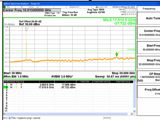
Band41C-30M-20G / 20+5MHz / 1RB+1RB/ QPSK / High CH
