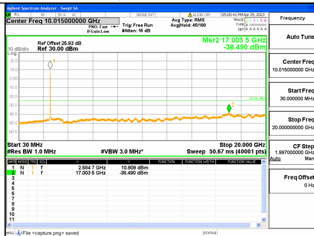
Band41C-30M-20G / 5+20MHz / 25RB+100RB/ QPSK / Mid CH
