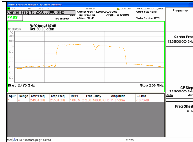
Band41C / 20+15MHz / Low CH / QPSK / 100 RB
