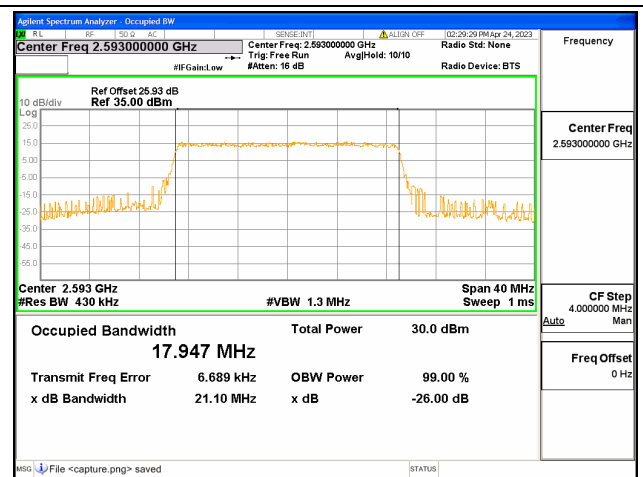
Band41 / 20MHz / 16QAM/ Mid CH
