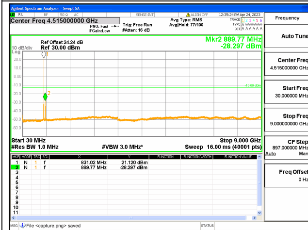
Band19 / 15MHz / High CH / QPSK
