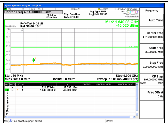
Band18 part22 / 5MHz / Mid CH / QPSK
