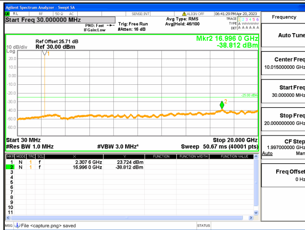
Band30-30M-20G / 5MHz / Mid CH / QPSK
