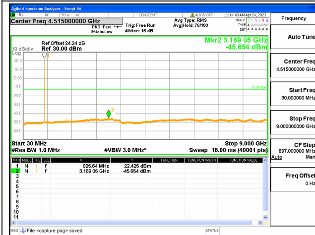
Band18 part22 / 5MHz / High CH / QPSK
