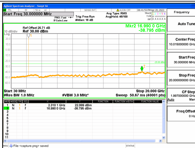
Band30-30M-20G / 5MHz / High CH / QPSK
