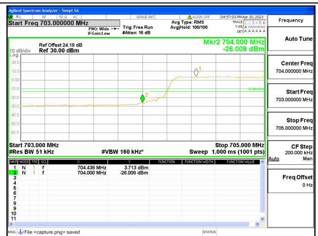
Band17 / 5MHz / Low CH / QPSK / FULL RB
