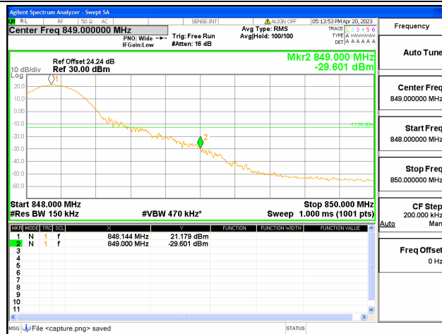
Band26 Part22 / 15MHz / High CH / QPSK / 1 RB
