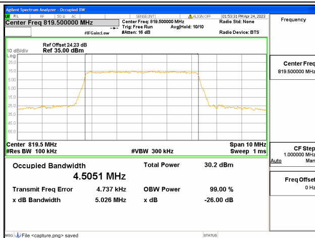
Band18 part90 / 5MHz / 16QAM/ Mid CH
