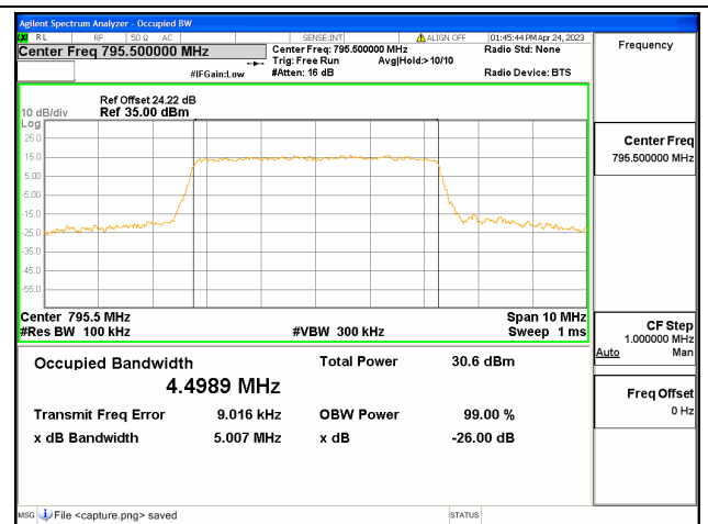
Band14 / 5MHz / 16QAM/ High CH
