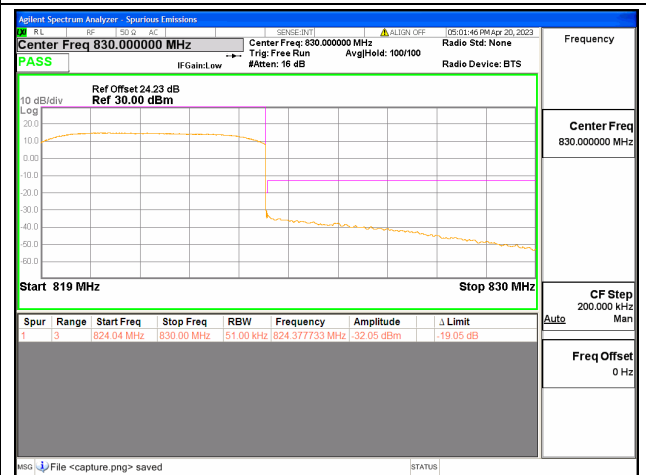
Band18 part90 / 5MHz / High CH / QPSK / FULL RB
