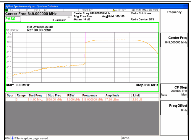
Band26 Part90 / 5MHz / Low CH / QPSK / FULL RB
