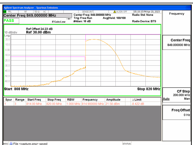
Band26 Part90 / 1.4MHz / Low CH / QPSK / FULL RB
