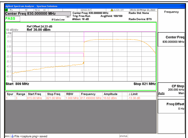
Band18 part90 / 5MHz / Low CH / QPSK / FULL RB
