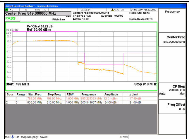
Band14 / 10MHz / High CH / QPSK / FULL RB
