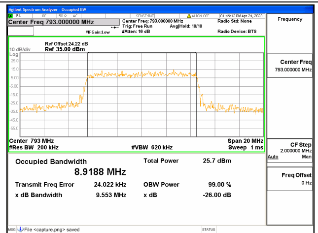
Band14 / 10MHz / 64QAM/ Mid CH
