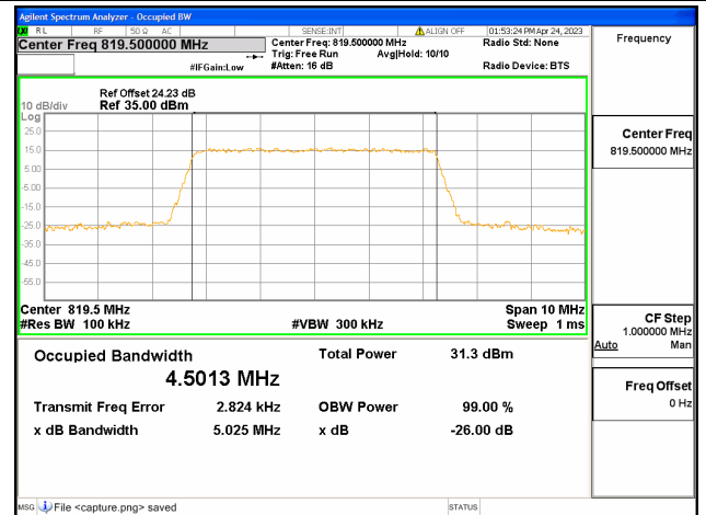
Band18 part90 / 5MHz / QPSK/ Mid CH
