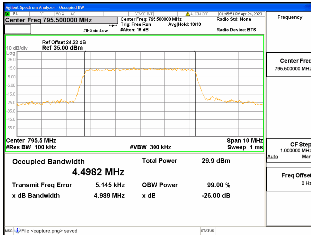
Band14 / 5MHz / 64QAM/ High CH
