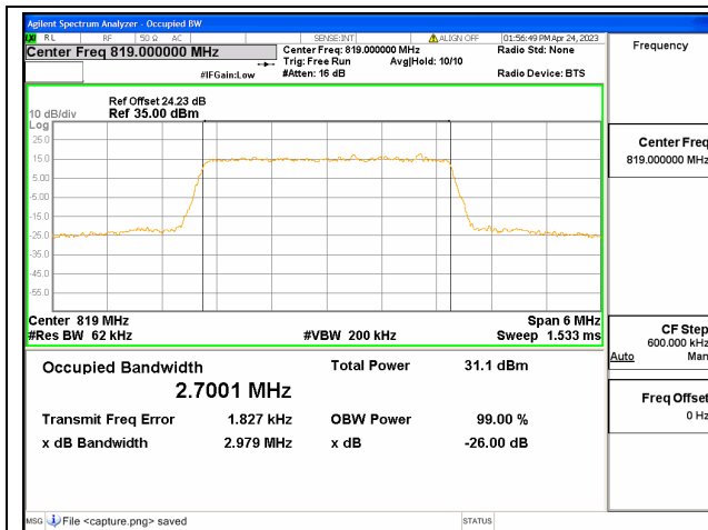
Band26 Part90 / 3MHz / QPSK/ Mid CH
