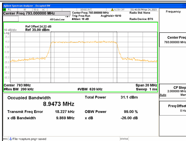
Band14 / 10MHz / 16QAM/ Mid CH
