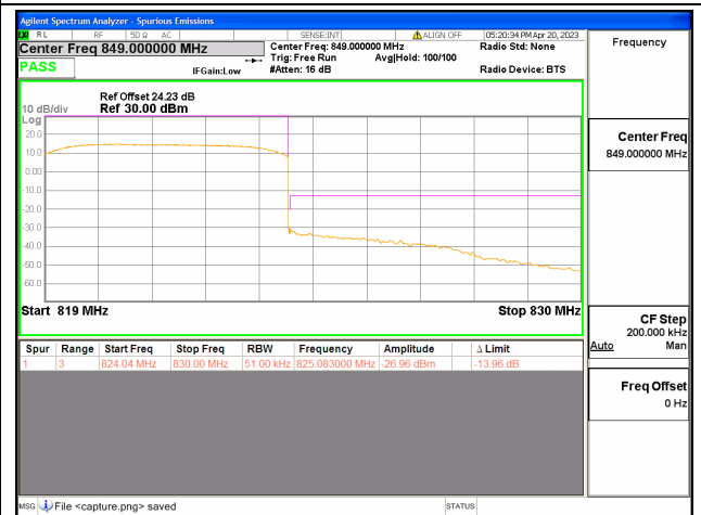
Band26 Part90 / 5MHz / High CH / QPSK / FULL RB
