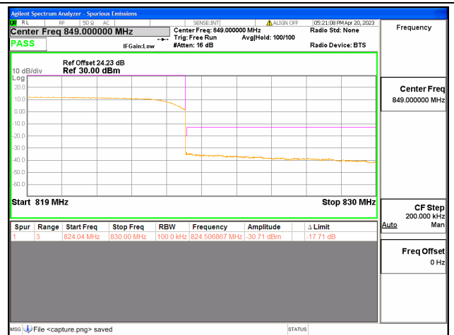
Band26 Part90 / 10MHz / High CH / QPSK / FULL RB
