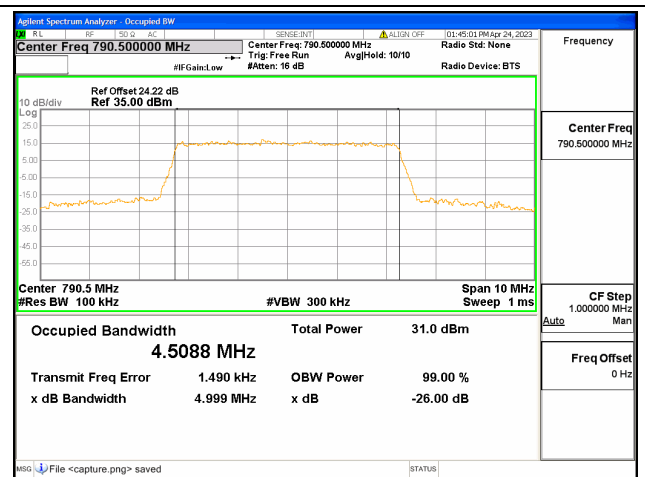
Band14 / 5MHz / 16QAM/ Low CH
