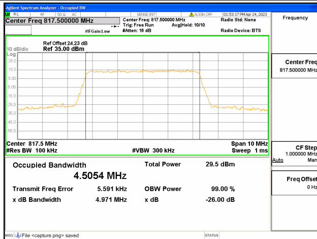
Band18 part90 / 5MHz / 64QAM/ Low CH
