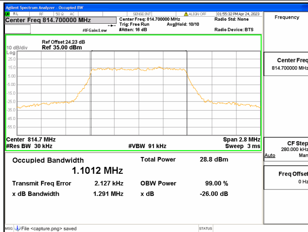
Band26 Part90 / 1.4MHz / 64QAM/ Low CH
