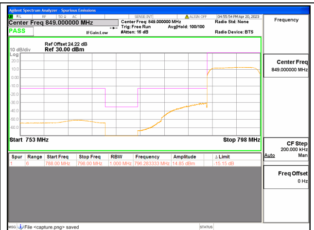
Band14 / 10MHz / Low CH / QPSK / FULL RB
