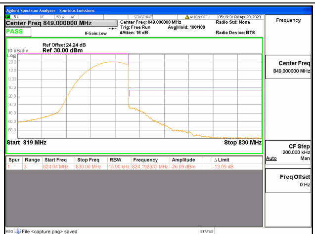
Band26 Part90 / 1.4MHz / High CH / QPSK / FULL RB
