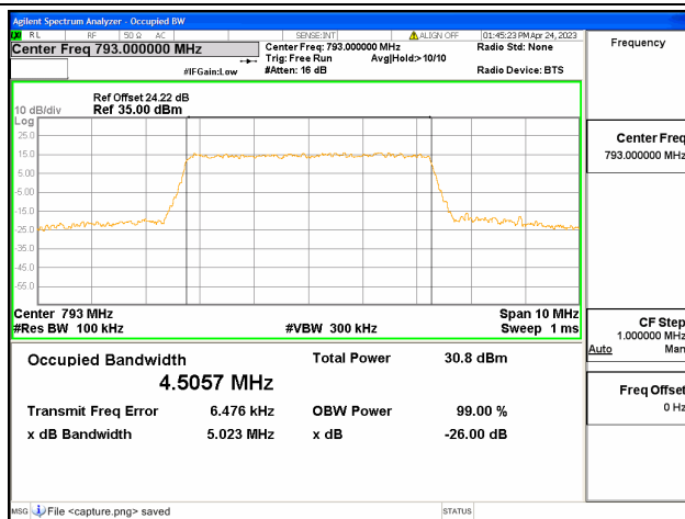
Band14 / 5MHz / 16QAM/ Mid CH
