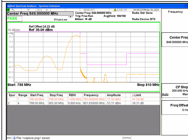
Band14 / 10MHz / High CH / QPSK / 1 RB
