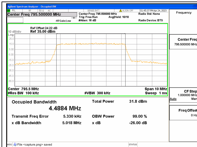
Band14 / 5MHz / QPSK/ High CH
