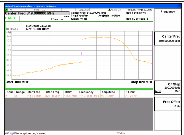
Band26 Part90 / 3MHz / Low CH / QPSK / FULL RB
