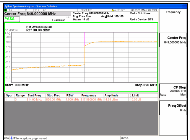
Band26 Part90 / 10MHz / Low CH / QPSK / FULL RB
