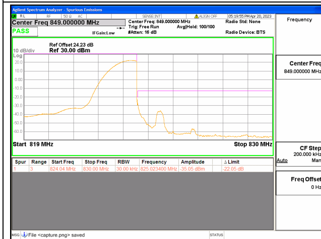
Band26 Part90 / 3MHz / High CH / QPSK / 1 RB
