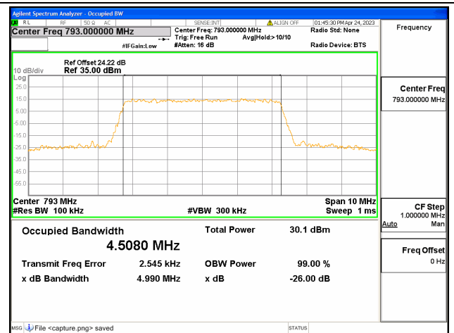
Band14 / 5MHz / 64QAM/ Mid CH
