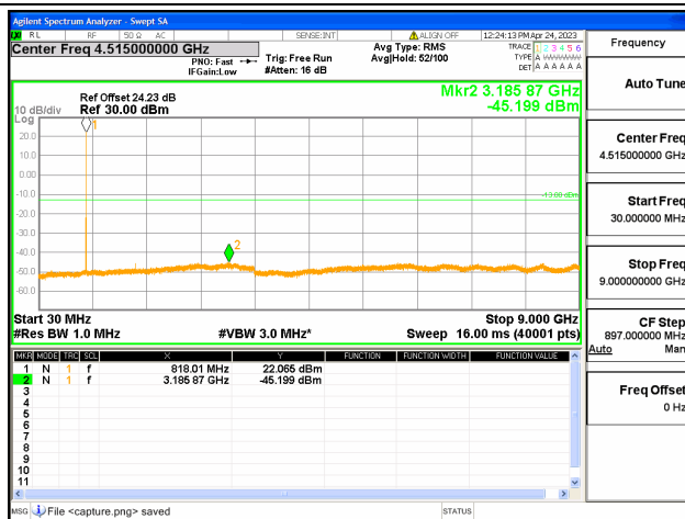
Band26 Part90 / 3MHz / Mid CH / QPSK
