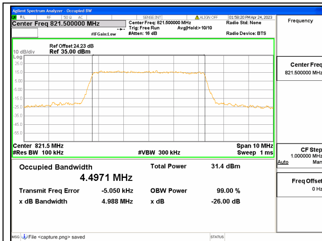
Band26 Part90 / 5MHz / QPSK/ High CH
