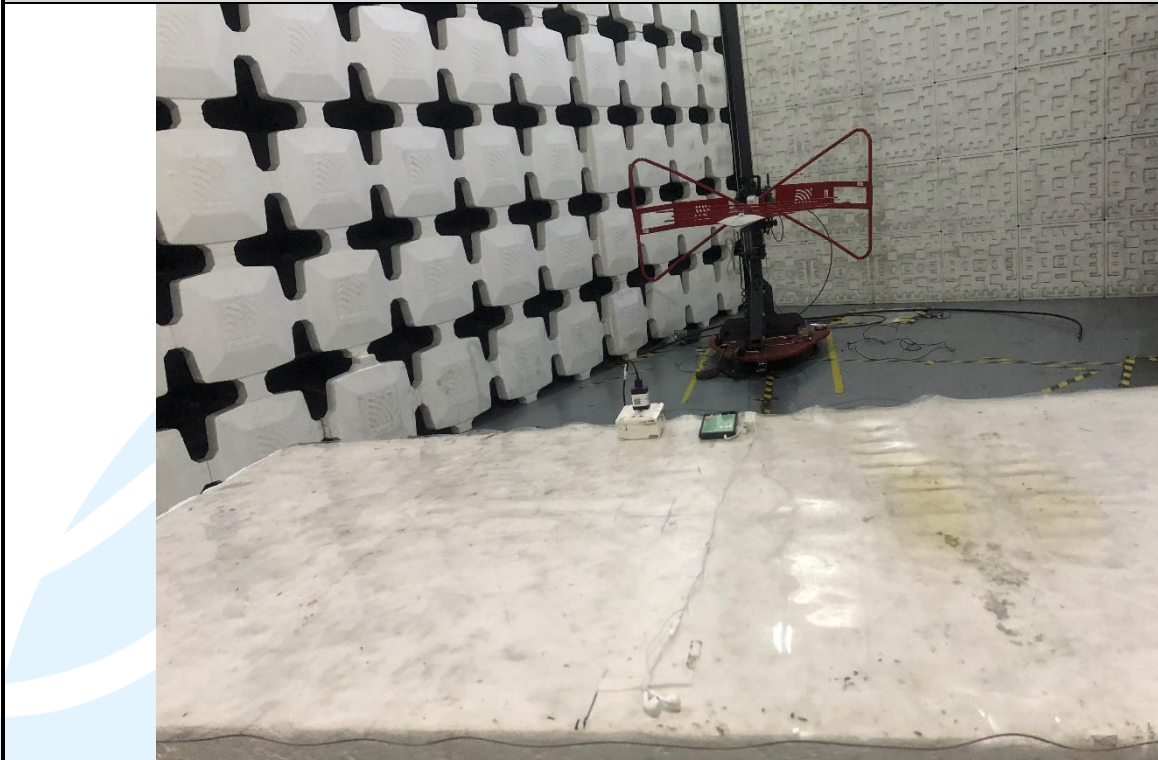
Radiated emission Test Setup-1 (30 MHz~1 GHz) – Test Mode 4/5
