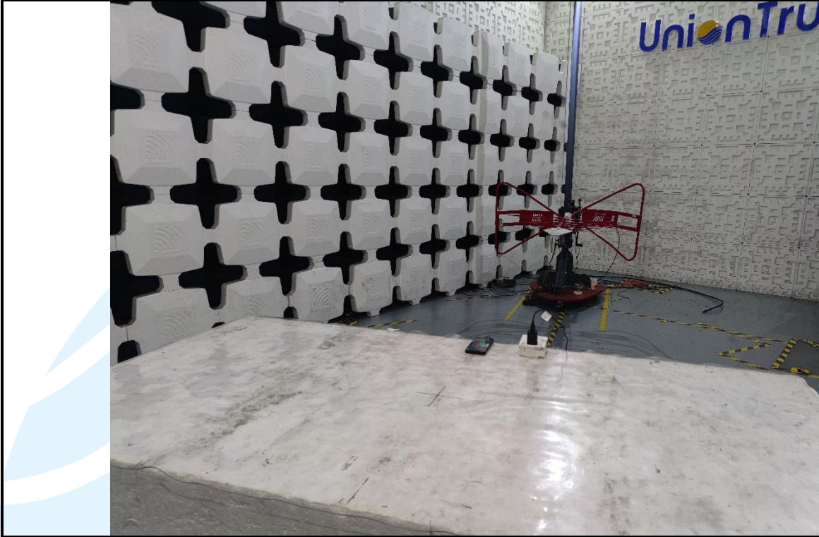
Radiated emission Test Setup-1 (30 MHz~1 GHz) – Test Mode 4 (Test Mode 1)
