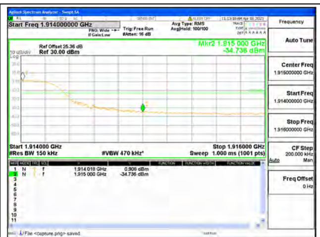
Band25 / 15MHz / High CH / QPSK / FULL RB
