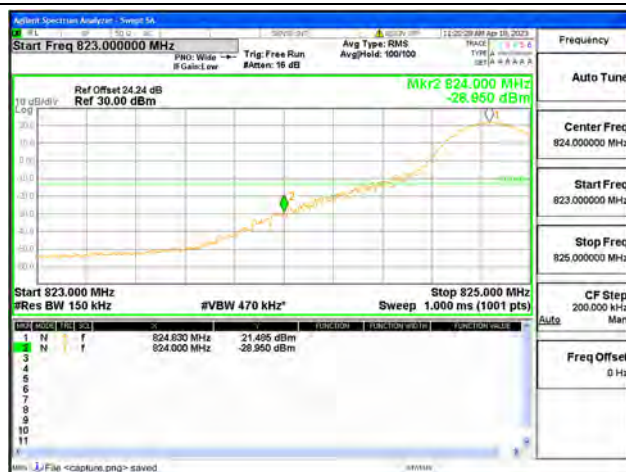
Band26 Part22 / 15MHz / Low CH / QPSK / 1 RB
