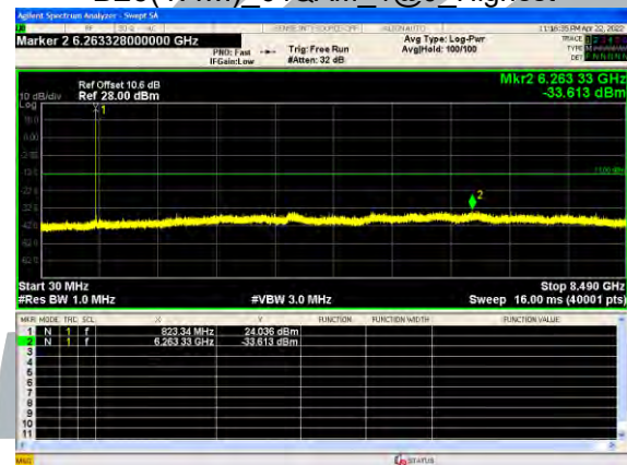
B26(1.4M)_64QAM 1@0_Highest
