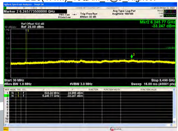
B26(1.4M)_16QAM 1@0_Highest
