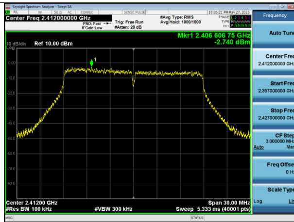
Tx. Spurious NVNT n20 2412MHz Ant1 Ref
