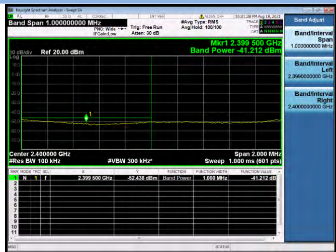
802.11b L Channel 1, Reference level
