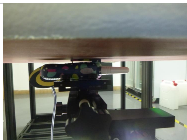
Body-worn(0mm)-Li
