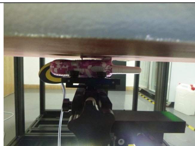
Body-worn(0mm) -4*AAA
