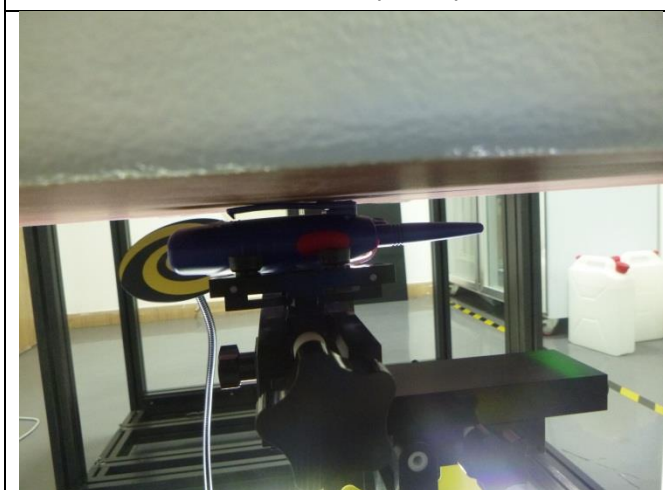
Body-worn(0mm)
