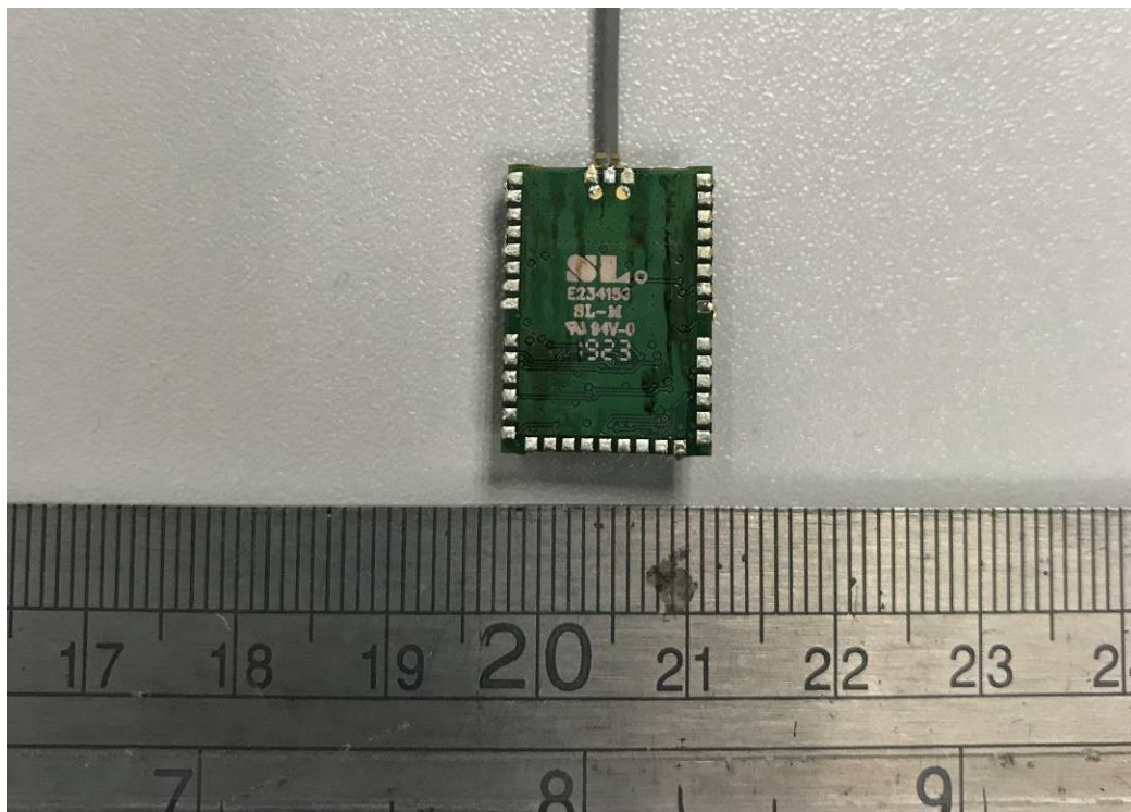
Internal View
