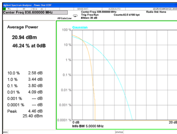
HSPA5_Middle_
