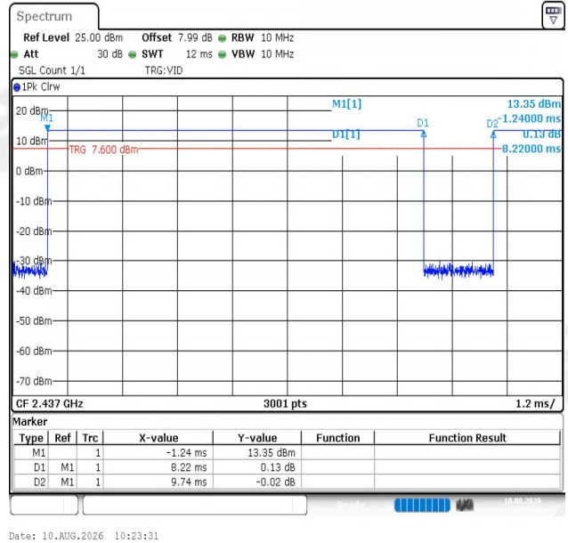
NTNV-11B-Ant1-2437
