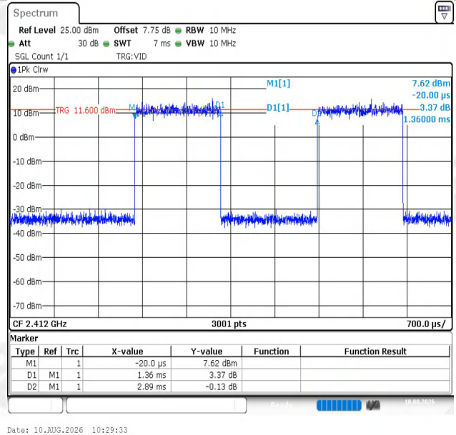
NTNV-11G-Ant1-2412
