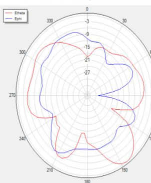
V Phi=0 freq=2400MHz
