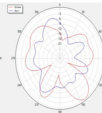
V Phi=0 freq=2430MHz
