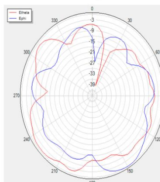
V Phi=90 freq=2410MHz
