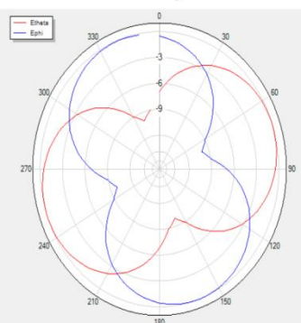
H Theta=0 freq=2430MHz
