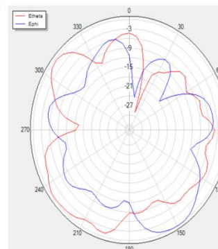
V Phi=90 freq=2420MHz
