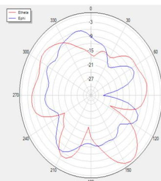
V Phi=0 freq=2410MHz
