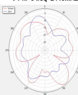
V Phi=0 freq=2440MHz
