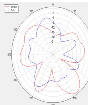
V Phi=0 freq=2420MHz
