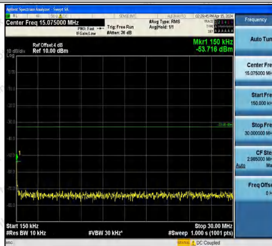
Band4-1312-4-0.15~30MHz-PASS
