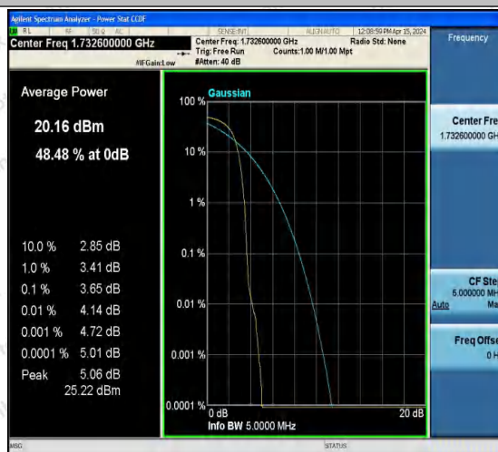
Band4-1413-3-PASS
