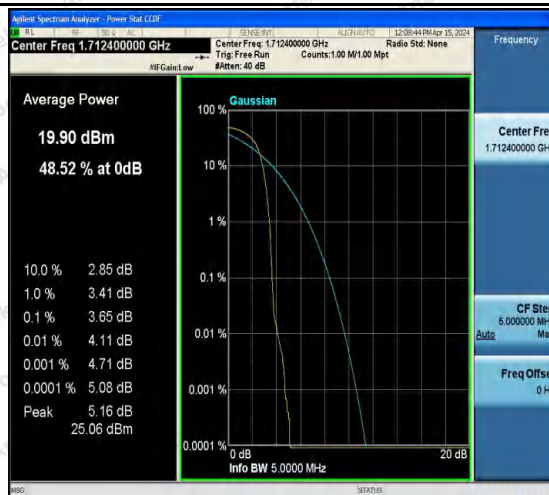
Band4-1312-3-PASS
