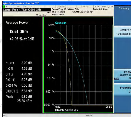
Band4-1312-4-PASS
