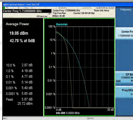
Band4-1413-4-PASS
