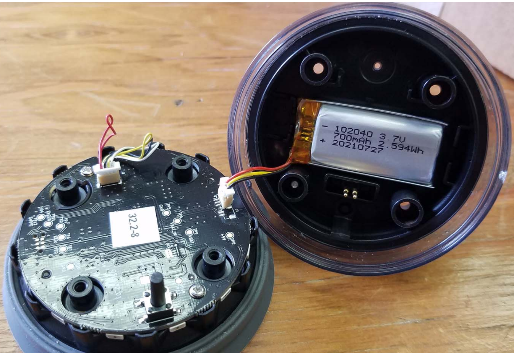
Inside View of the EUT - View #1
