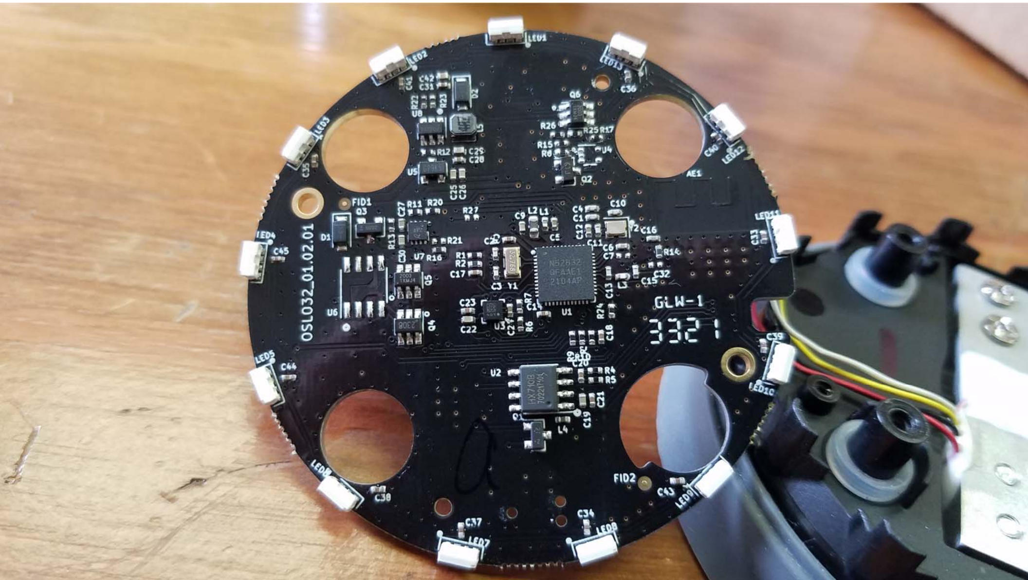
Bottom View of the PCB for the EUT - View #1
