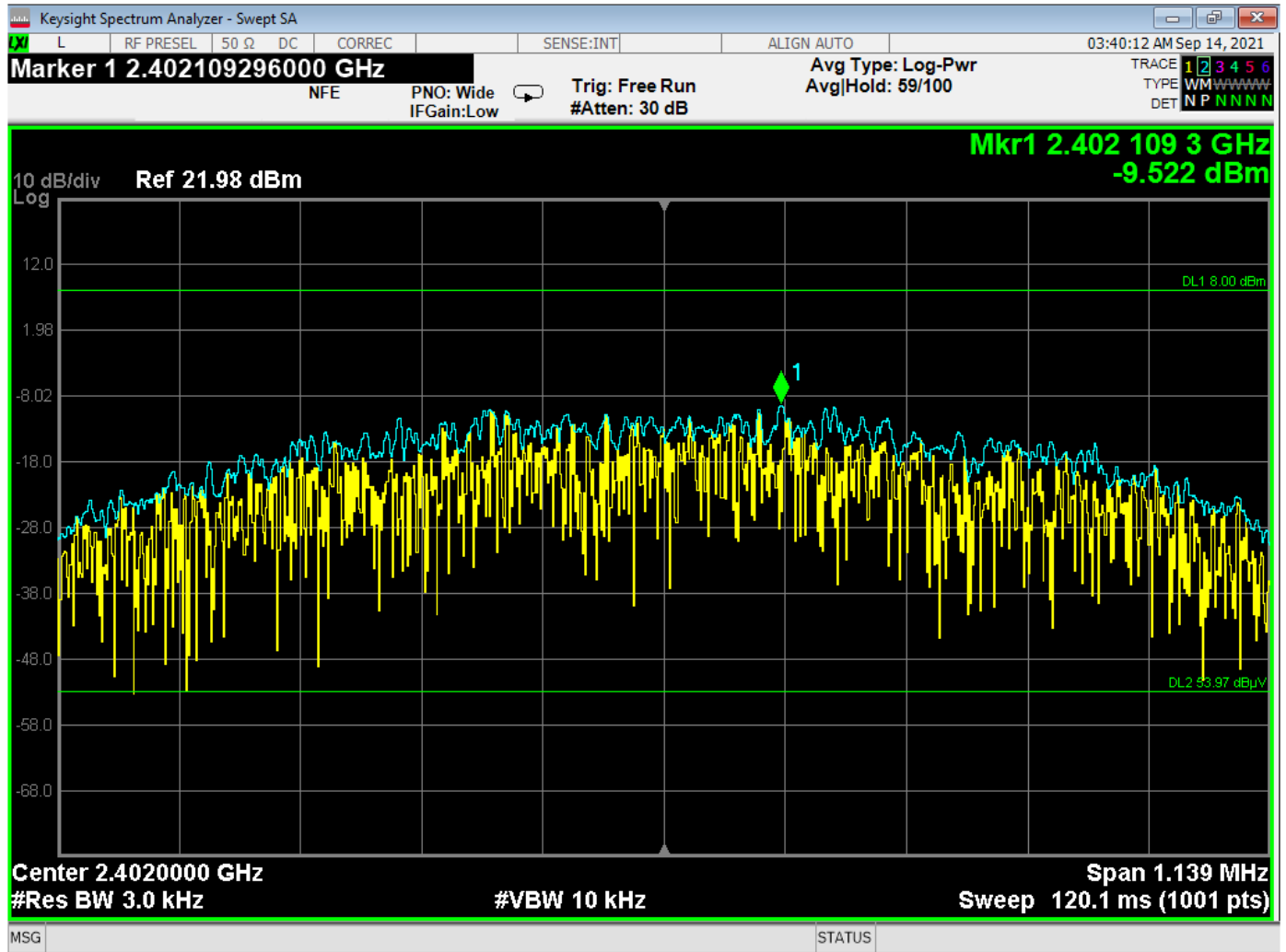
Peak Power Spectral Density – Low Channel
