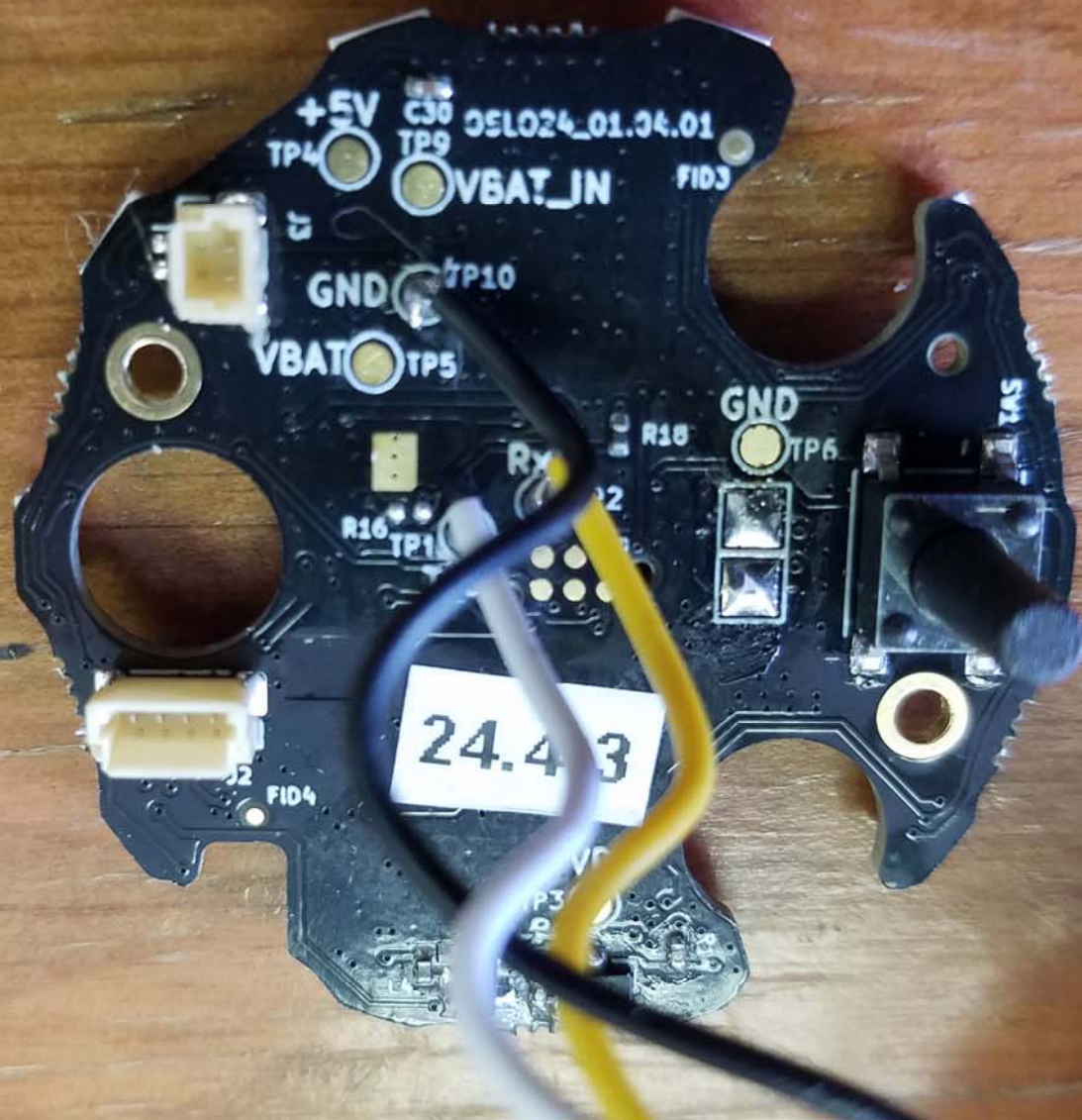
Top View of the PCB for the EUT - View #1
