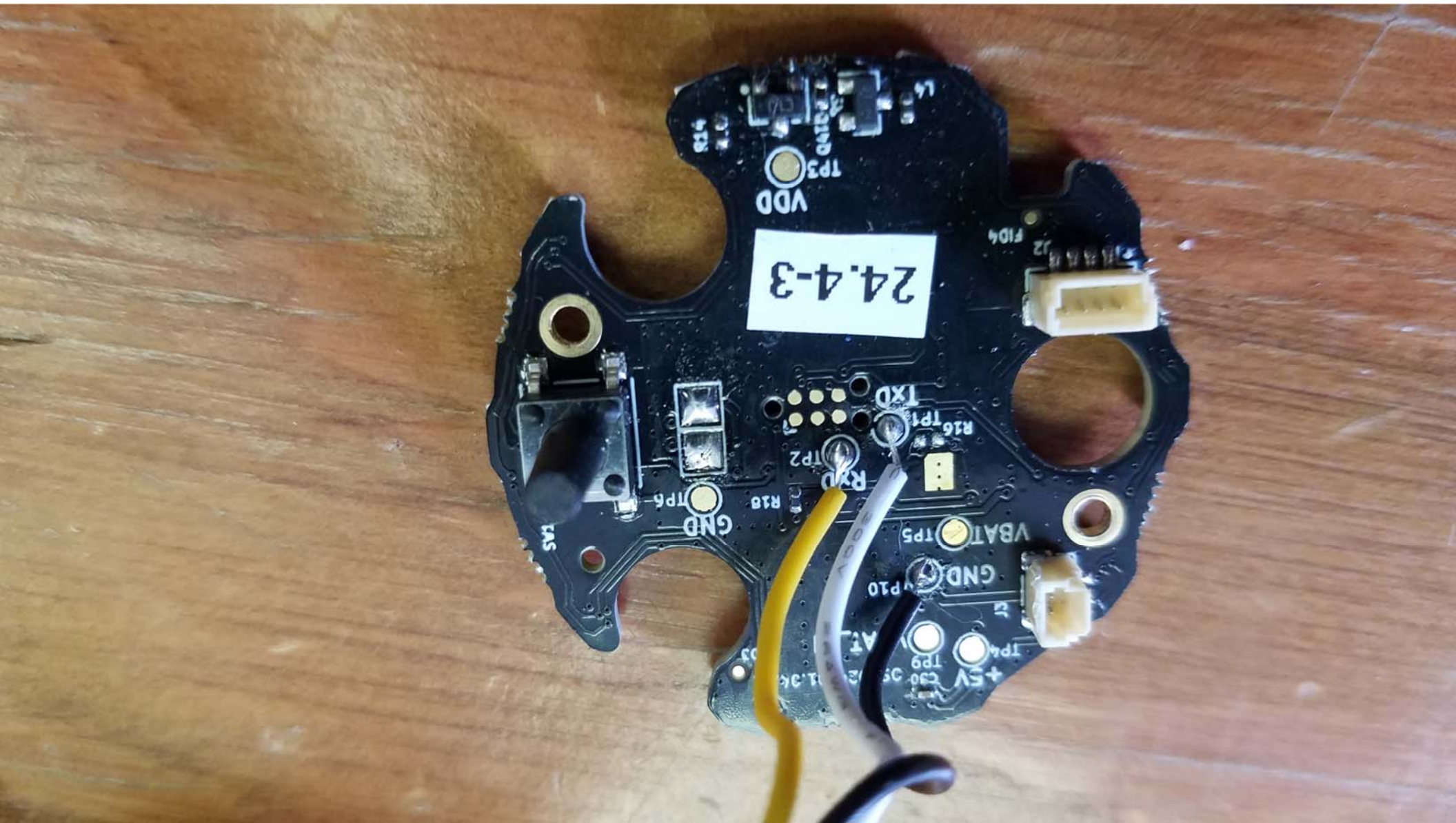
Top View of the PCB for the EUT - View #4
