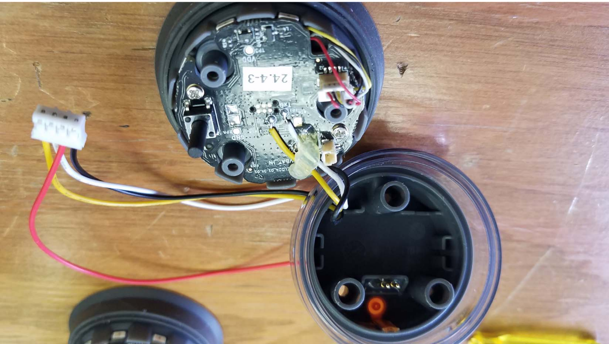
Inside View #2 of the EUT
