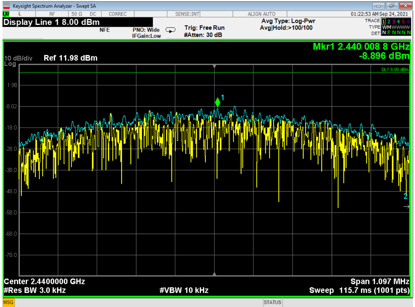
Peak Power Spectral Density – Middle Channel
