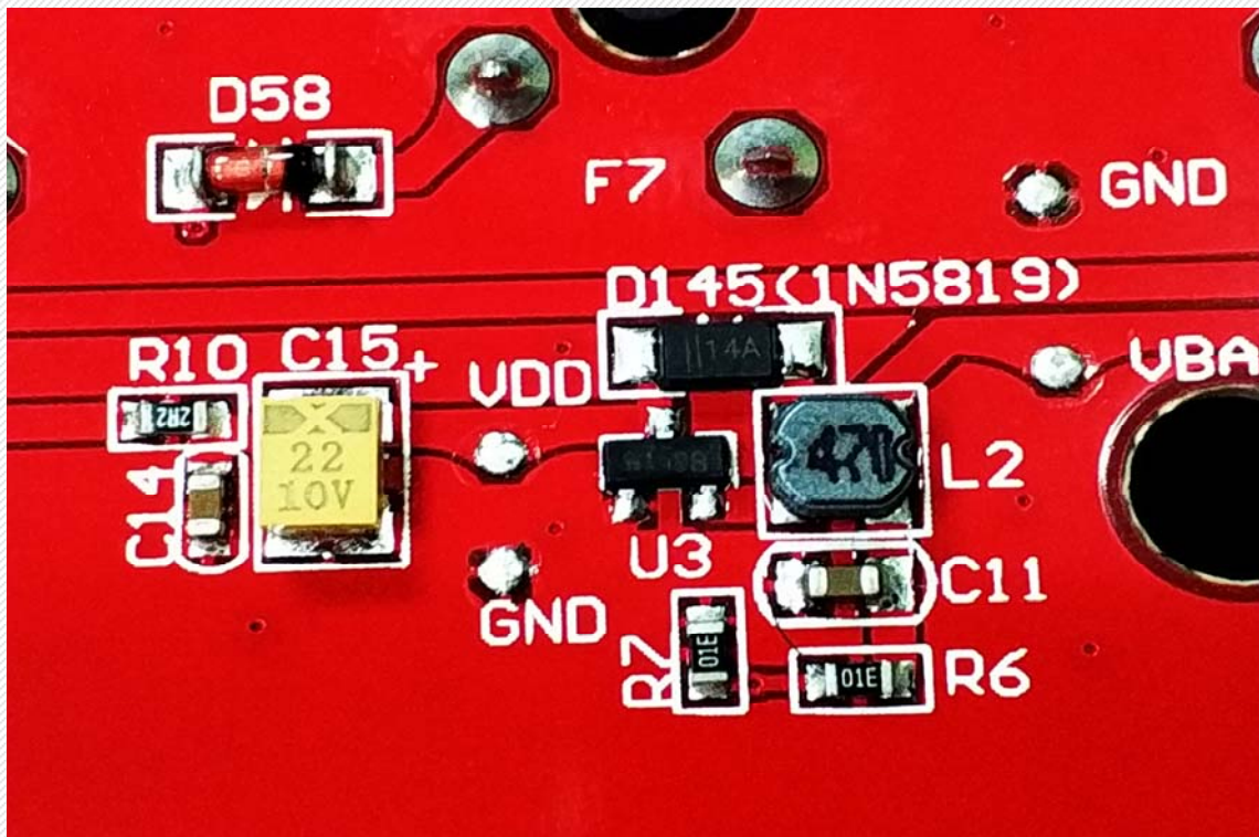
< PCB Close in view of W200 >
