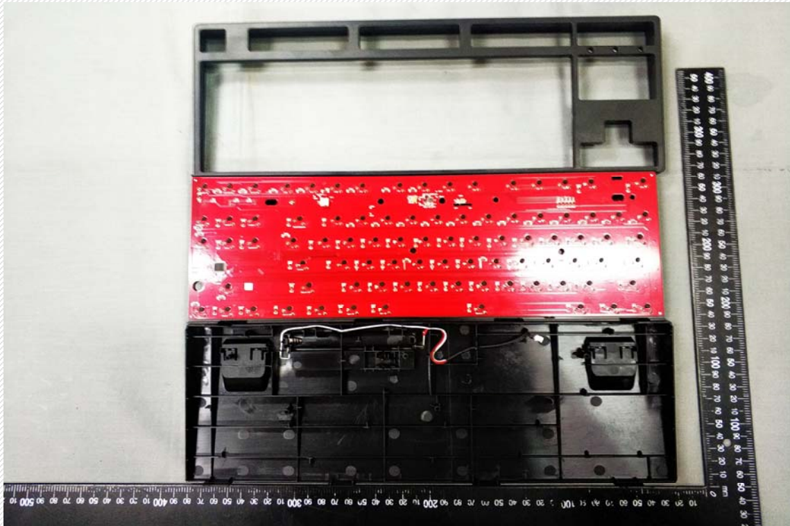
< PCB-F view of W200 >
