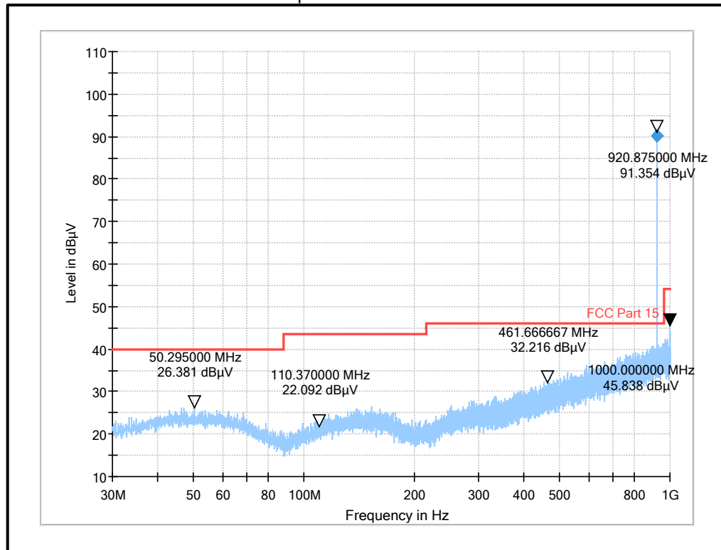
Radiated Transmitter spurious emission from 30 MHz – 1 GHz
