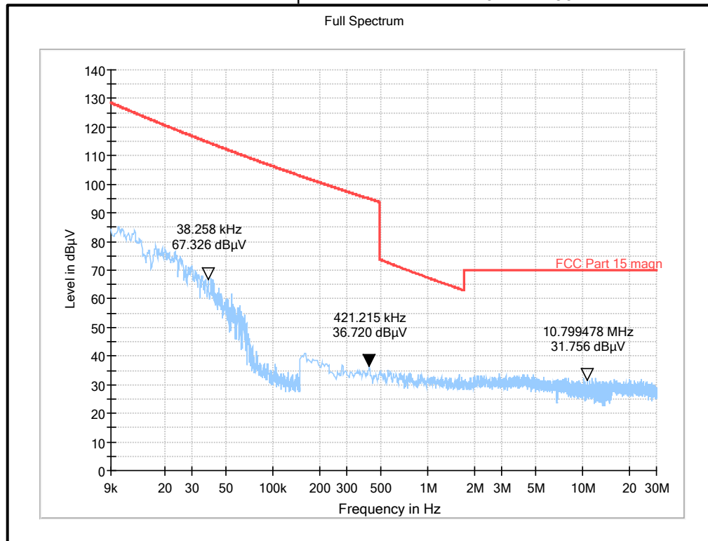
Radiated Transmitter spurious emission from 9 kHz – 30 MHz
