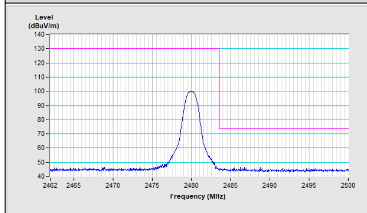
BT GFSK Channel 78
