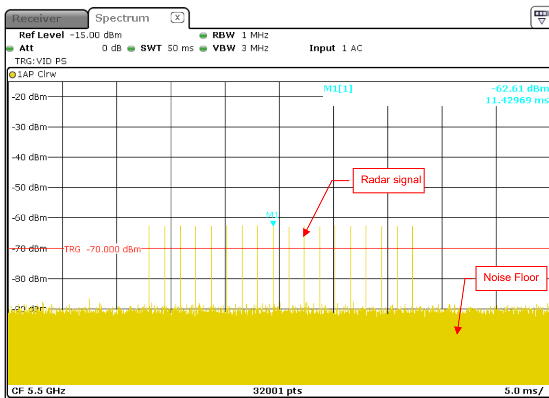
Radar Signal 0
