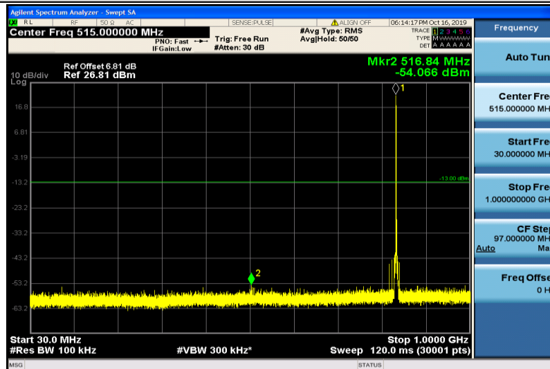
Band5-1.4MHz-QPSK-20525-1RB#0-30~1000MHz
