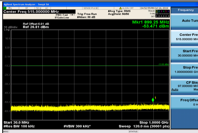
Band4-3MHz-QPSK-20175-1RB#0-30~1000MHz
