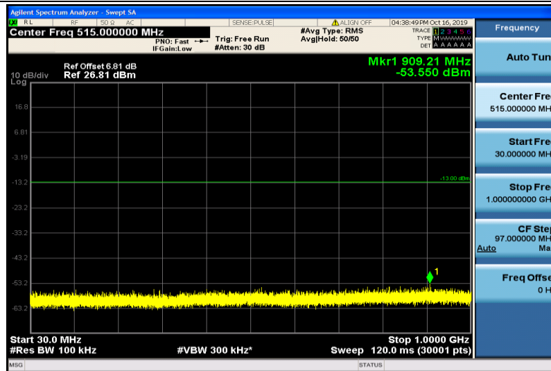
Band4-1.4MHz-QPSK-19957-1RB#0-30~1000MHz
