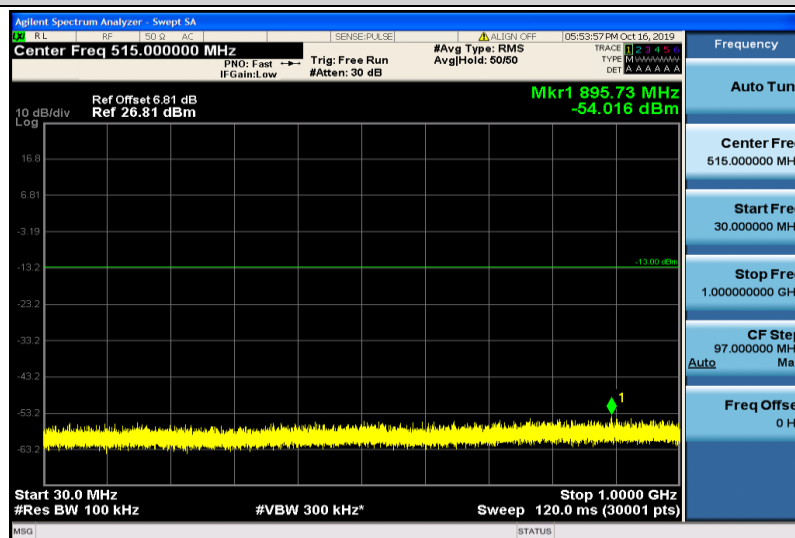
Band4-15MHz-QPSK-20325-1RB#0-30~1000MHz
