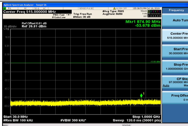
Band4-5MHz-QPSK-20175-1RB#0-30~1000MHz
