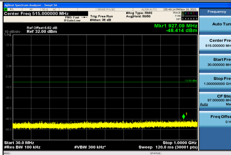
Band2-15MHz-16QAM-18900-1RB#0-30~1000MHz
