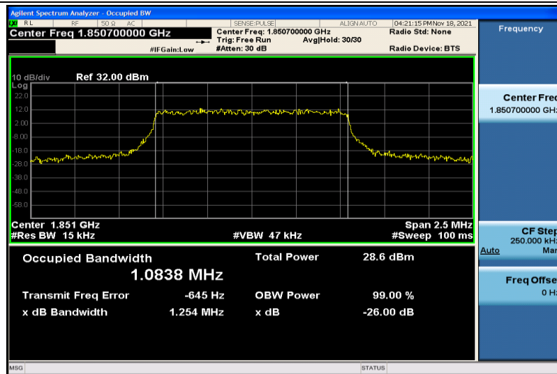
Band2-1.4MHz-QPSK-18607-6RB#0-1.0838
