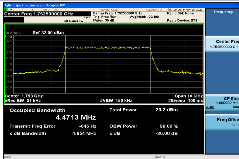
Band4-5MHz-QPSK-20375-25RB#0-4.4713
