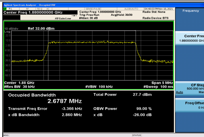
Band2-3MHz-16QAM-18900-15RB#0-2.6787
