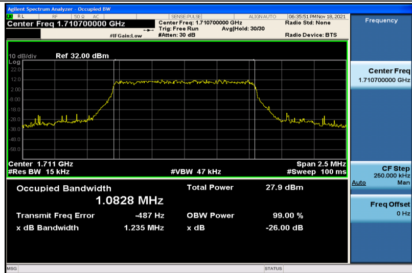
Band4-1.4MHz-QPSK-19957-6RB#0-1.0828
