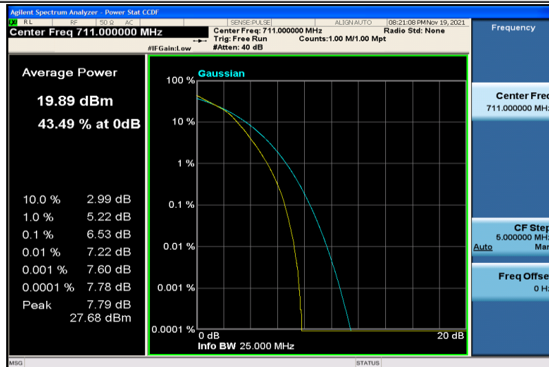
Band17-10MHz-16QAM-23800-50RB#0
