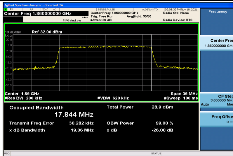
Band2-20MHz-16QAM-18700-100RB#0-17.844
