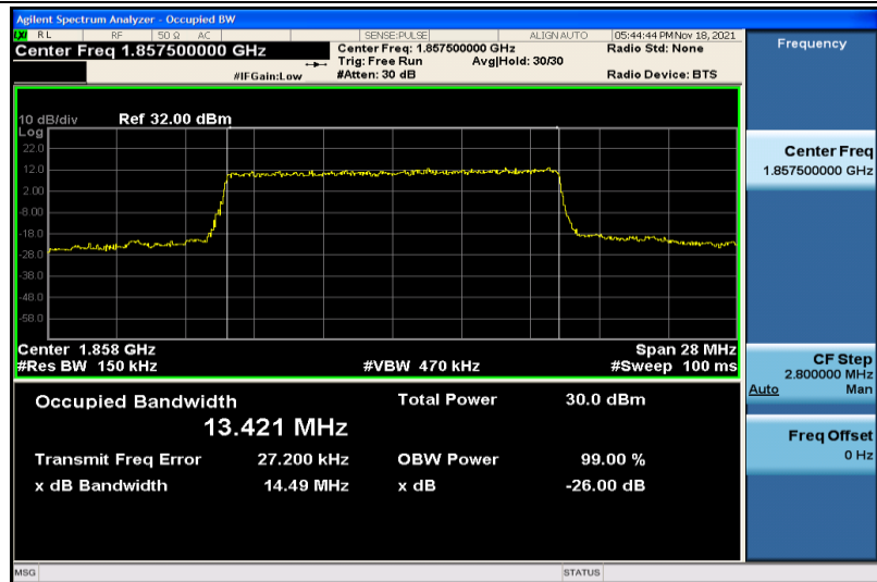
Band2-15MHz-QPSK-18675-75RB#0-13.421
