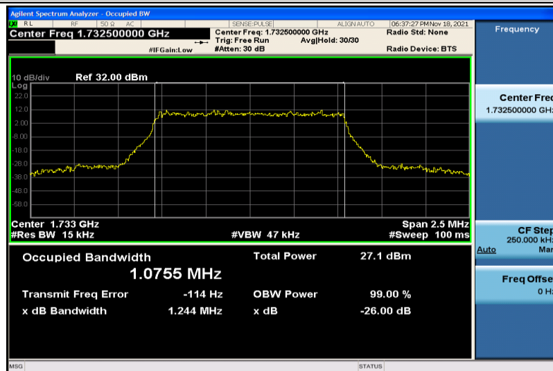
Band4-1.4MHz-16QAM-20175-6RB#0-1.0755
