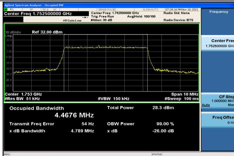
Band4-5MHz-16QAM-20375-25RB#0-4.4676
