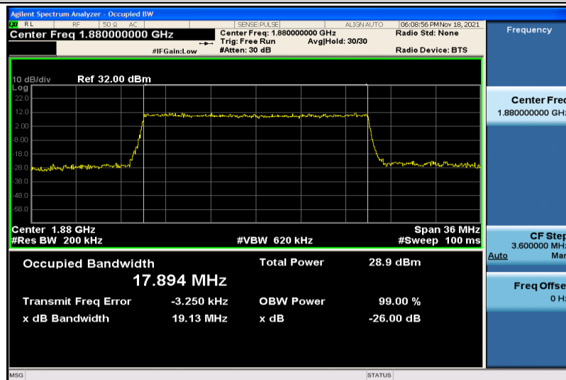
Band2-20MHz-16QAM-18900-100RB#0-17.894
