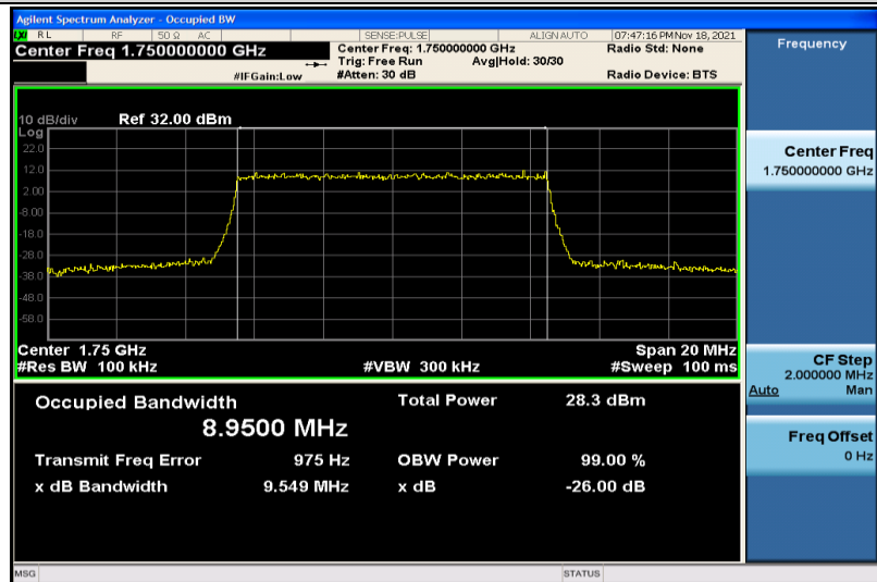
Band4-10MHz-16QAM-20350-50RB#0-8.9500
