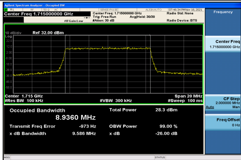
Band4-10MHz-16QAM-20000-50RB#0-8.9360
