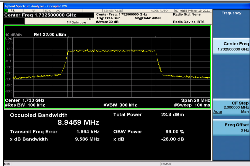
Band4-10MHz-16QAM-20175-50RB#0-8.9459
