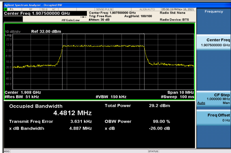
Band2-5MHz-QPSK-19175-25RB#0-4.4812
