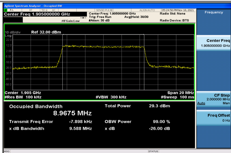
Band2-10MHz-QPSK-19150-50RB#0-8.9675
