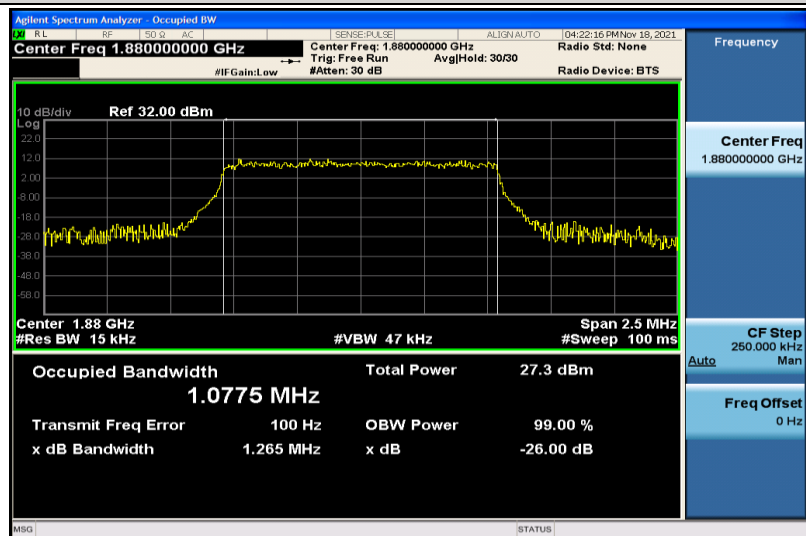
Band2-1.4MHz-16QAM-18900-6RB#0-1.0775
