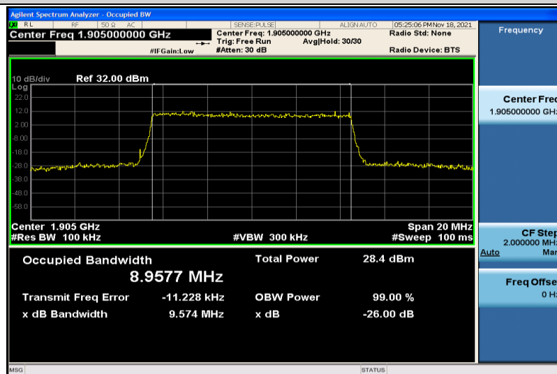
Band2-10MHz-16QAM-19150-50RB#0-8.9577
