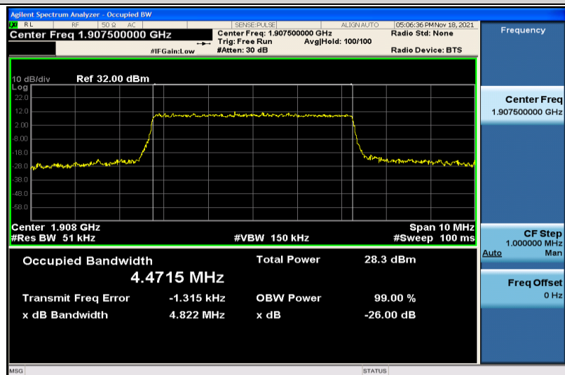
Band2-5MHz-16QAM-19175-25RB#0-4.4715
