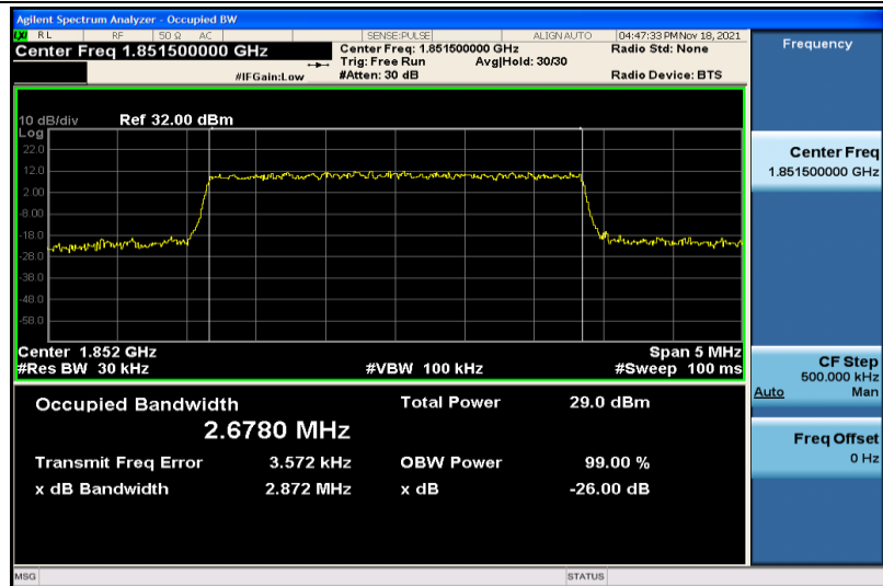
Band2-3MHz-QPSK-18615-15RB#0-2.6780
