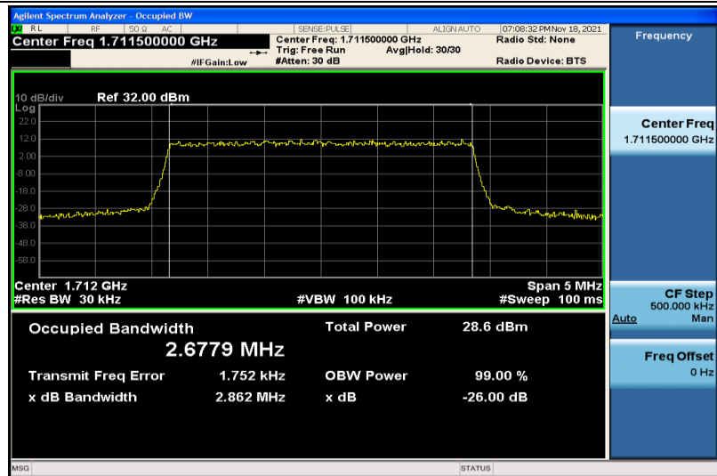
Band4-3MHz-QPSK-19965-15RB#0-2.6779
