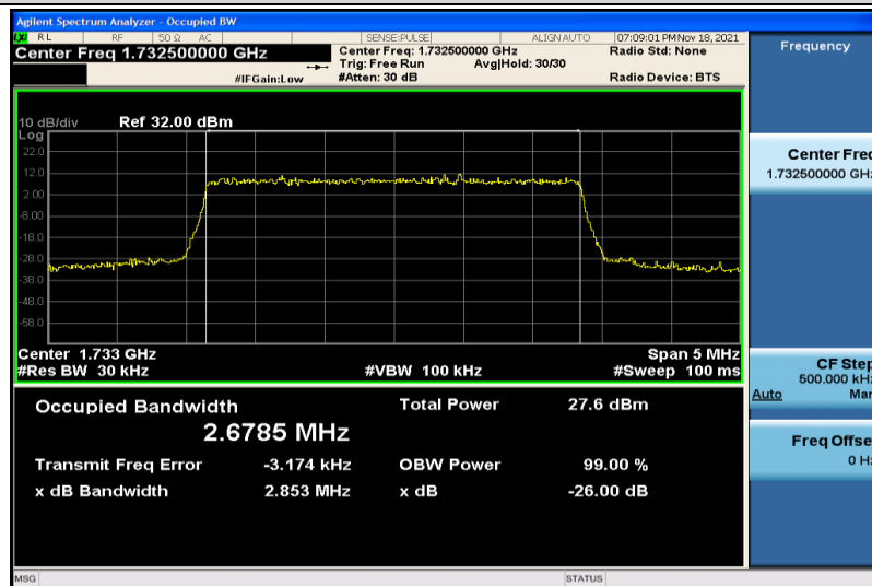
Band4-3MHz-16QAM-20175-15RB#0-2.6785
