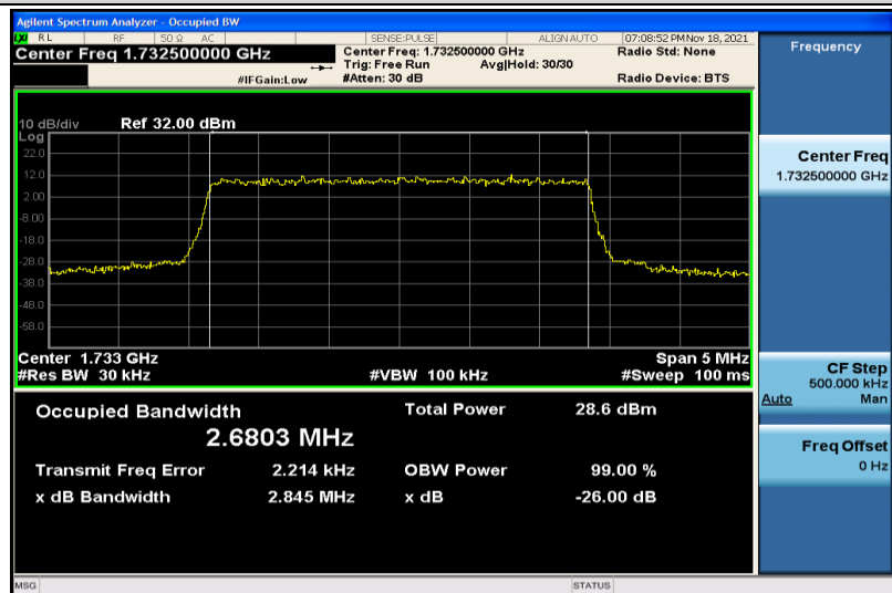
Band4-3MHz-QPSK-20175-15RB#0-2.6803
