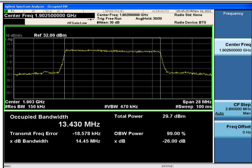
Band2-15MHz-QPSK-19125-75RB#0-13.430
