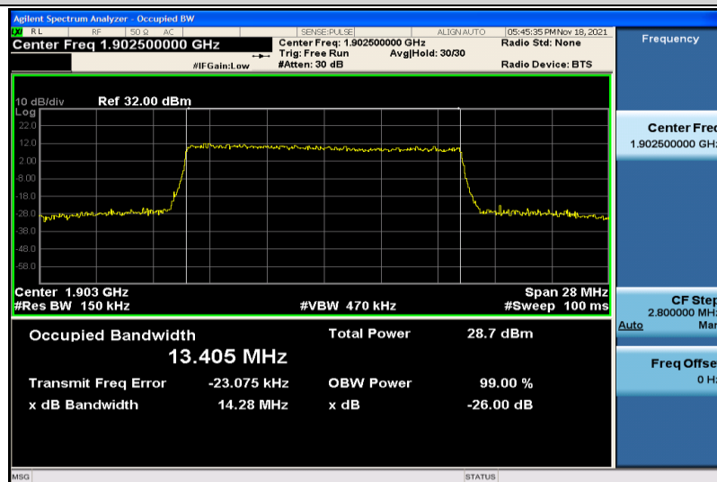
Band2-15MHz-16QAM-19125-75RB#0-13.405
