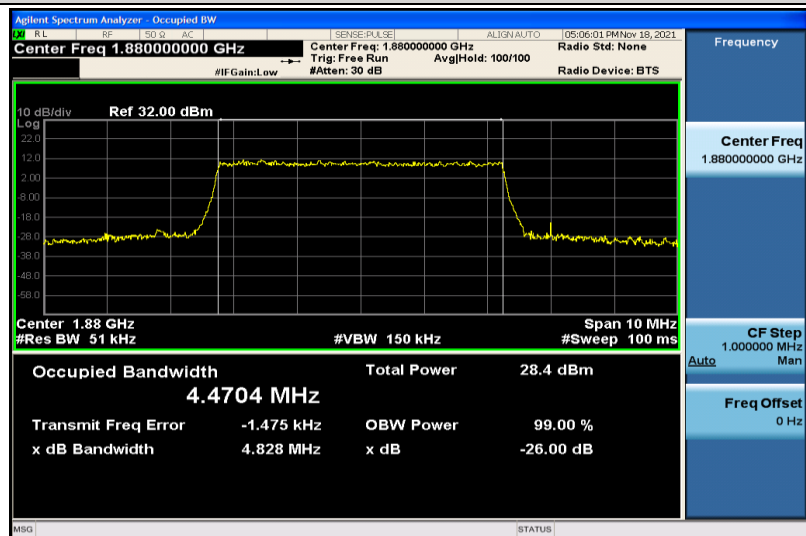
Band2-5MHz-16QAM-18900-25RB#0-4.4704
