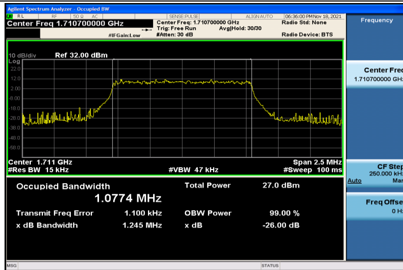
Band4-1.4MHz-16QAM-19957-6RB#0-1.0774
