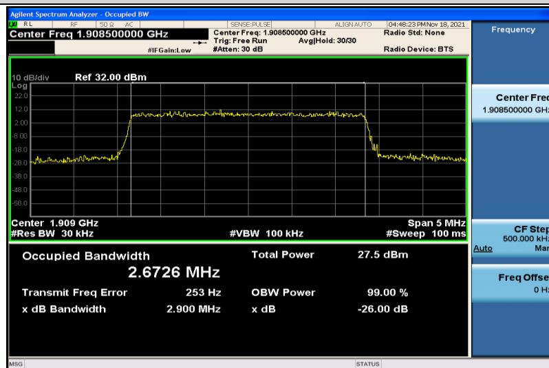
Band2-3MHz-16QAM-19185-15RB#0-2.6726
