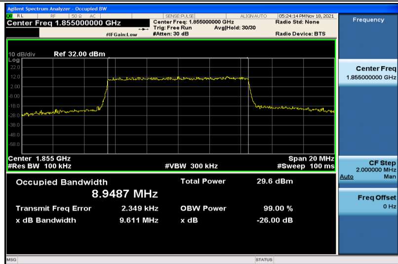
Band2-10MHz-QPSK-18650-50RB#0-8.9487
