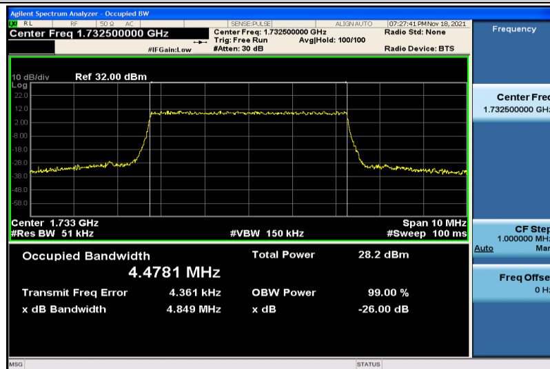
Band4-5MHz-16QAM-20175-25RB#0-4.4781
