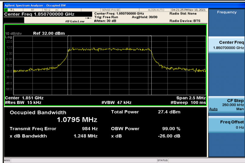
Band2-1.4MHz-16QAM-18607-6RB#0-1.0795
