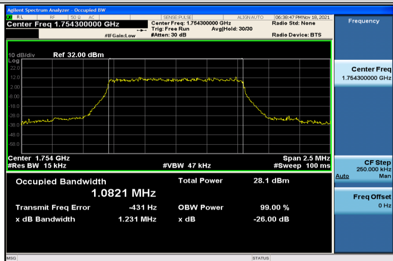
Band4-1.4MHz-QPSK-20393-6RB#0-1.0821
