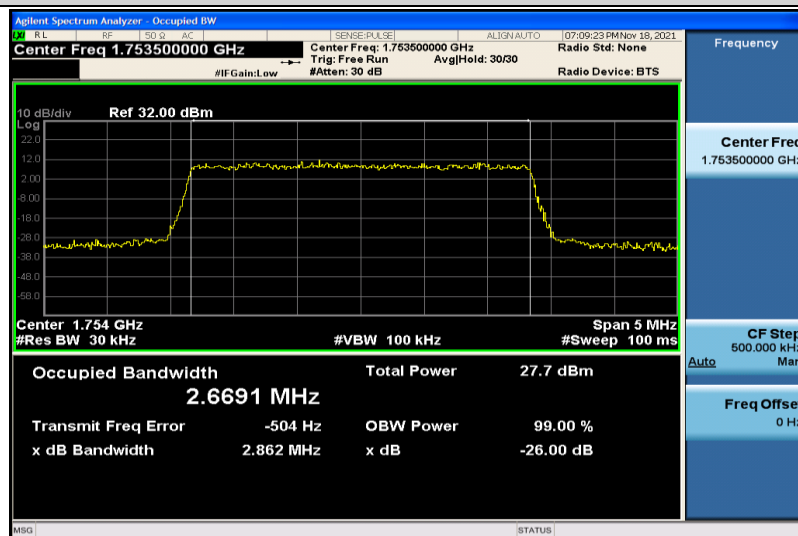
Band4-3MHz-16QAM-20385-15RB#0-2.6691
