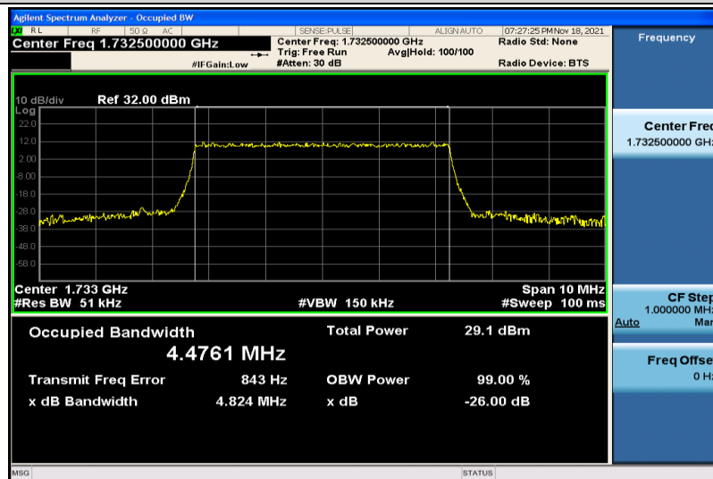
Band4-5MHz-QPSK-20175-25RB#0-4.4761
