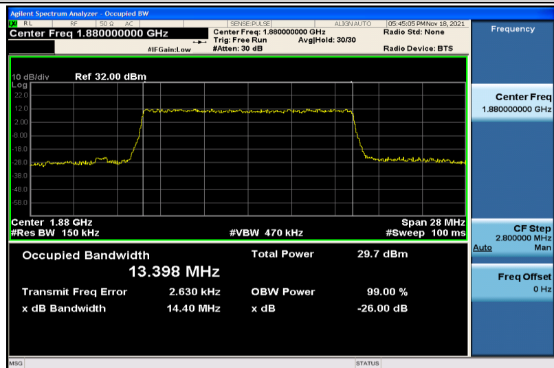
Band2-15MHz-QPSK-18900-75RB#0-13.398
