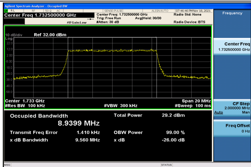
Band4-10MHz-QPSK-20175-50RB#0-8.9399
