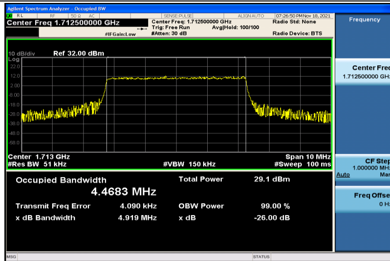
Band4-5MHz-QPSK-19975-25RB#0-4.4683
