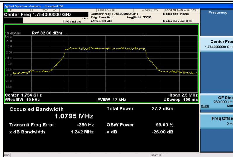
Band4-1.4MHz-16QAM-20393-6RB#0-1.0795
