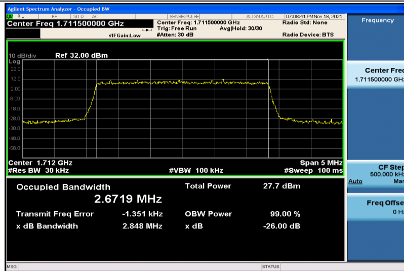
Band4-3MHz-16QAM-19965-15RB#0-2.6719
