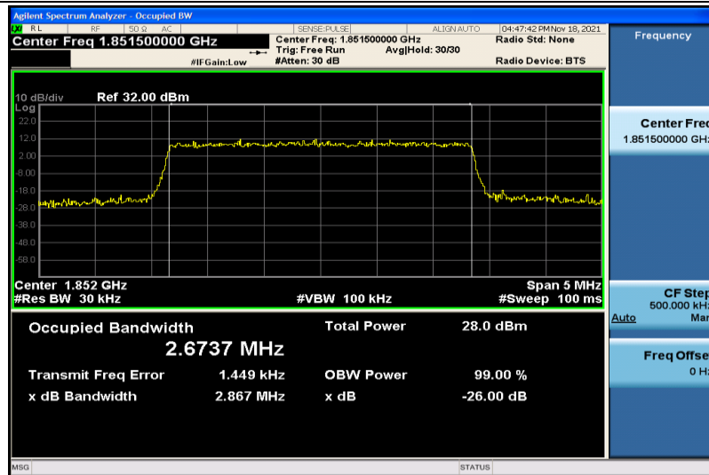
Band2-3MHz-16QAM-18615-15RB#0-2.6737
