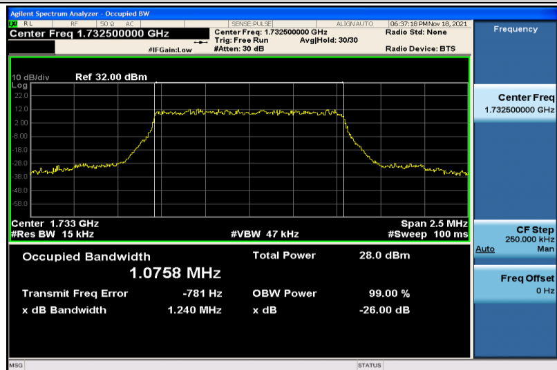
Band4-1.4MHz-QPSK-20175-6RB#0-1.0758
