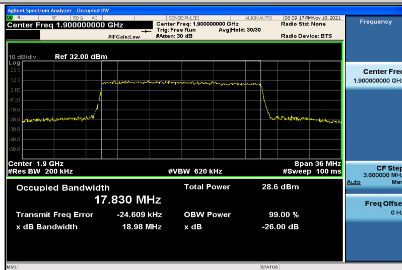
Band2-20MHz-16QAM-19100-100RB#0-17.830
