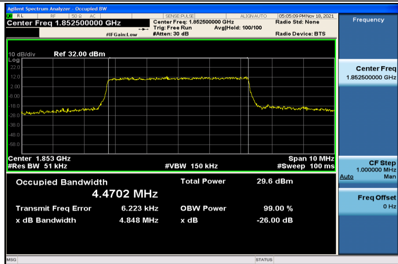
Band2-5MHz-QPSK-18625-25RB#0-4.4702
