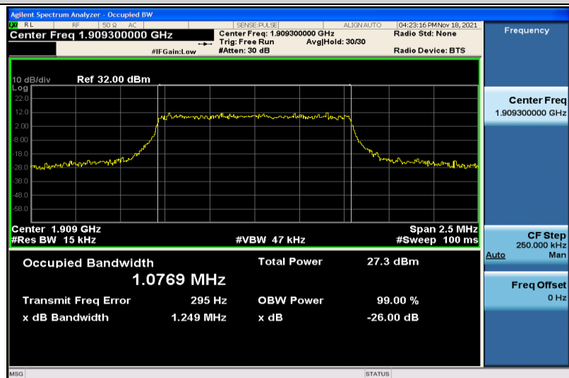
Band2-1.4MHz-16QAM-19193-6RB#0-1.0769
