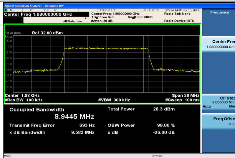
Band2-10MHz-16QAM-18900-50RB#0-8.9445
