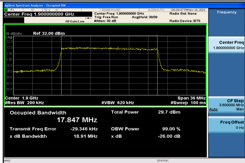
Band2-20MHz-QPSK-19100-100RB#0-17.847
