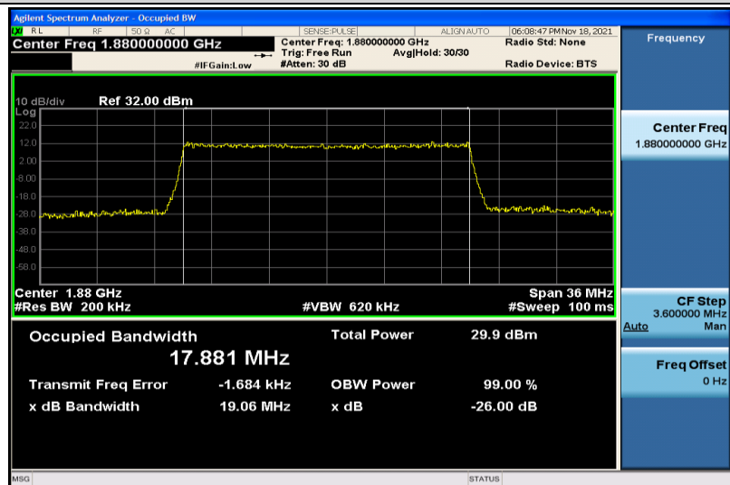
Band2-20MHz-QPSK-18900-100RB#0-17.881
