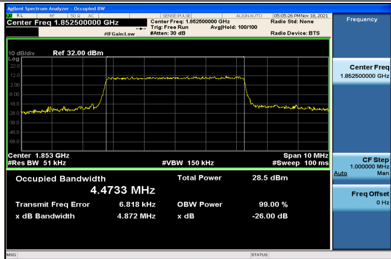
Band2-5MHz-16QAM-18625-25RB#0-4.4733
