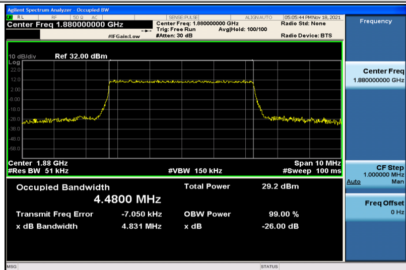
Band2-5MHz-QPSK-18900-25RB#0-4.4800
