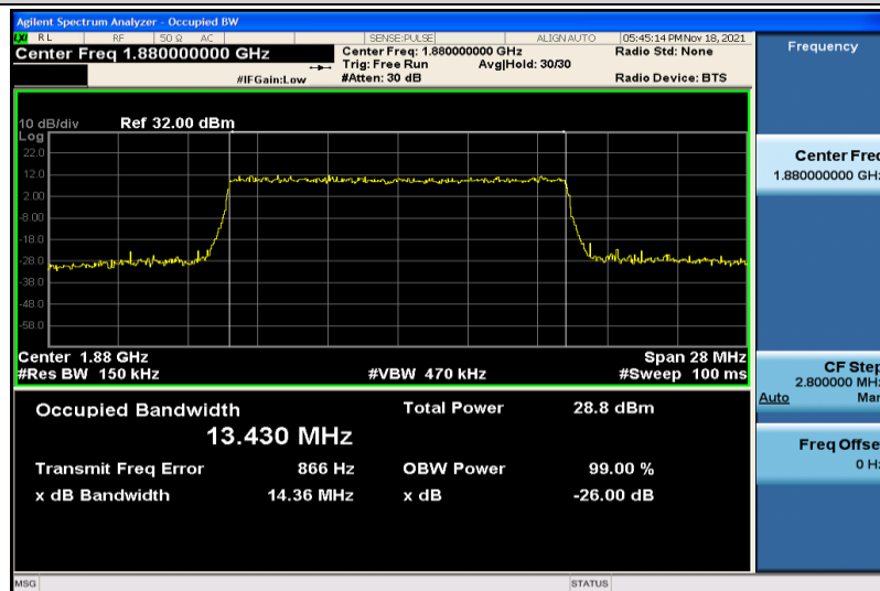
Band2-15MHz-16QAM-18900-75RB#0-13.430
