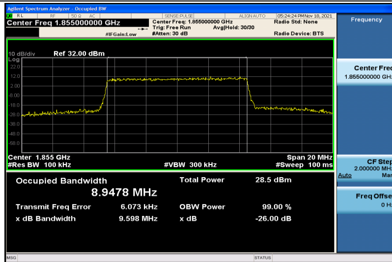
Band2-10MHz-16QAM-18650-50RB#0-8.9478
