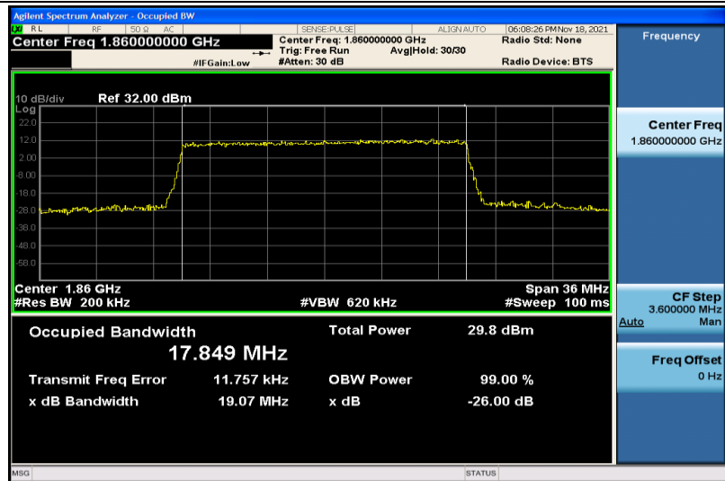
Band2-20MHz-QPSK-18700-100RB#0-17.849
