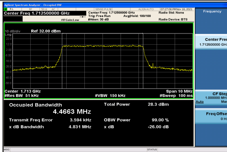
Band4-5MHz-16QAM-19975-25RB#0-4.4663
