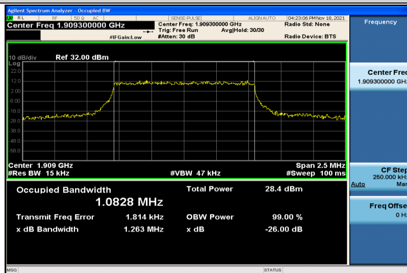
Band2-1.4MHz-QPSK-19193-6RB#0-1.0828
