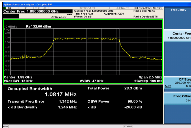
Band2-1.4MHz-QPSK-18900-6RB#0-1.0817
