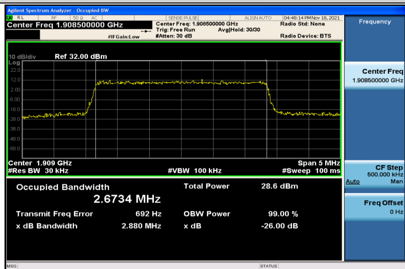
Band2-3MHz-QPSK-19185-15RB#0-2.6734
